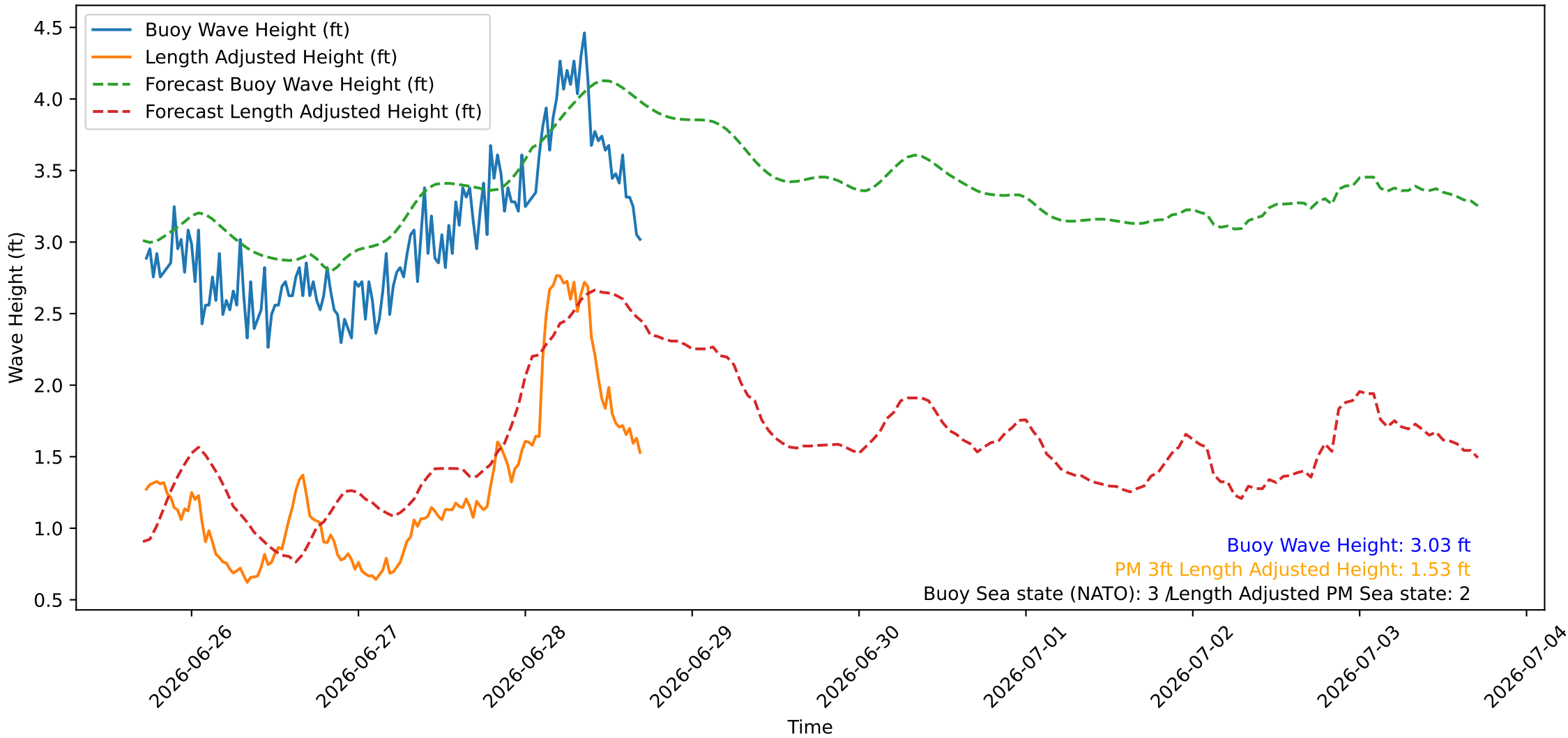
Wave Heights over Time for Red Beach at 2026-06-28 17:20:47
