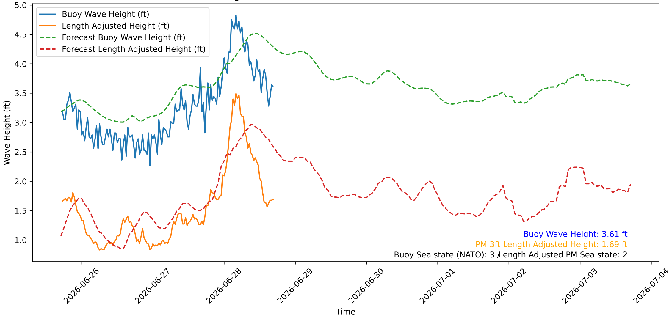
Wave Heights over Time for Green Beach at 2026-06-28 17:21:09
