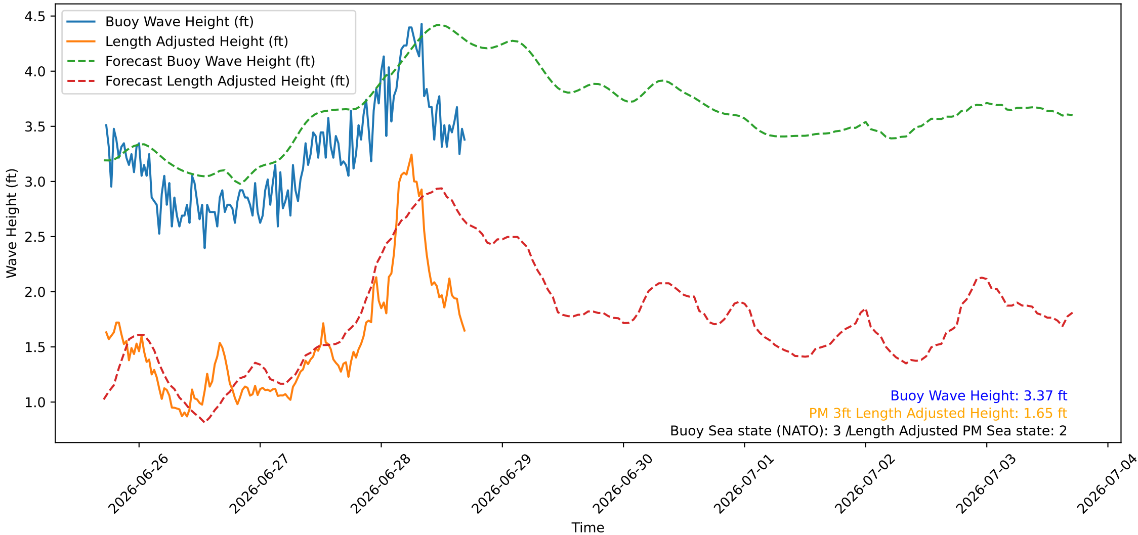
Wave Heights over Time for Oceanside Harbor at 2026-06-28 17:20:26
