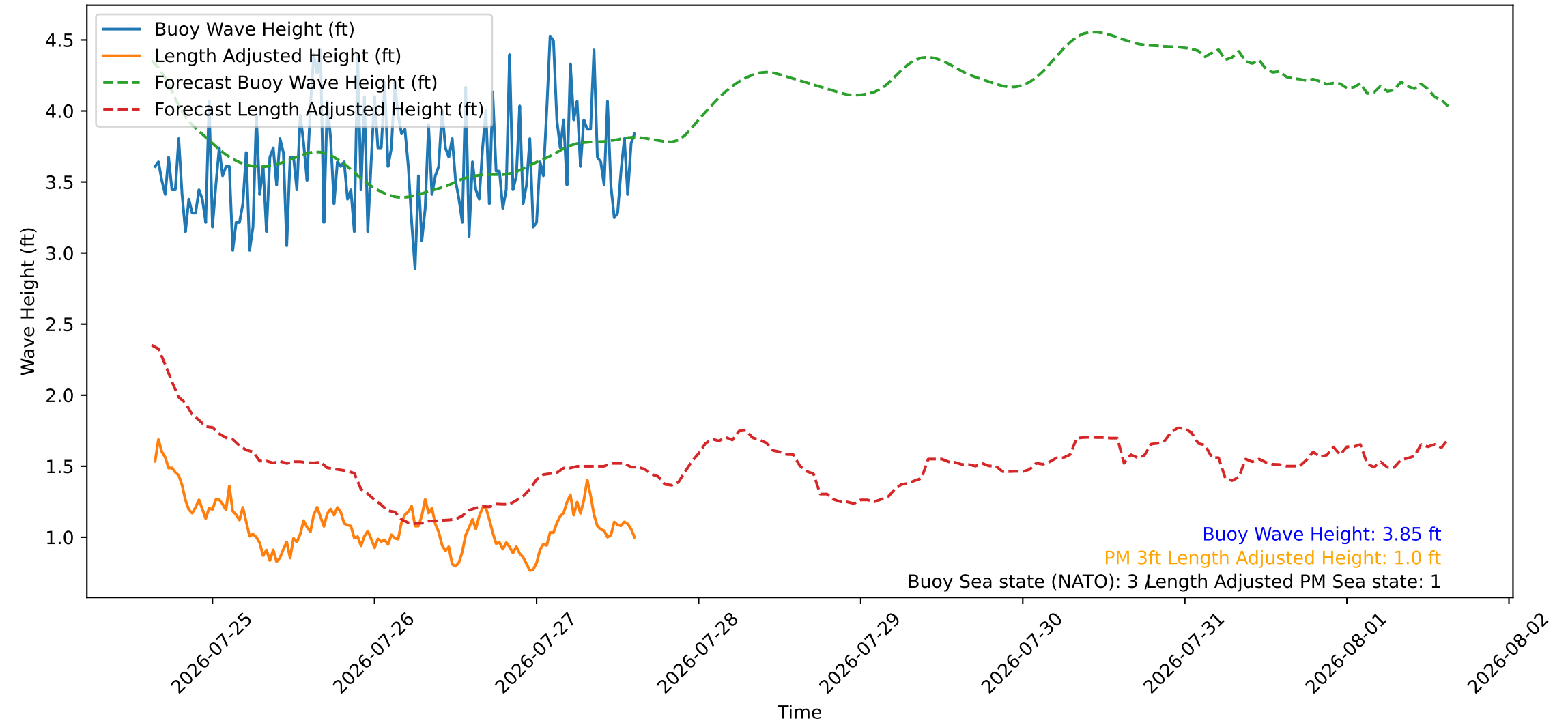
Wave Heights over Time for Red Beach at 2026-07-27 15:10:46
