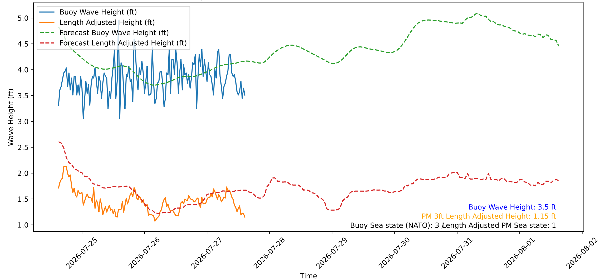
Wave Heights over Time for Oceanside Harbor at 2026-07-27 15:10:26
