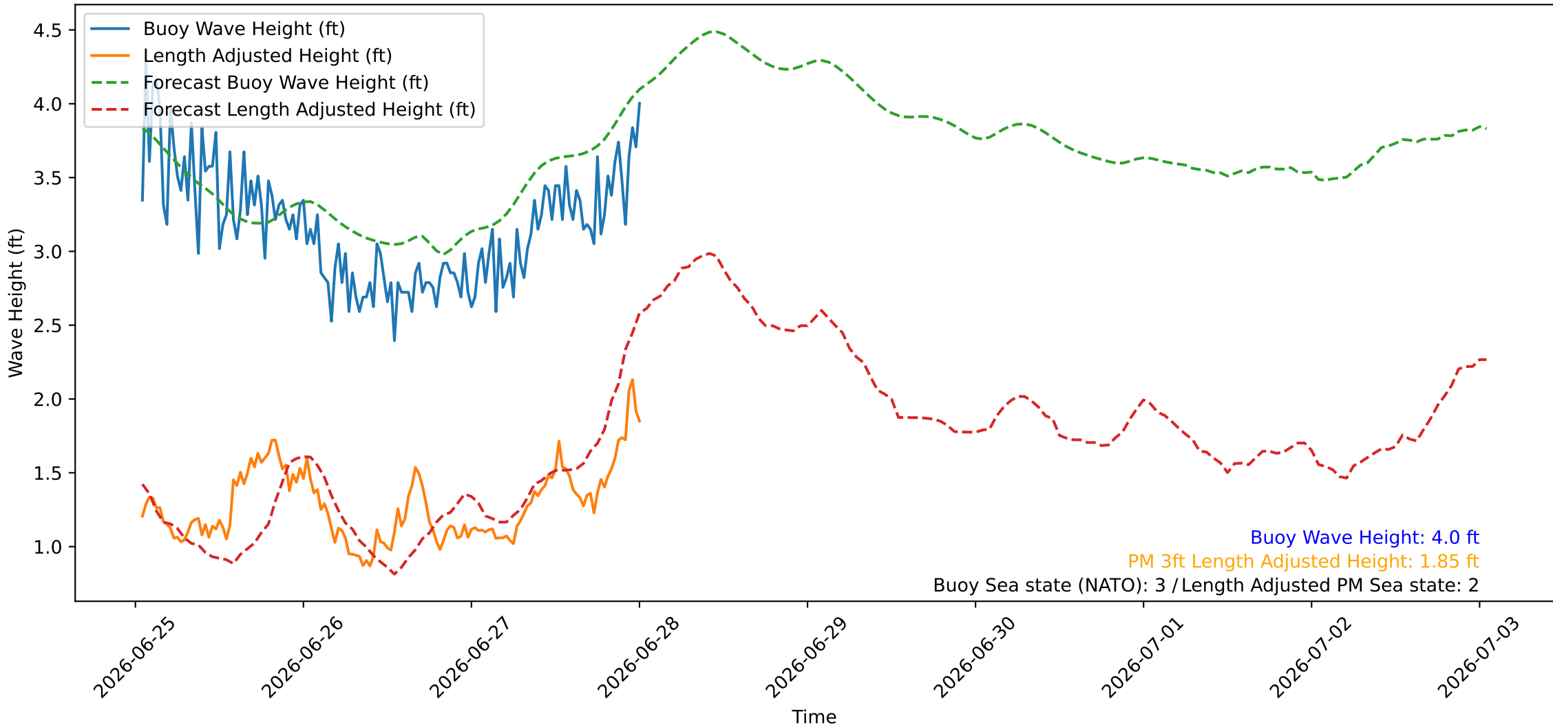
Wave Heights over Time for Oceanside Harbor at 2026-06-28 01:00:26
