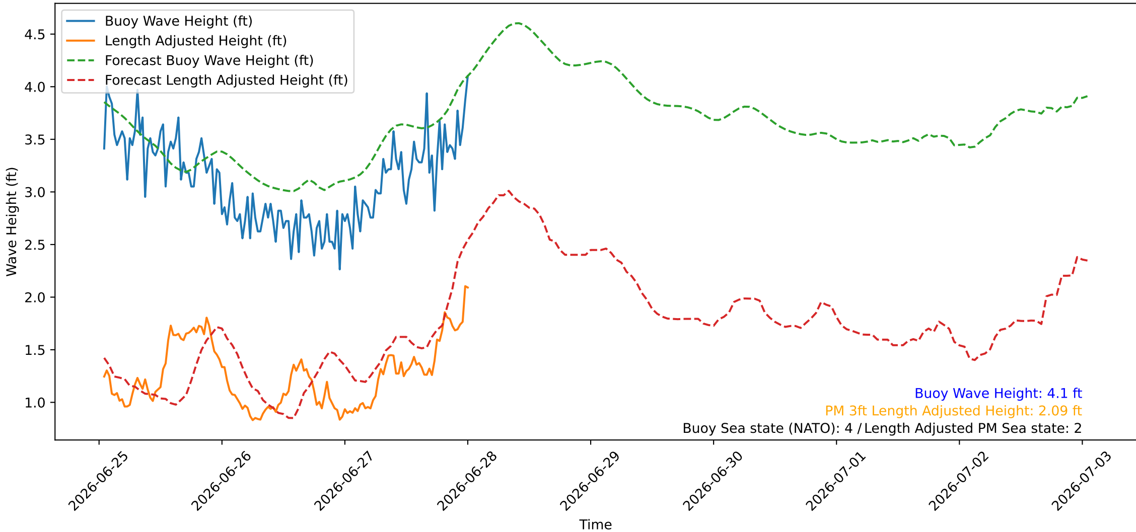
Wave Heights over Time for Green Beach at 2026-06-28 01:01:08
