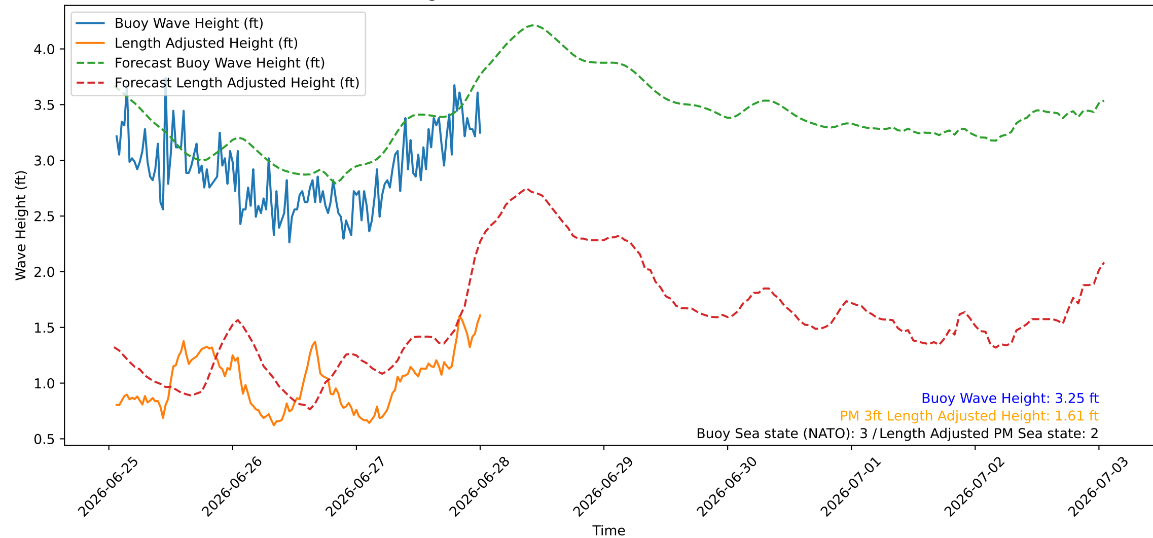
Wave Heights over Time for Red Beach at 2026-06-28 01:00:45
