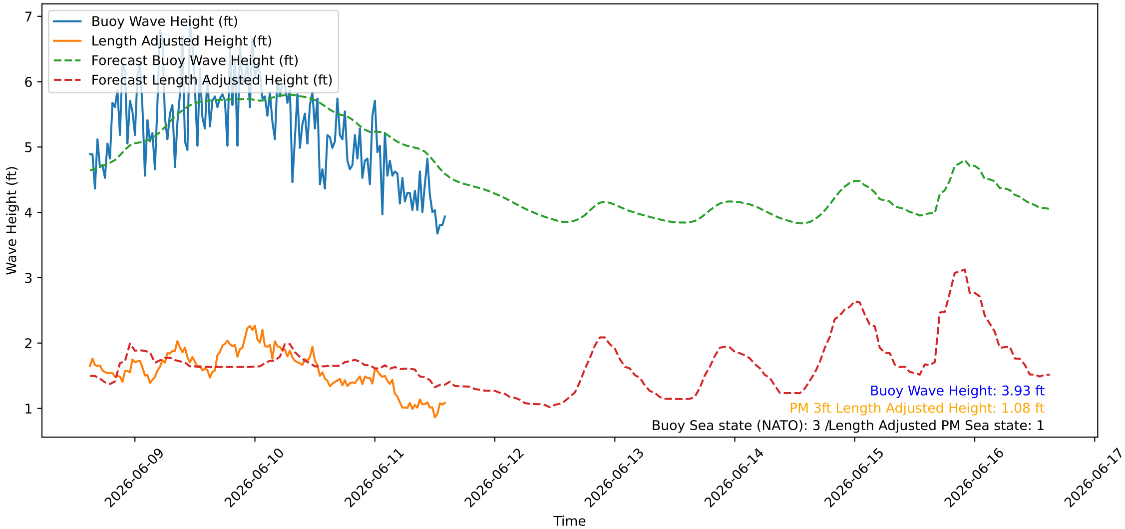
Wave Heights over Time for Green Beach at 2026-06-11 15:01:09
