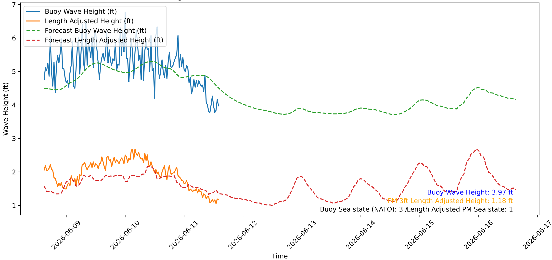
Wave Heights over Time for Oceanside Harbor at 2026-06-11 15:00:27
