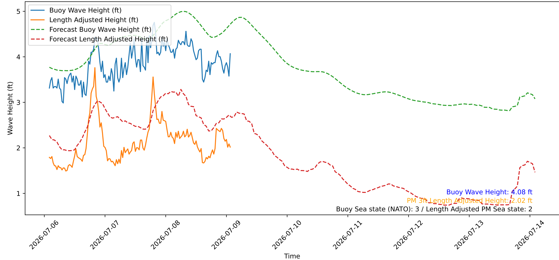
Wave Heights over Time for Green Beach at 2026-07-09 02:11:09
