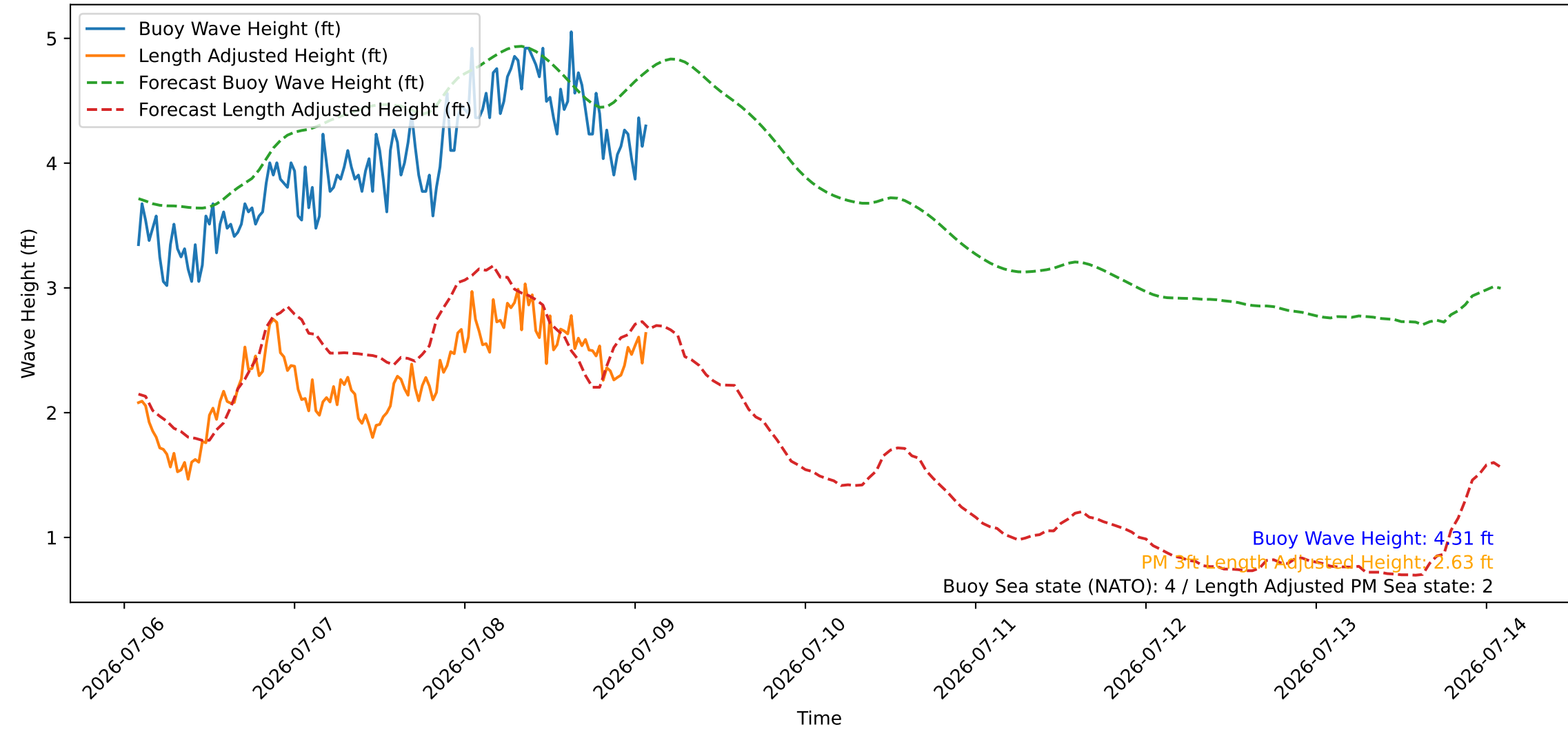
Wave Heights over Time for Oceanside Harbor at 2026-07-09 02:10:27
