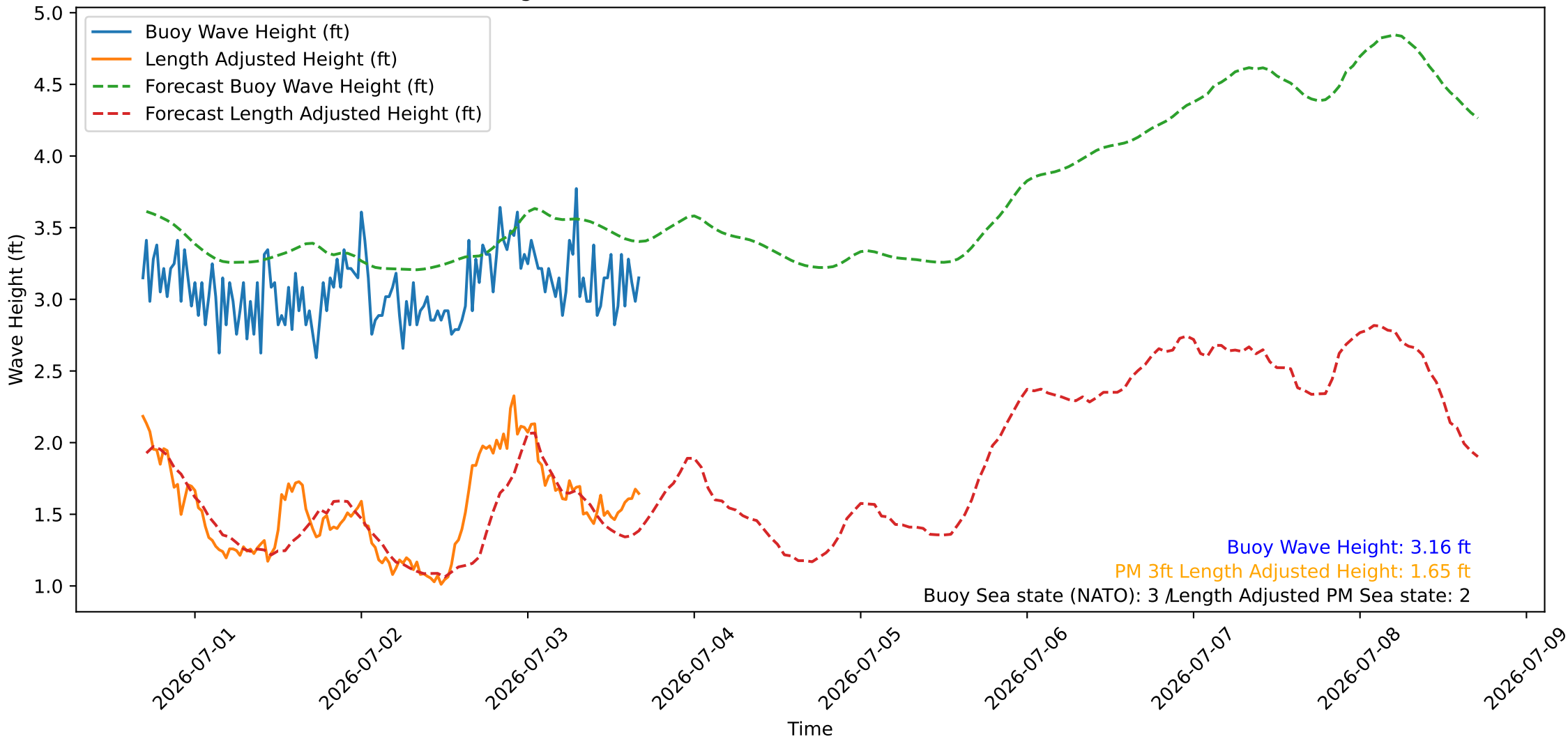
Wave Heights over Time for Oceanside Harbor at 2026-07-03 16:30:26
