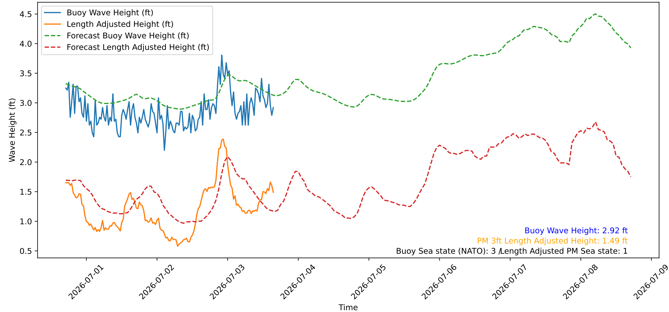
Wave Heights over Time for Red Beach at 2026-07-03 16:30:46
