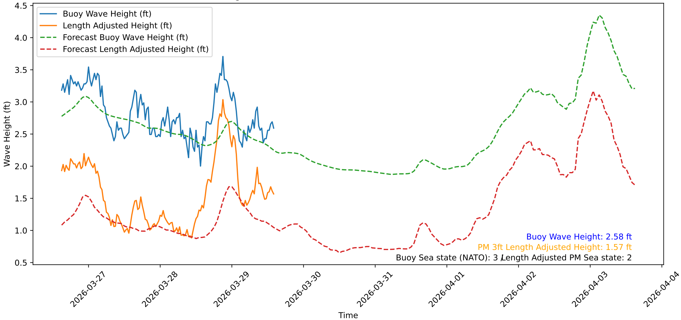
Wave Heights over Time for Green Beach at 2026-03-29 14:51:08
