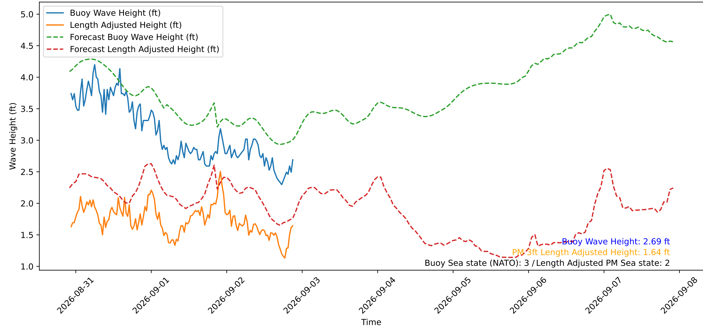
Wave Heights over Time for Red Beach at 2026-09-02 22:00:50
