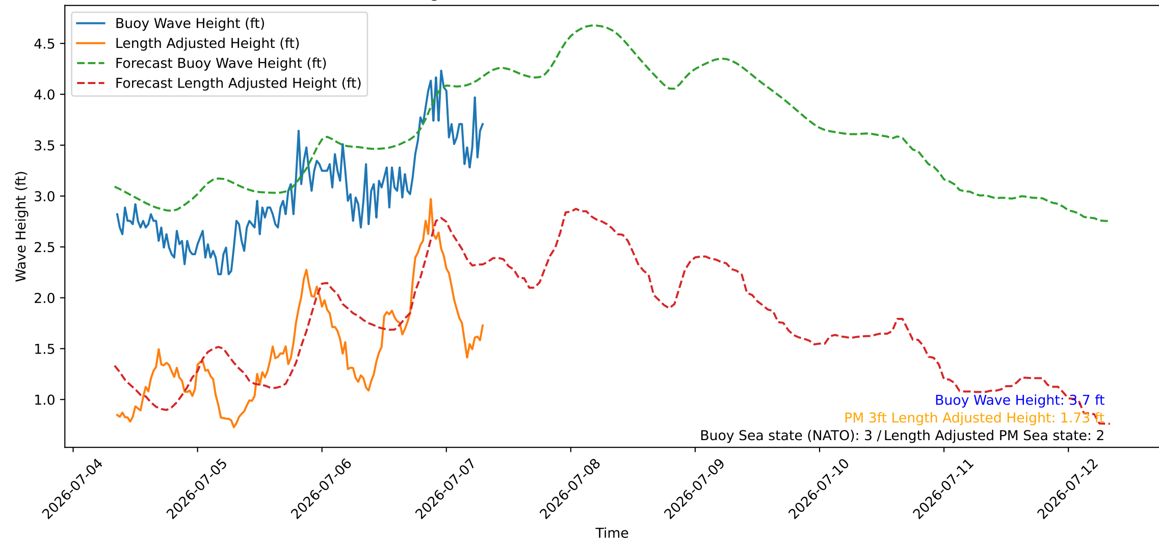
Wave Heights over Time for Red Beach at 2026-07-07 08:00:45
