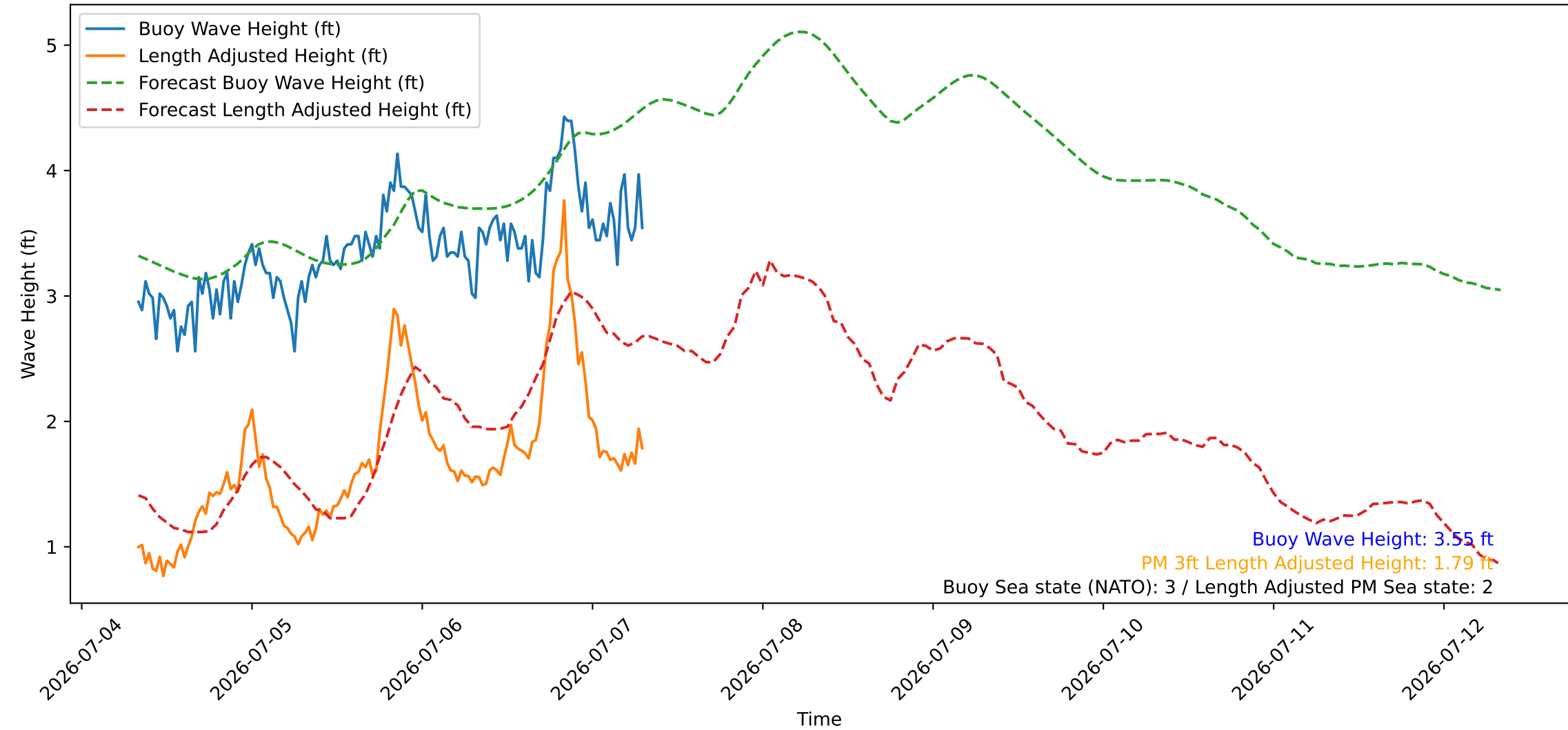
Wave Heights over Time for Green Beach at 2026-07-07 08:01:08
