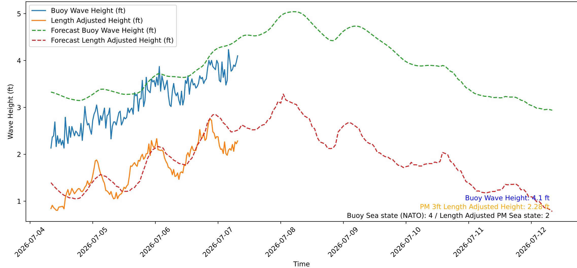
Wave Heights over Time for Oceanside Harbor at 2026-07-07 08:00:26
