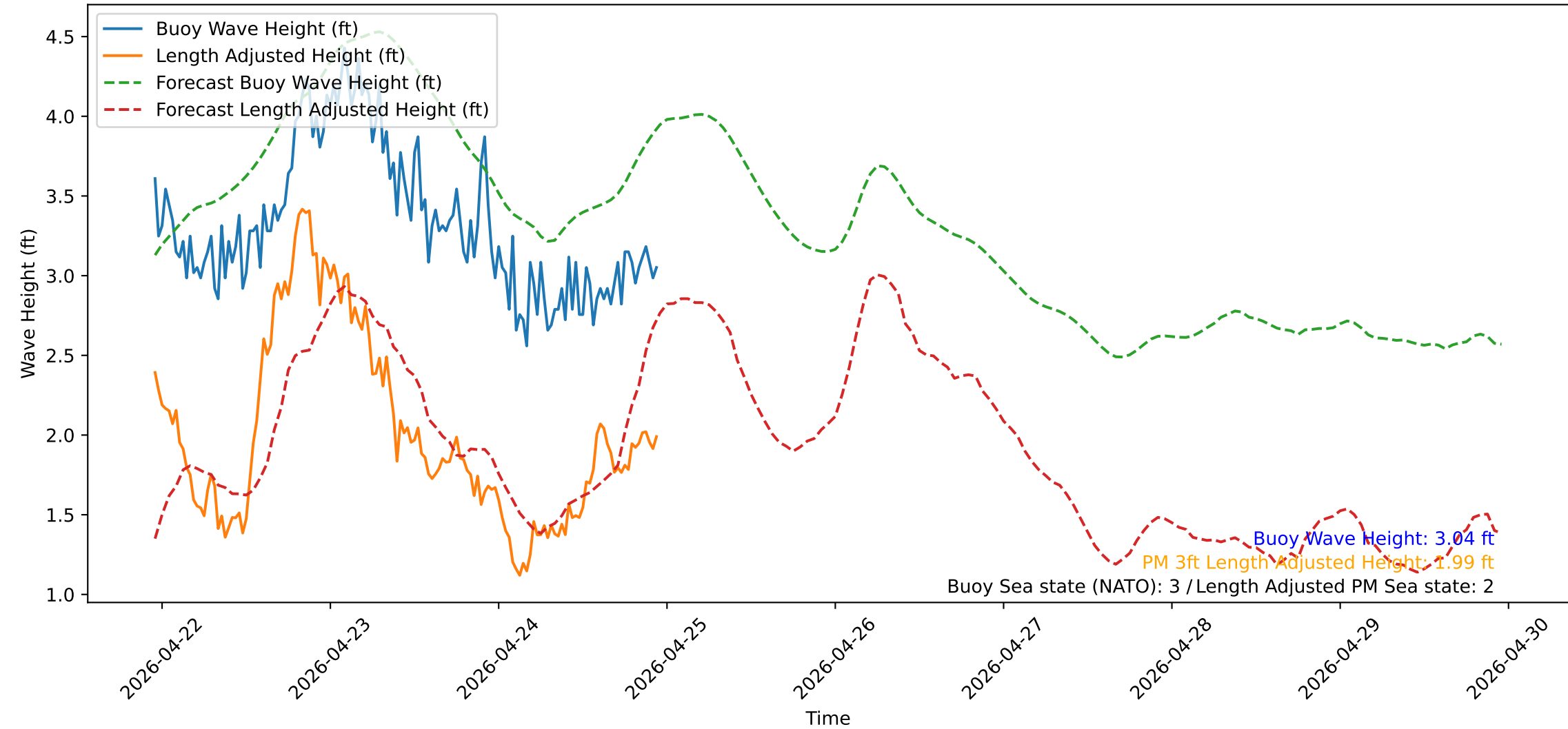
Wave Heights over Time for Oceanside Harbor at 2026-04-24 23:10:32
