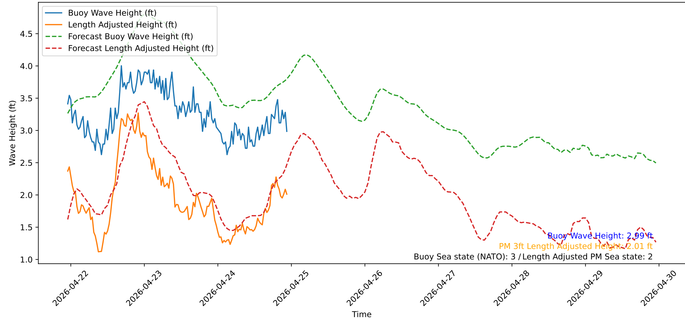
Wave Heights over Time for Green Beach at 2026-04-24 23:11:13
