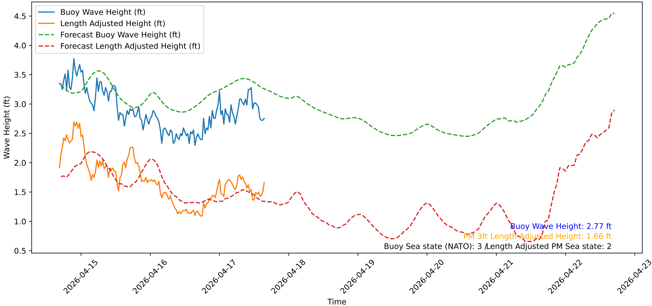
Wave Heights over Time for Oceanside Harbor at 2026-04-17 16:30:32
