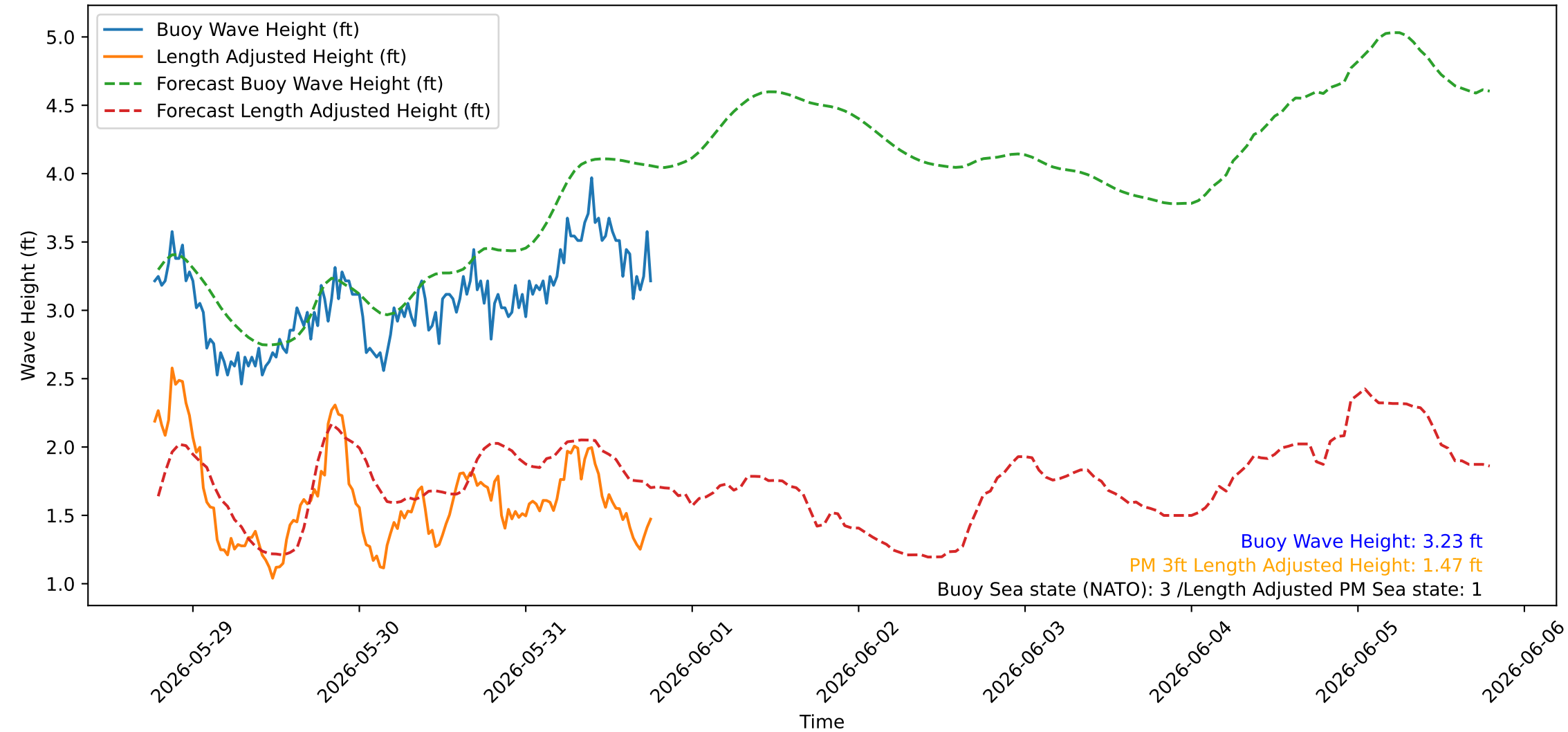
Wave Heights over Time for Green Beach at 2026-05-31 18:41:08
