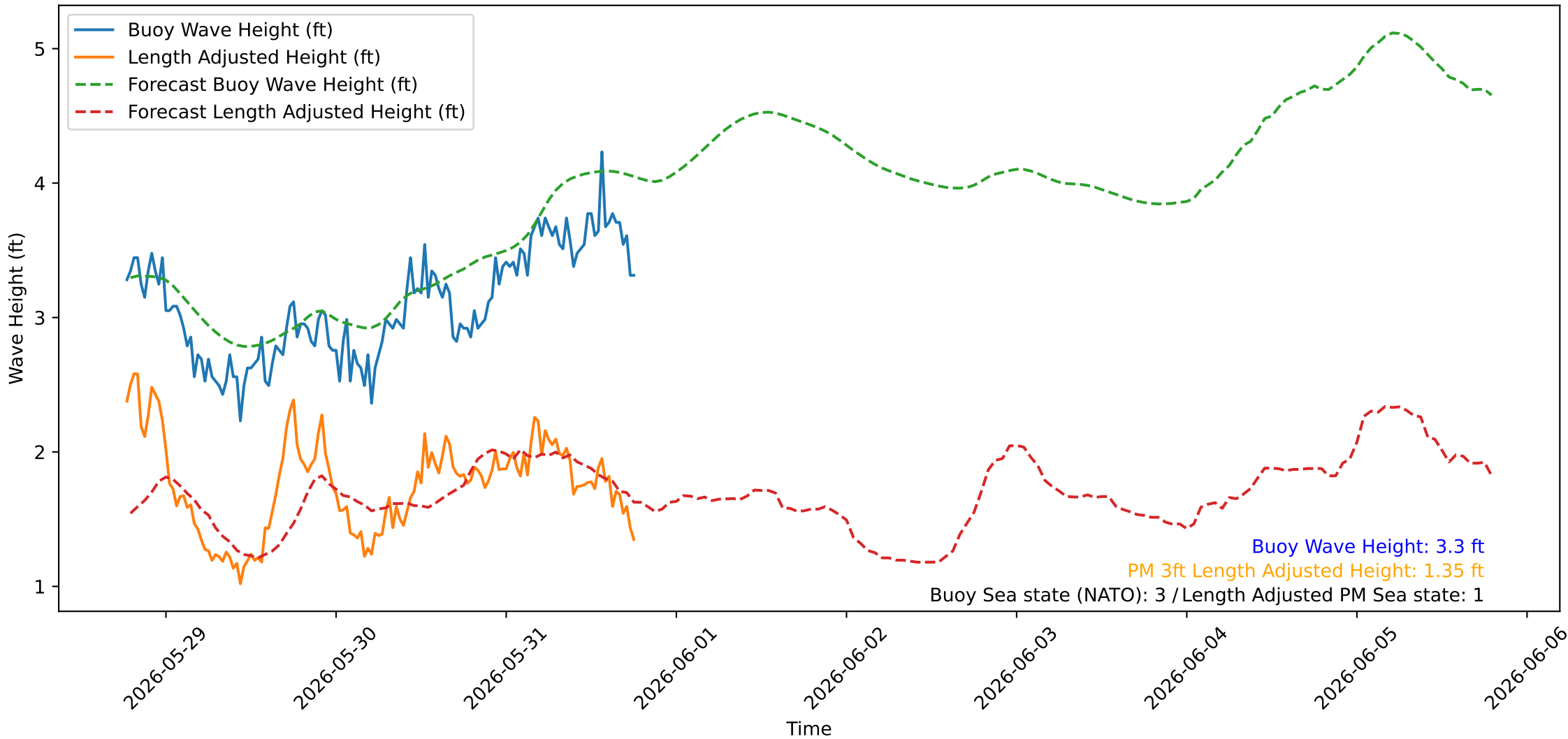
Wave Heights over Time for Oceanside Harbor at 2026-05-31 18:40:25
