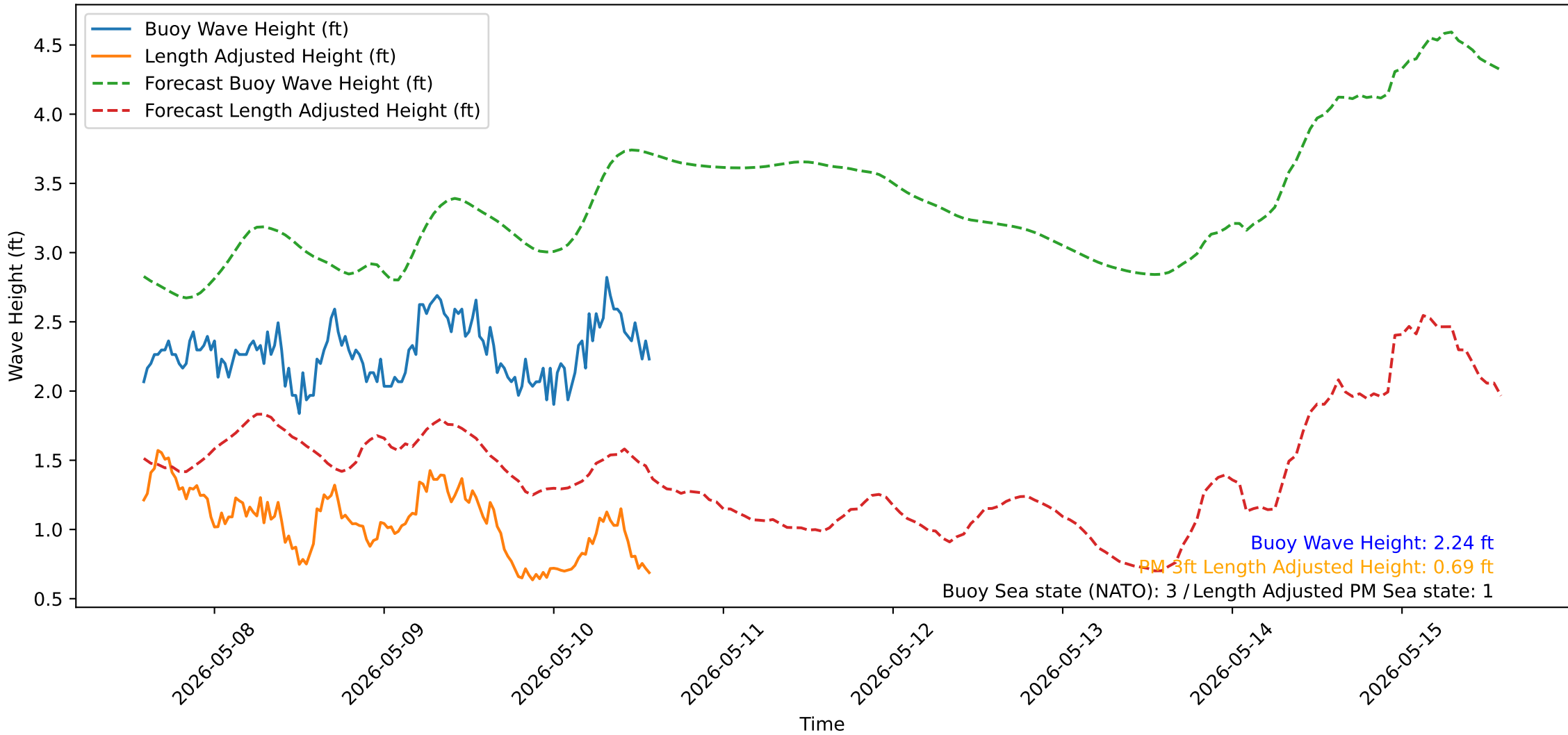
Wave Heights over Time for Green Beach at 2026-05-10 14:11:15
