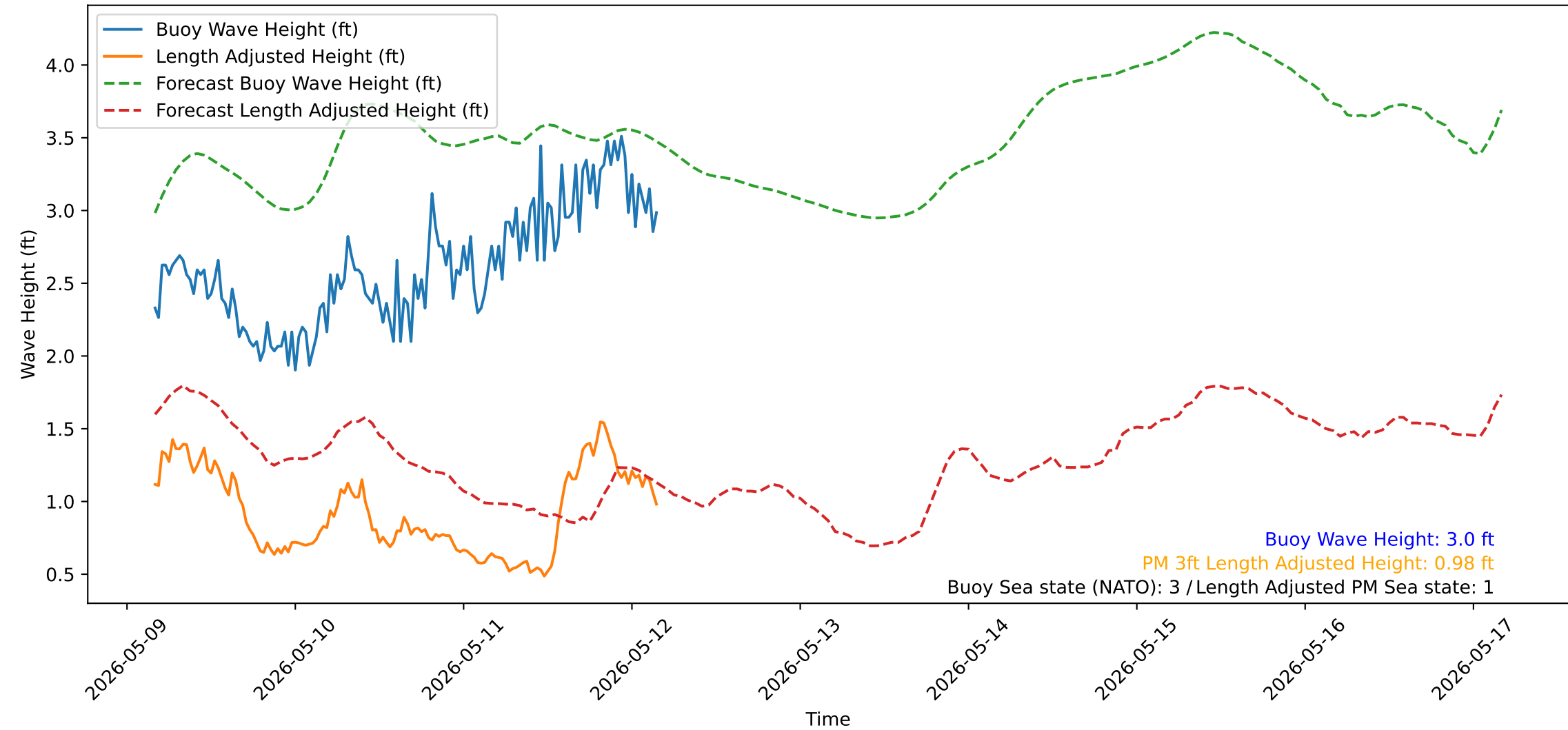
Wave Heights over Time for Green Beach at 2026-05-12 04:11:13
