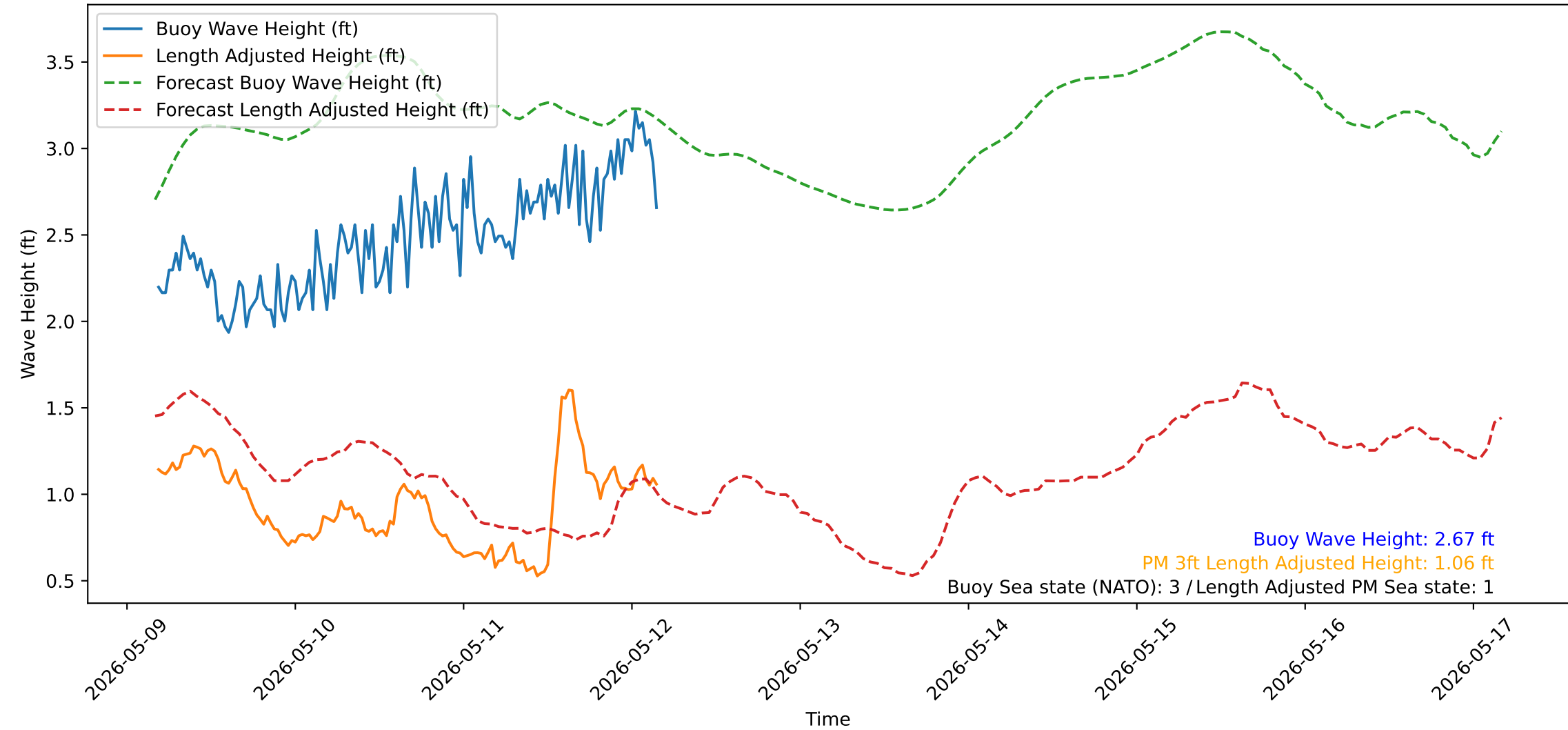
Wave Heights over Time for Red Beach at 2026-05-12 04:10:51
