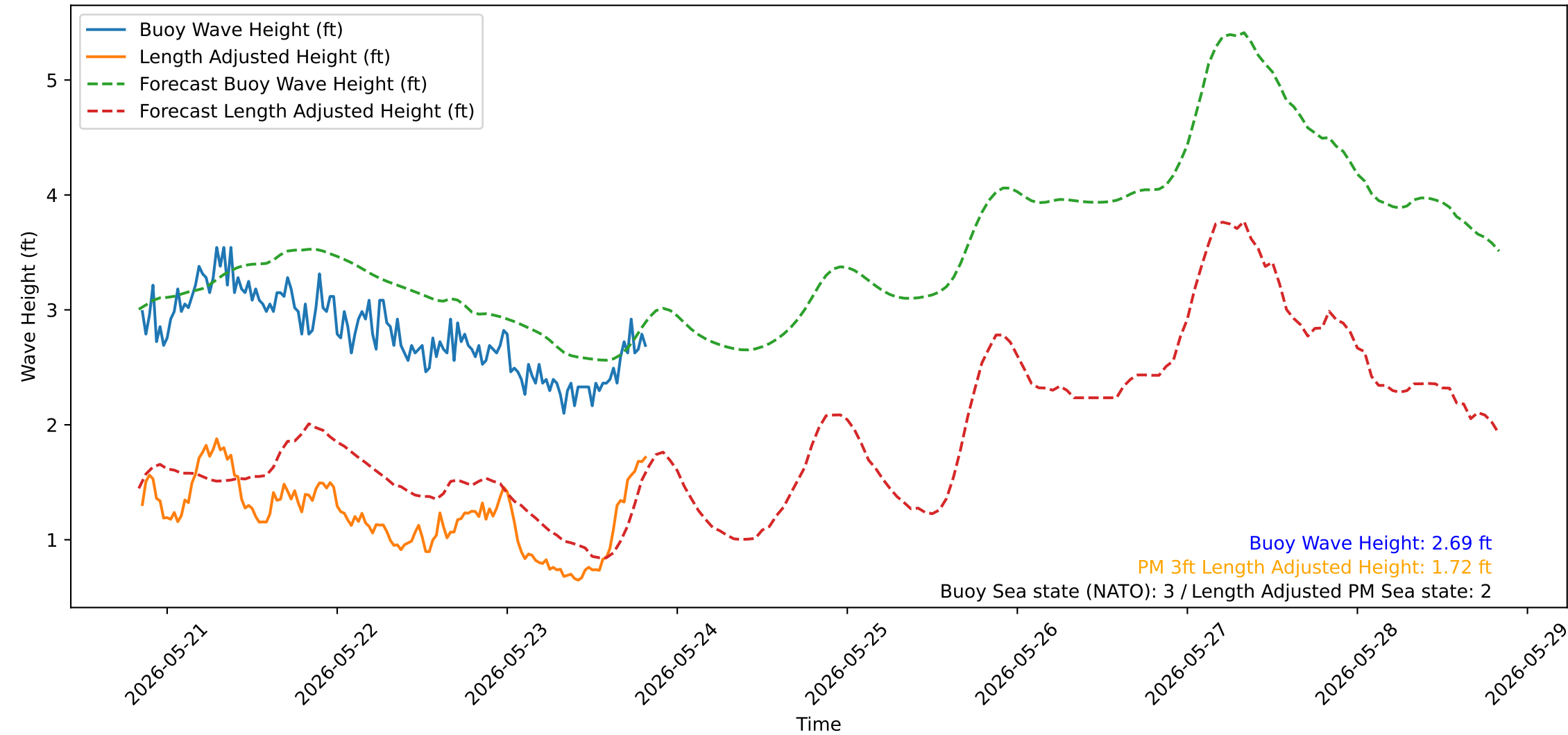
Wave Heights over Time for Green Beach at 2026-05-23 20:21:15
