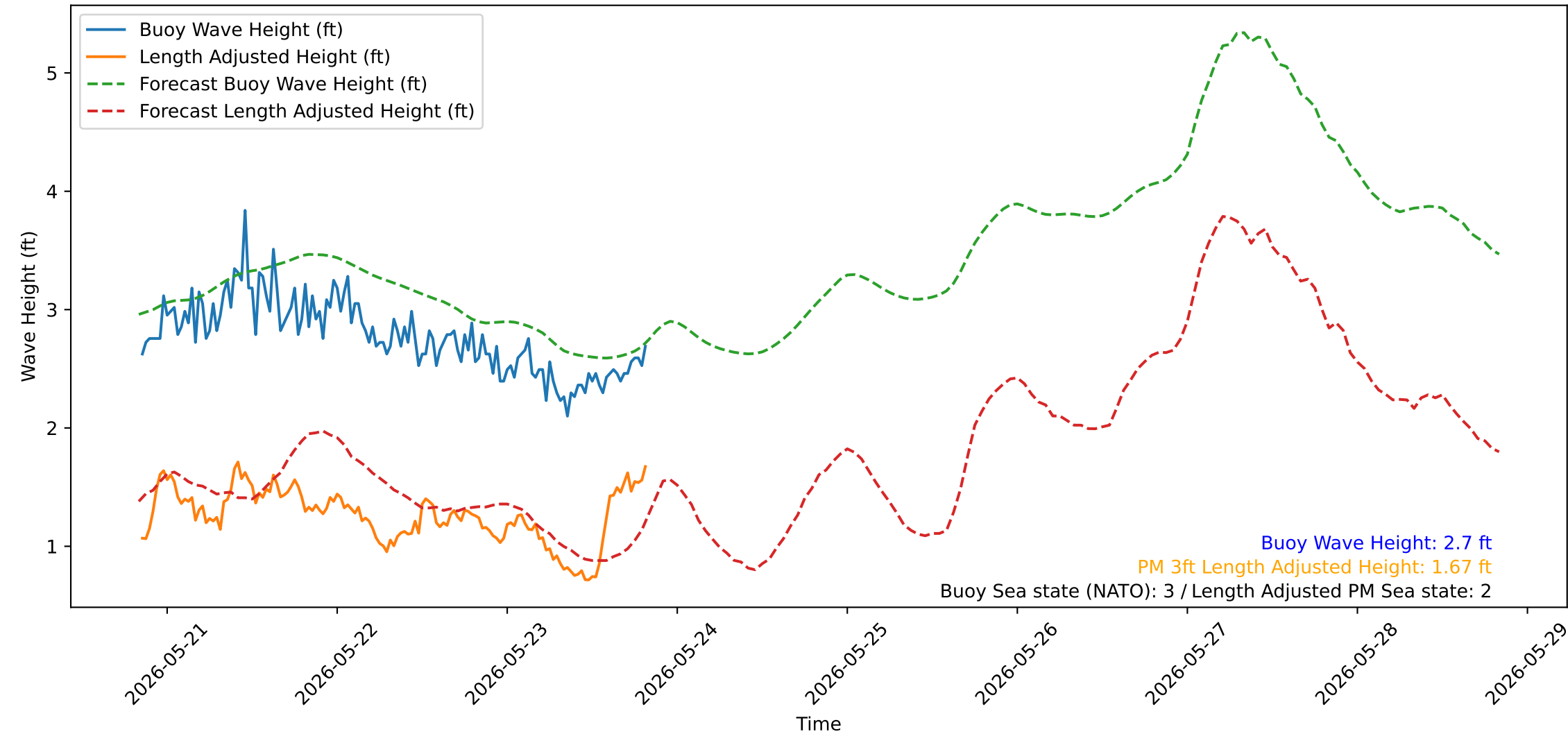
Wave Heights over Time for Oceanside Harbor at 2026-05-23 20:20:32
