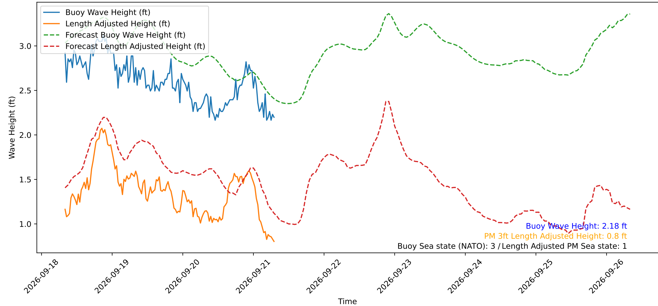
Wave Heights over Time for Green Beach at 2026-09-21 07:51:13
