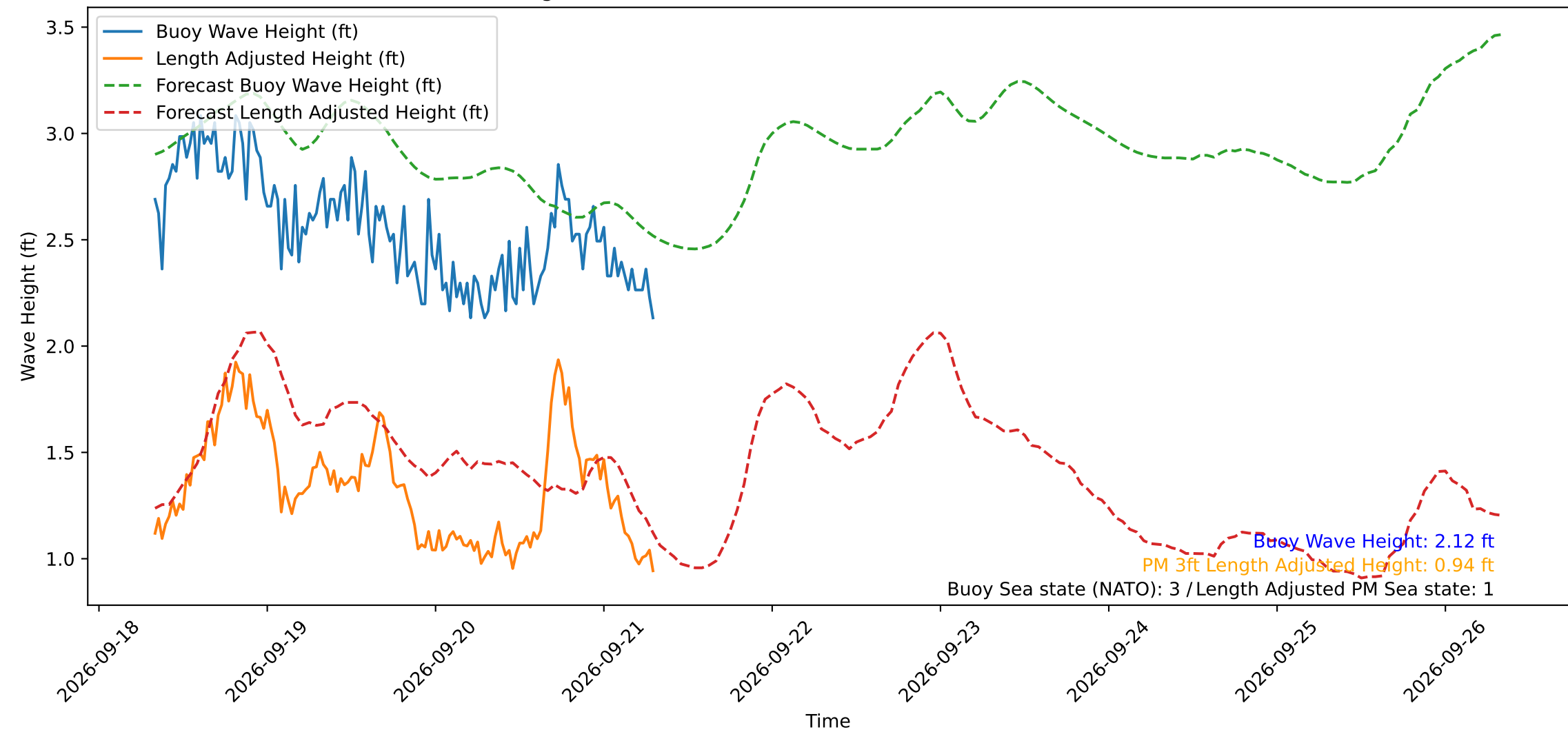
Wave Heights over Time for Oceanside Harbor at 2026-09-21 07:50:30
