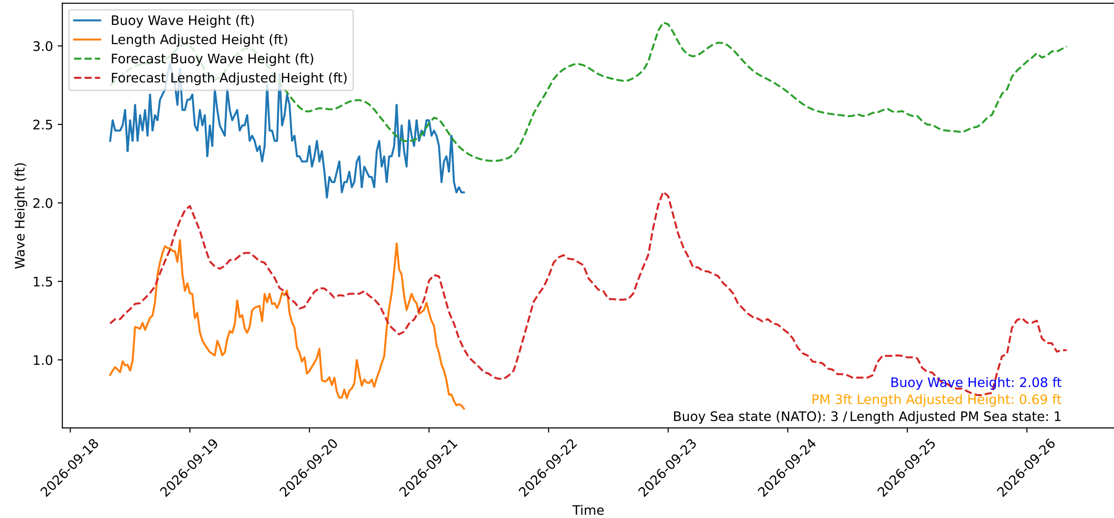
Wave Heights over Time for Red Beach at 2026-09-21 07:50:50
