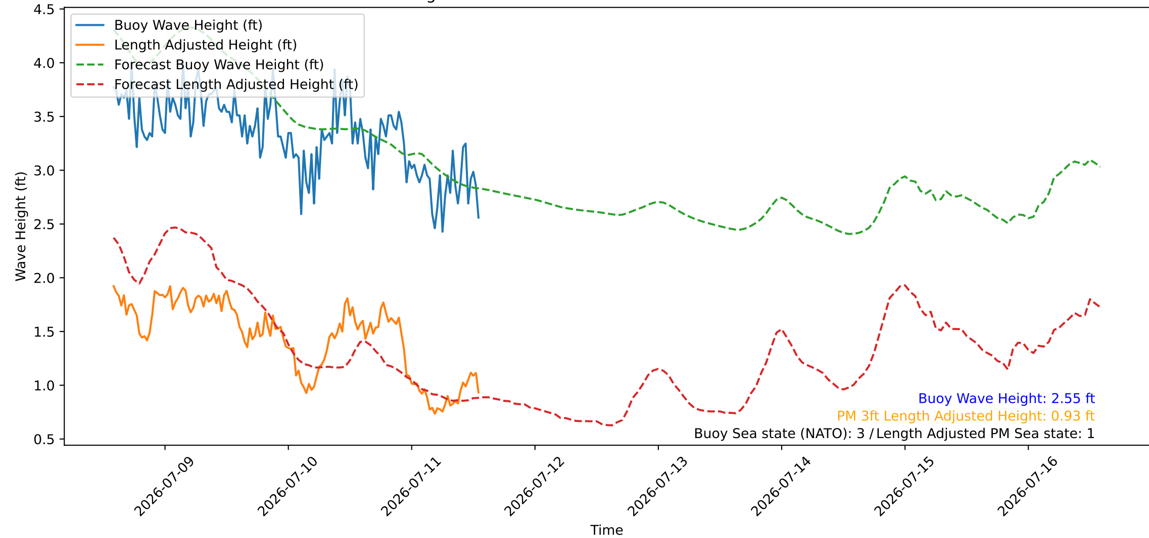
Wave Heights over Time for Red Beach at 2026-07-11 13:50:47
