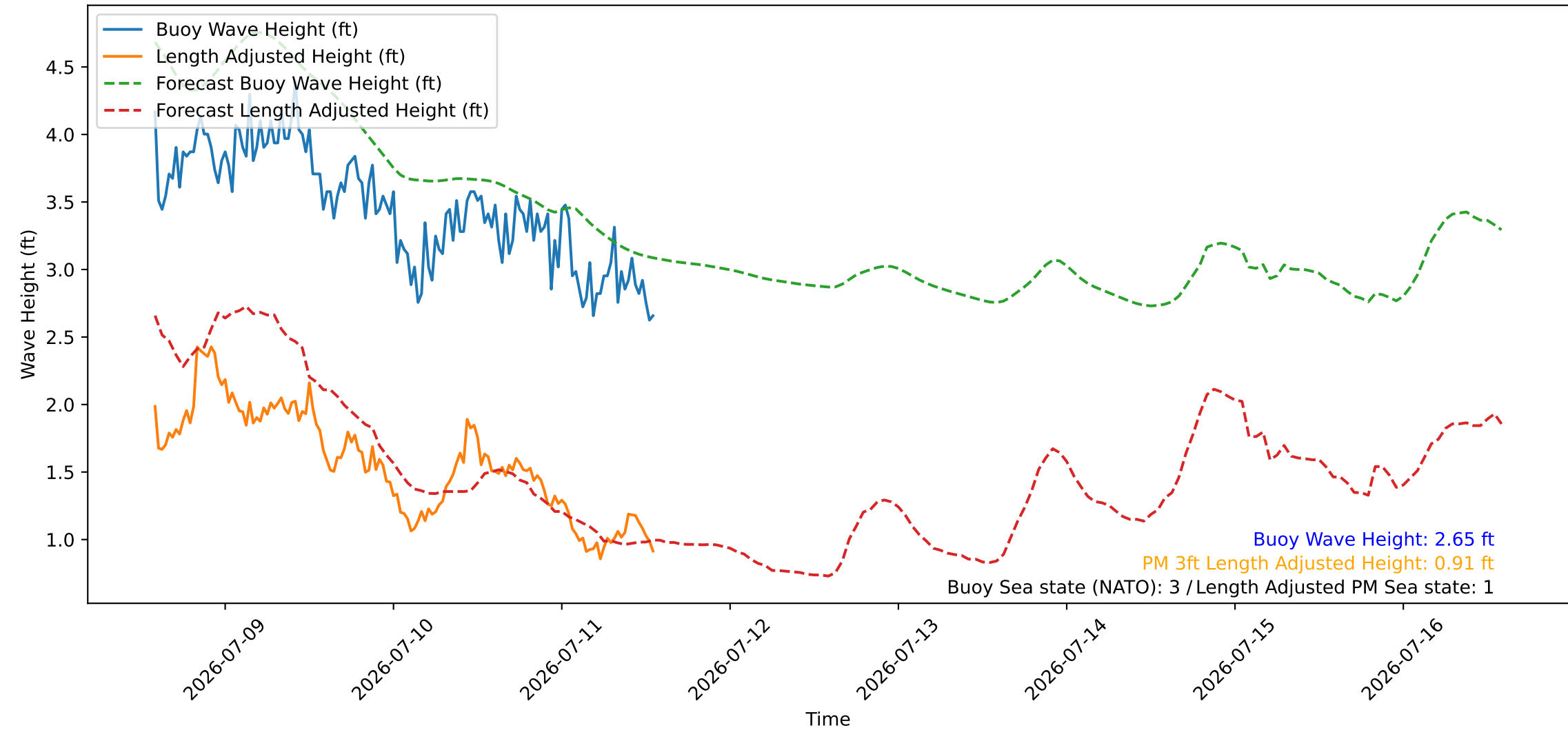
Wave Heights over Time for Green Beach at 2026-07-11 13:51:09
