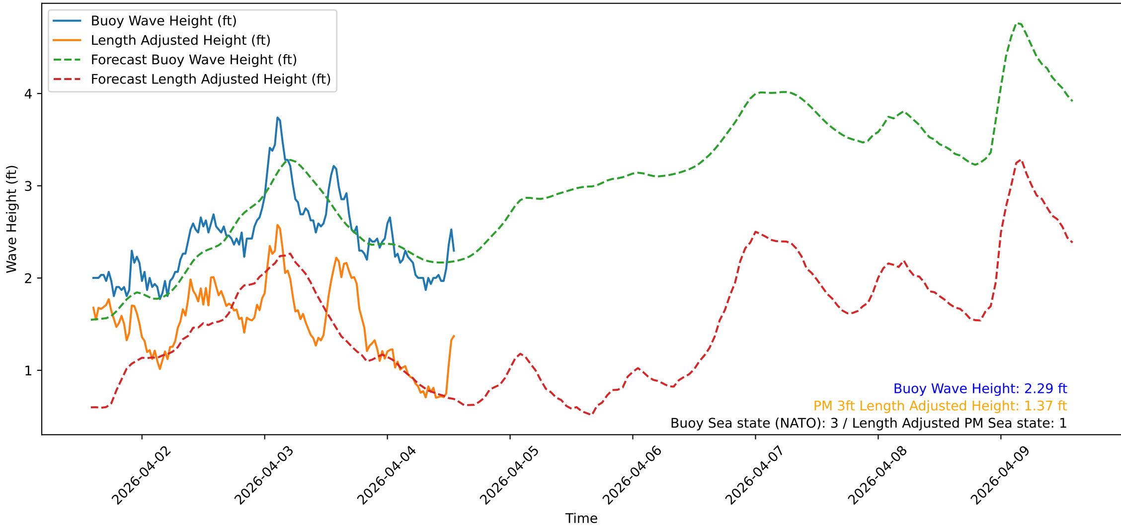
Wave Heights over Time for Red Beach at 2026-04-04 14:00:49
