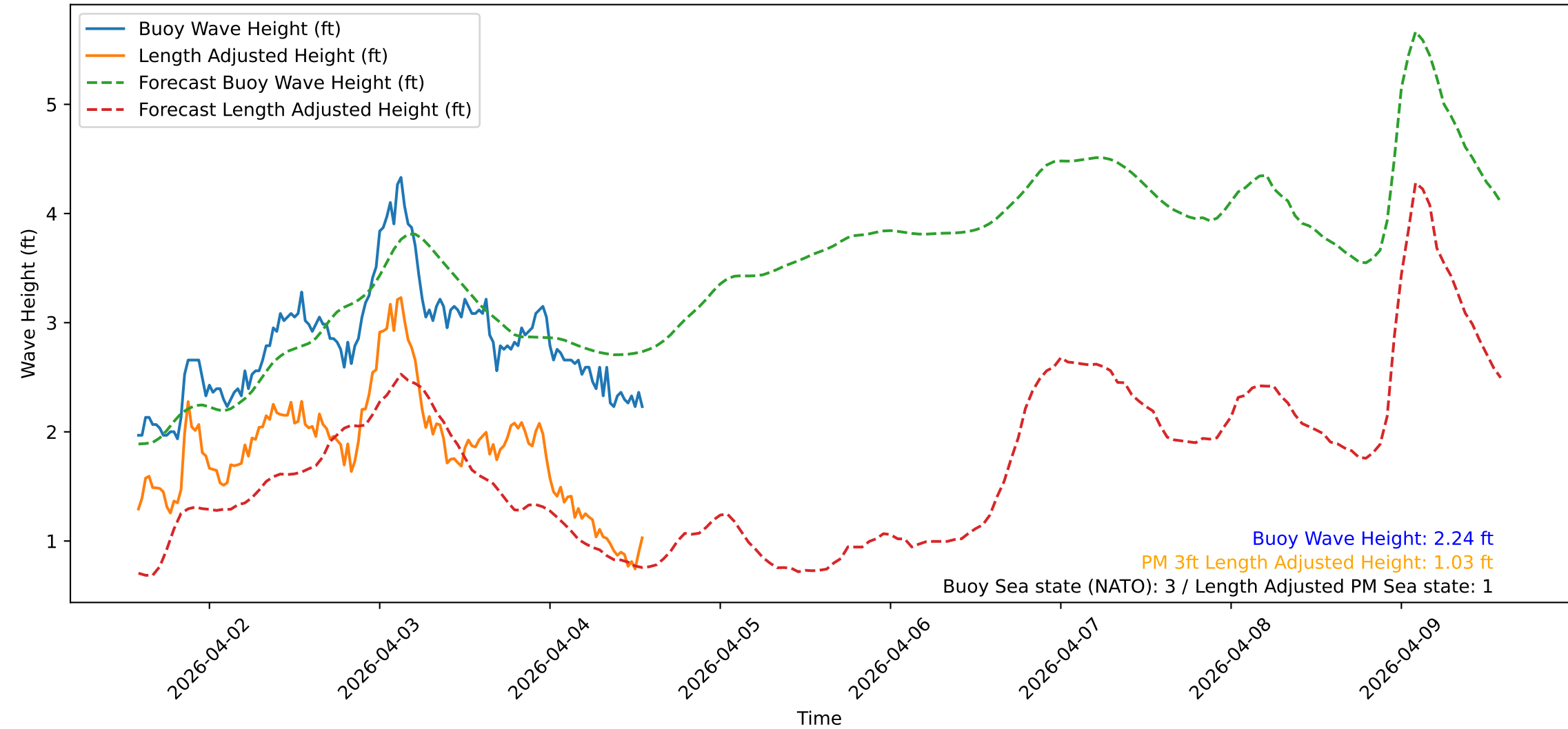
Wave Heights over Time for Green Beach at 2026-04-04 14:01:11
