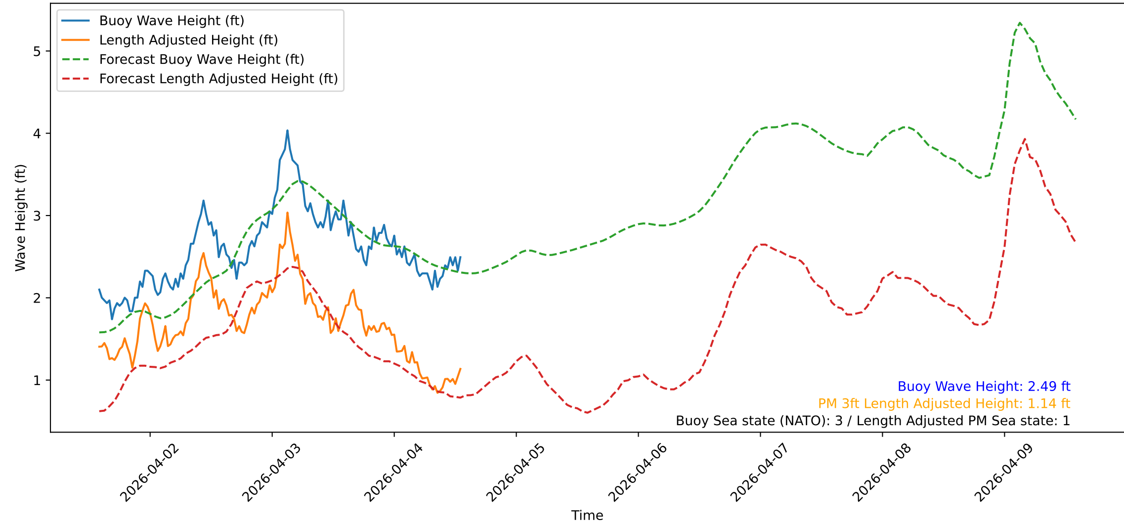
Wave Heights over Time for Oceanside Harbor at 2026-04-04 14:00:32
