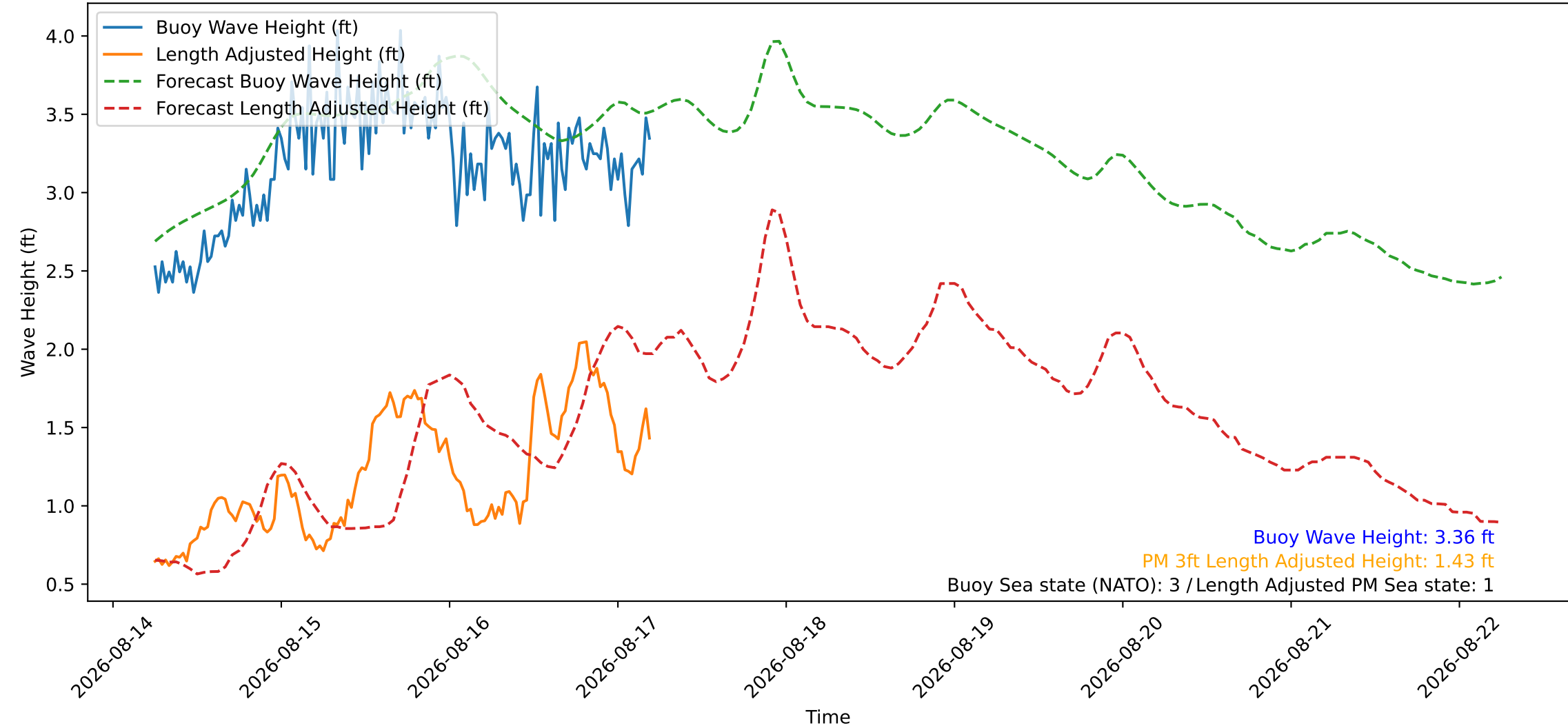
Wave Heights over Time for Red Beach at 2026-08-17 05:30:45
