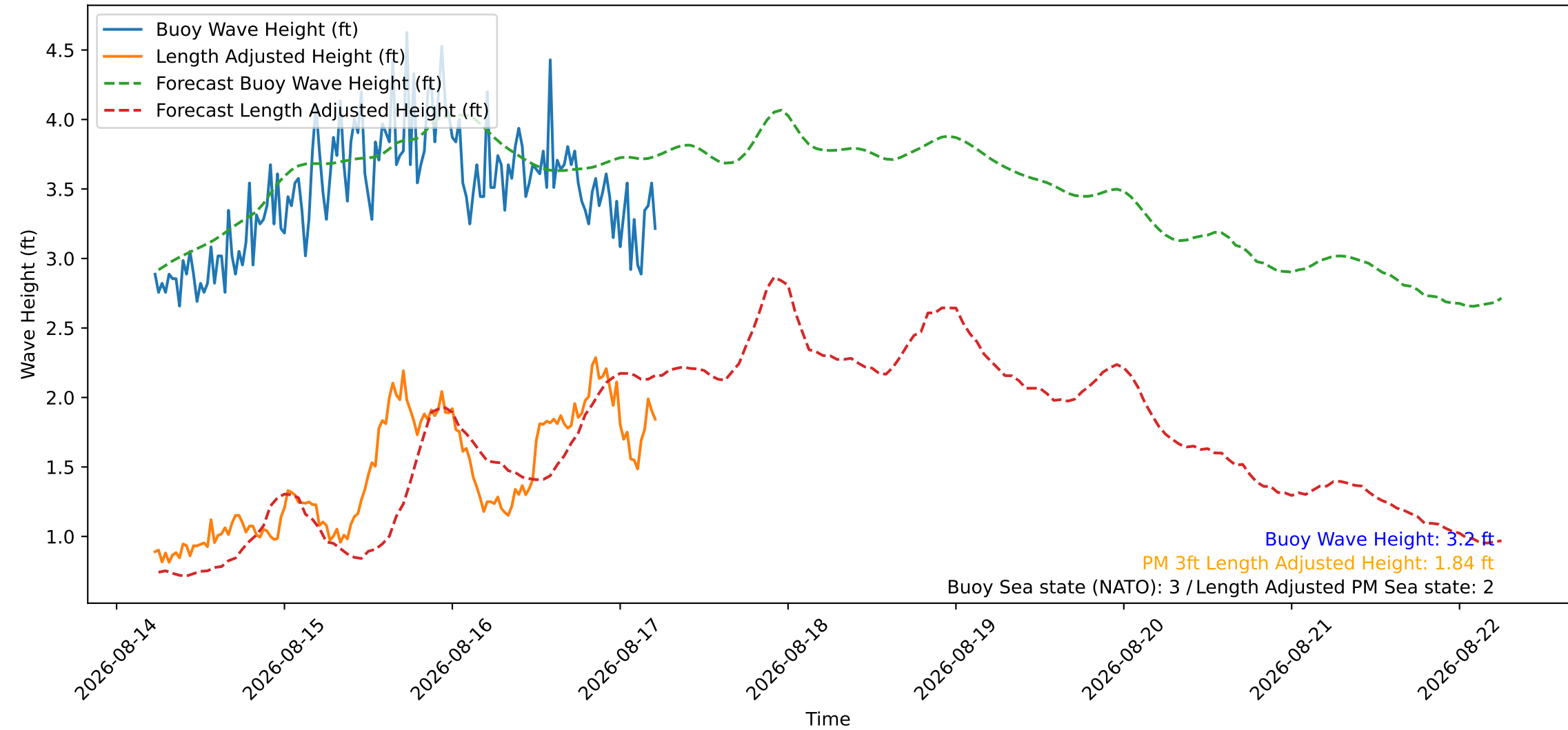
Wave Heights over Time for Oceanside Harbor at 2026-08-17 05:30:26
