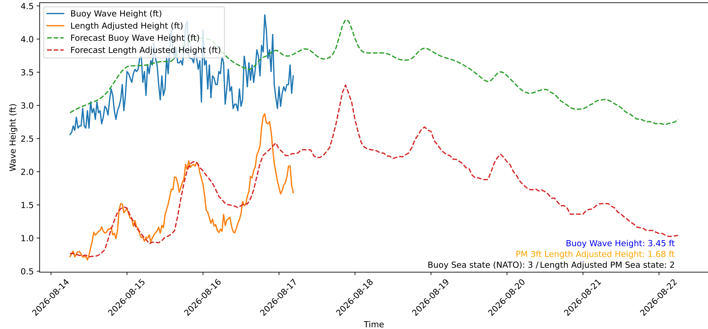
Wave Heights over Time for Green Beach at 2026-08-17 05:31:07
