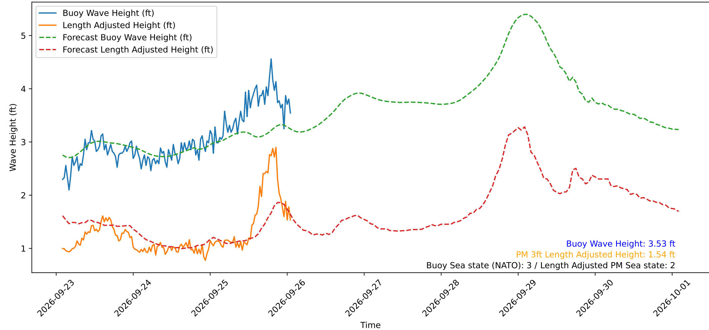
Wave Heights over Time for Green Beach at 2026-09-26 01:41:11
