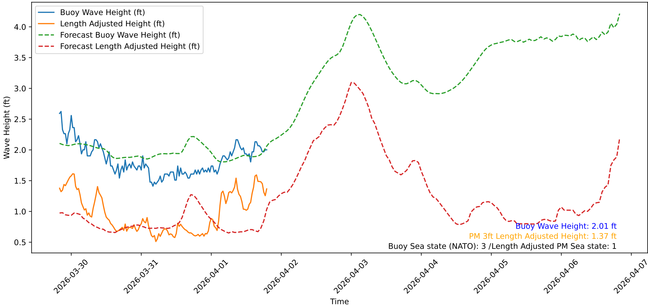
Wave Heights over Time for Green Beach at 2026-04-01 20:01:09
