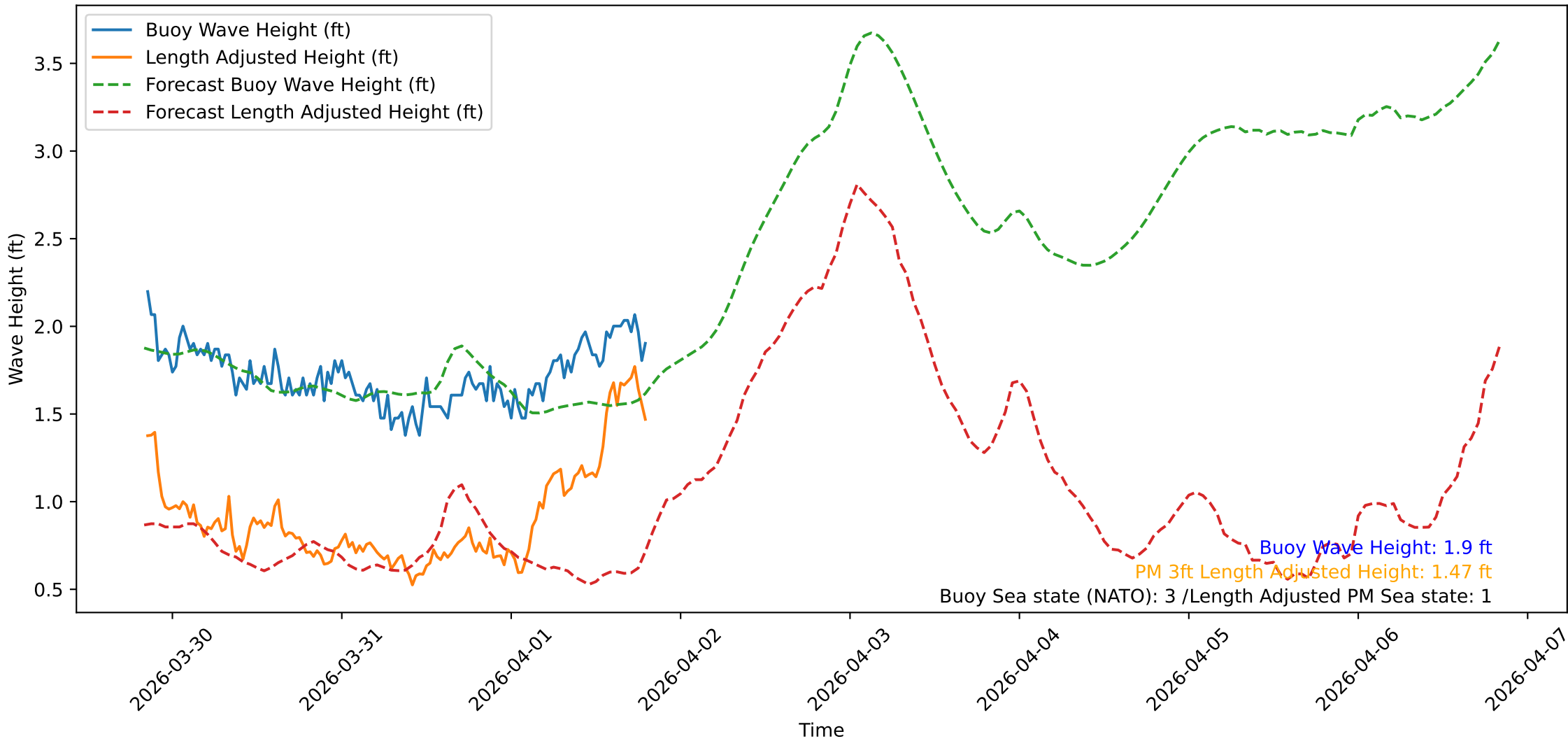
Wave Heights over Time for Red Beach at 2026-04-01 20:00:47
