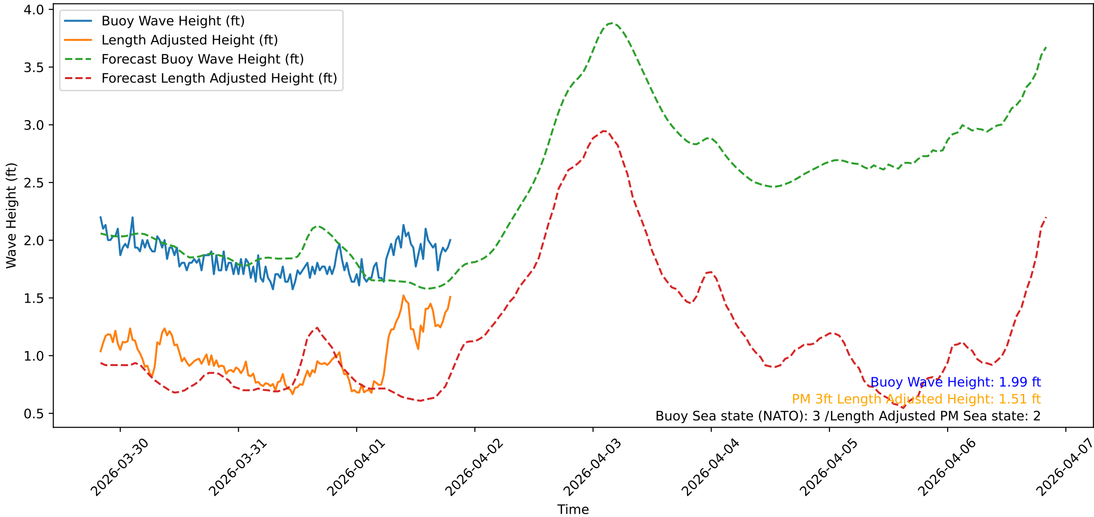
Wave Heights over Time for Oceanside Harbor at 2026-04-01 20:00:31
