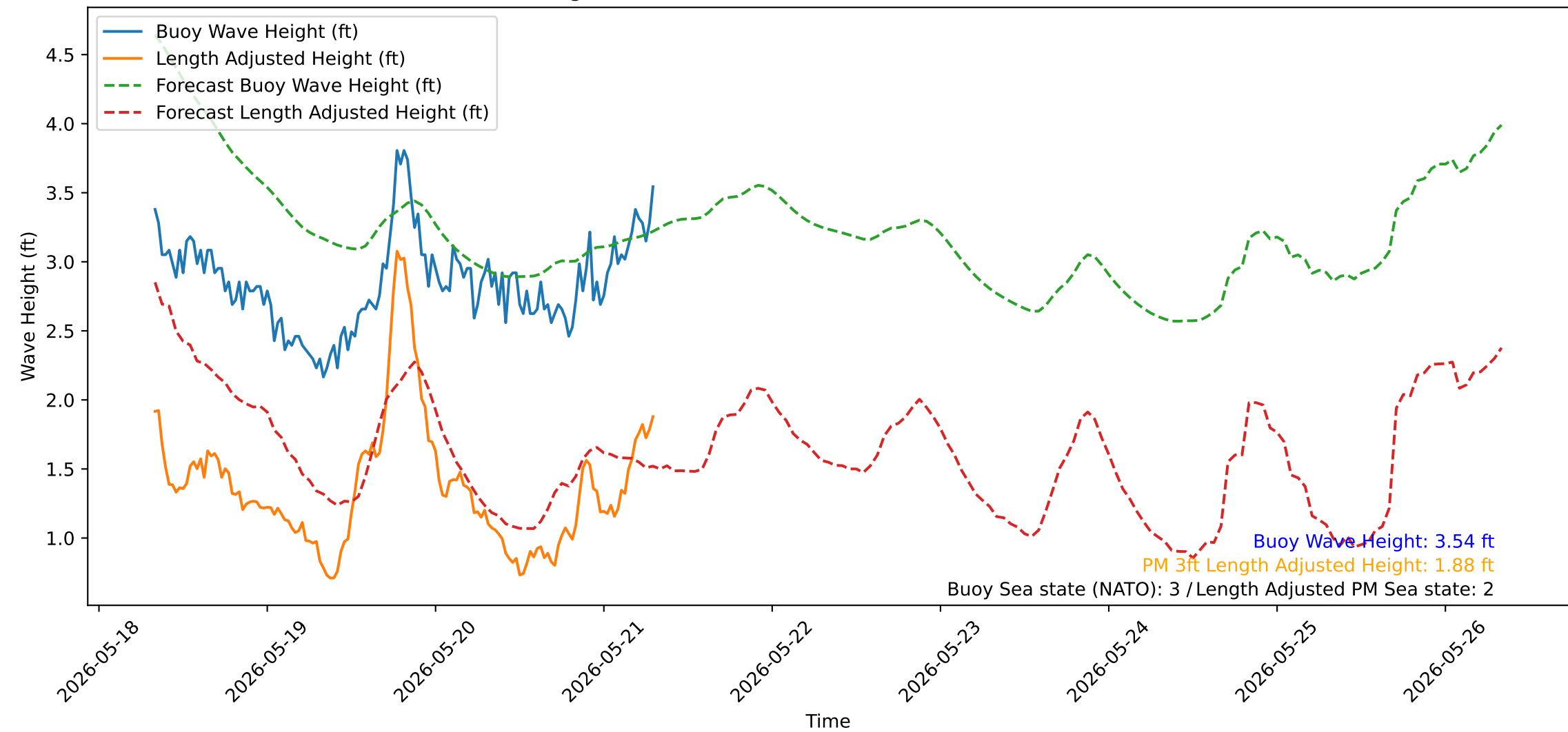
Wave Heights over Time for Green Beach at 2026-05-21 07:51:14
