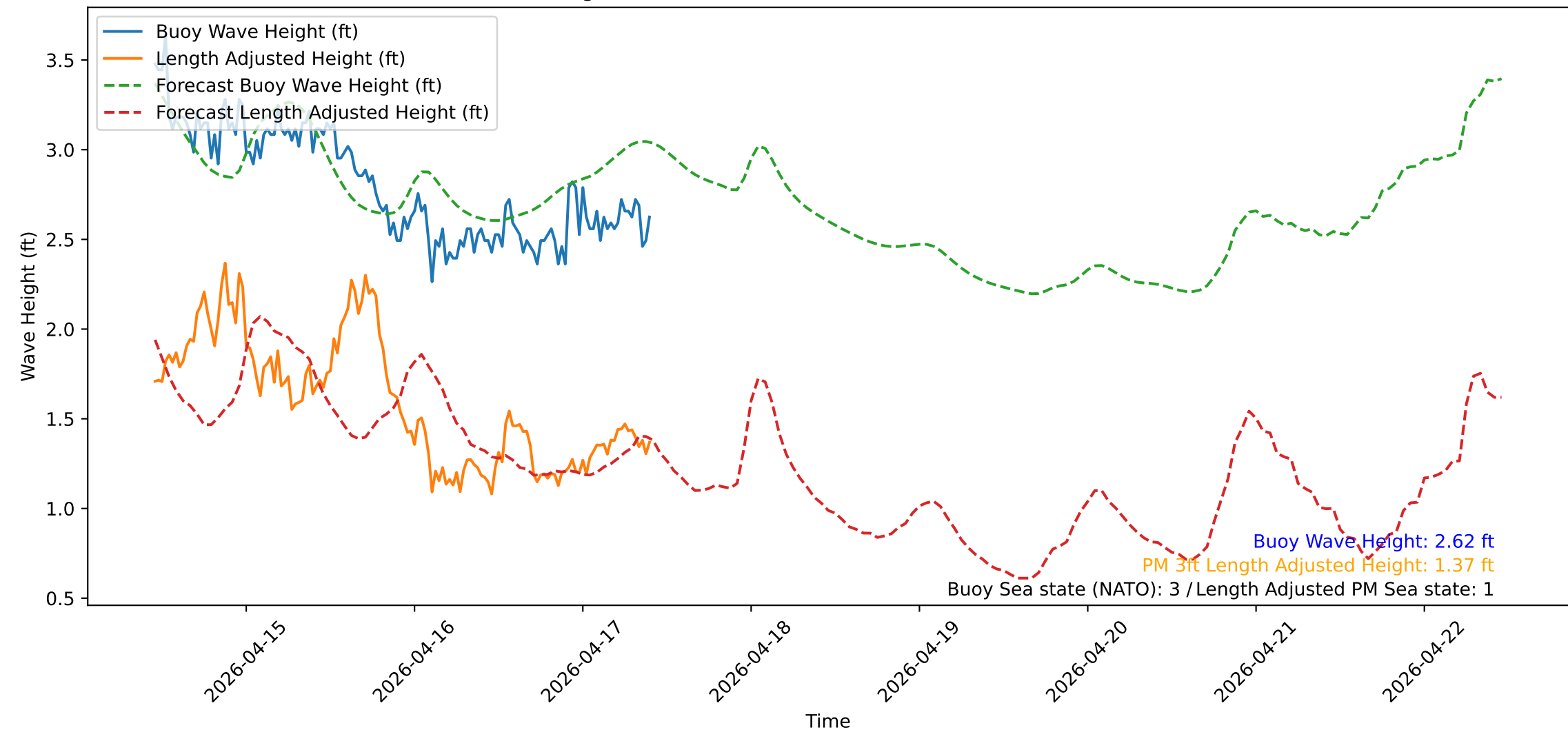
Wave Heights over Time for Red Beach at 2026-04-17 10:30:53
