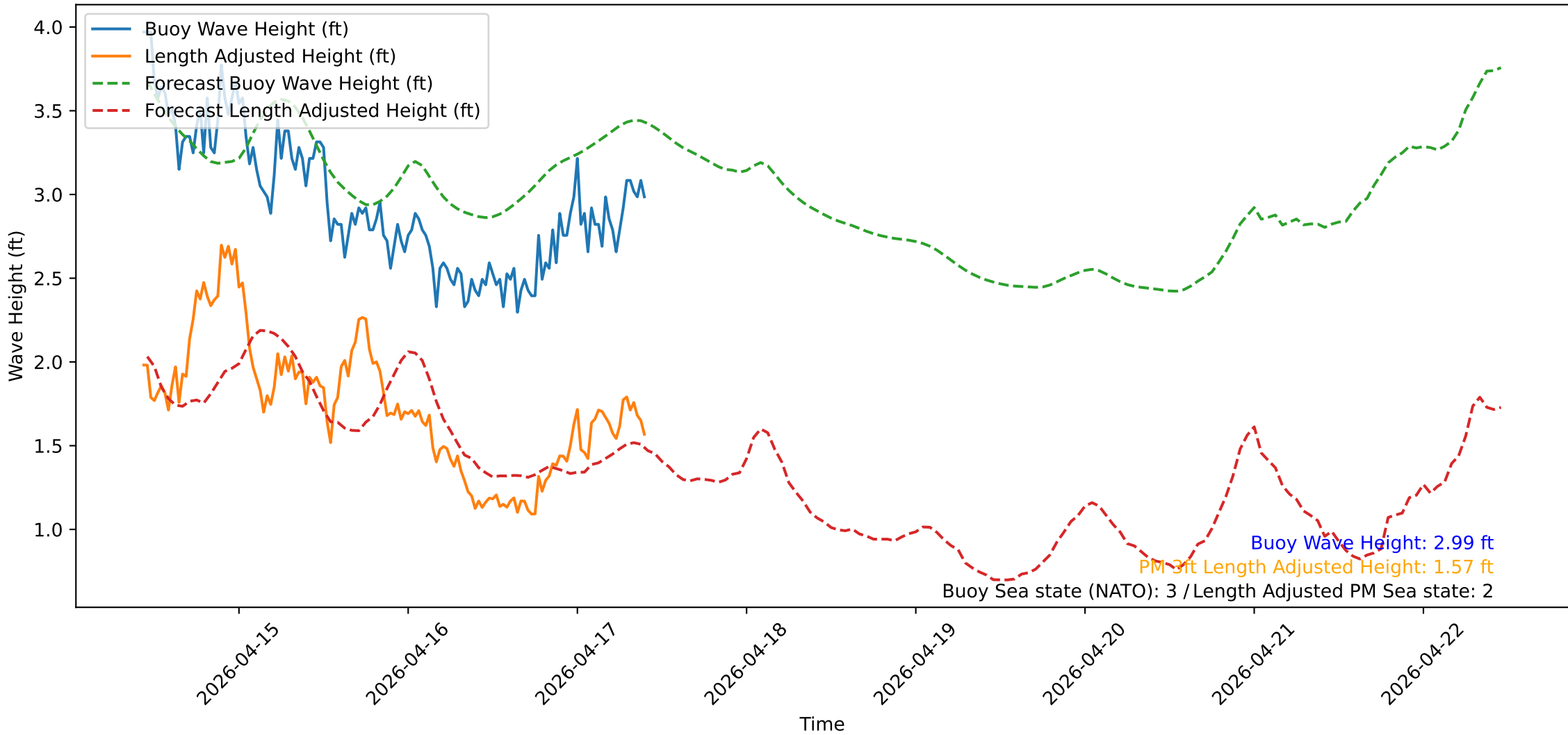
Wave Heights over Time for Oceanside Harbor at 2026-04-17 10:30:32
