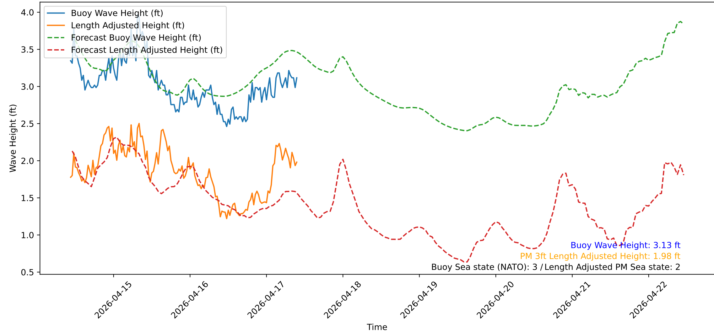
Wave Heights over Time for Green Beach at 2026-04-17 10:31:16
