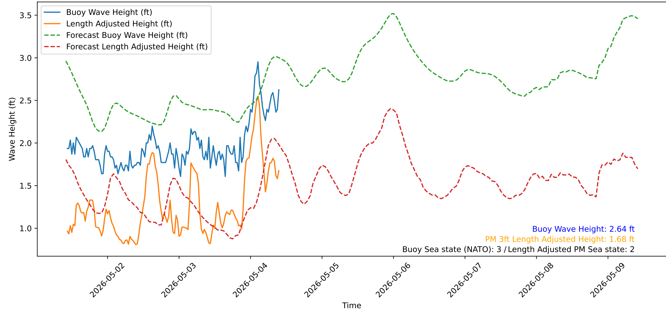
Wave Heights over Time for Red Beach at 2026-05-04 10:20:51
