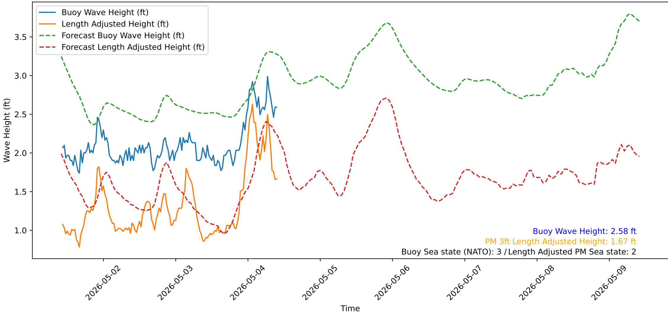
Wave Heights over Time for Green Beach at 2026-05-04 10:21:13
