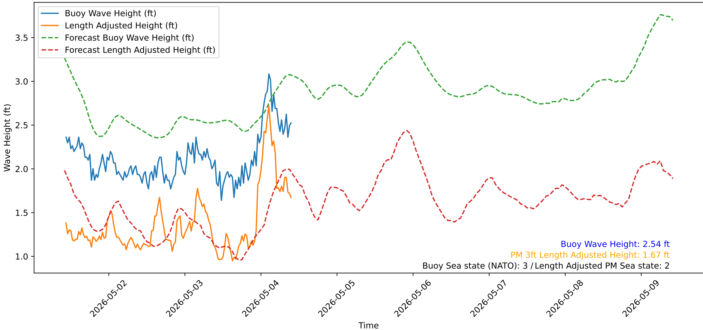
Wave Heights over Time for Oceanside Harbor at 2026-05-04 10:20:31
