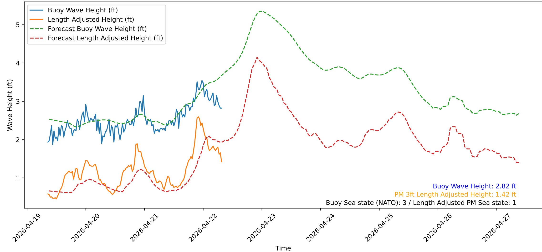
Wave Heights over Time for Green Beach at 2026-04-22 08:31:13
