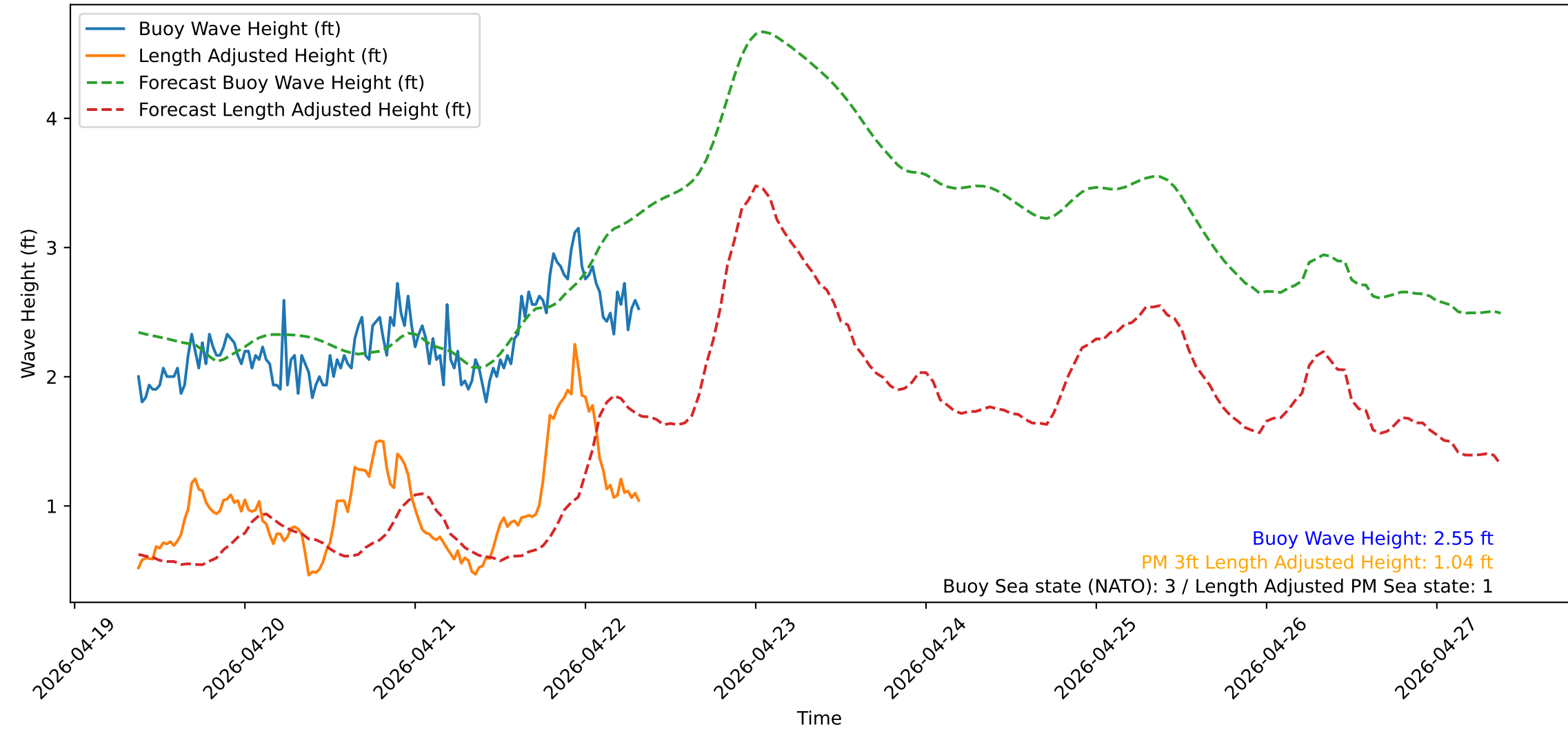
Wave Heights over Time for Red Beach at 2026-04-22 08:30:50
