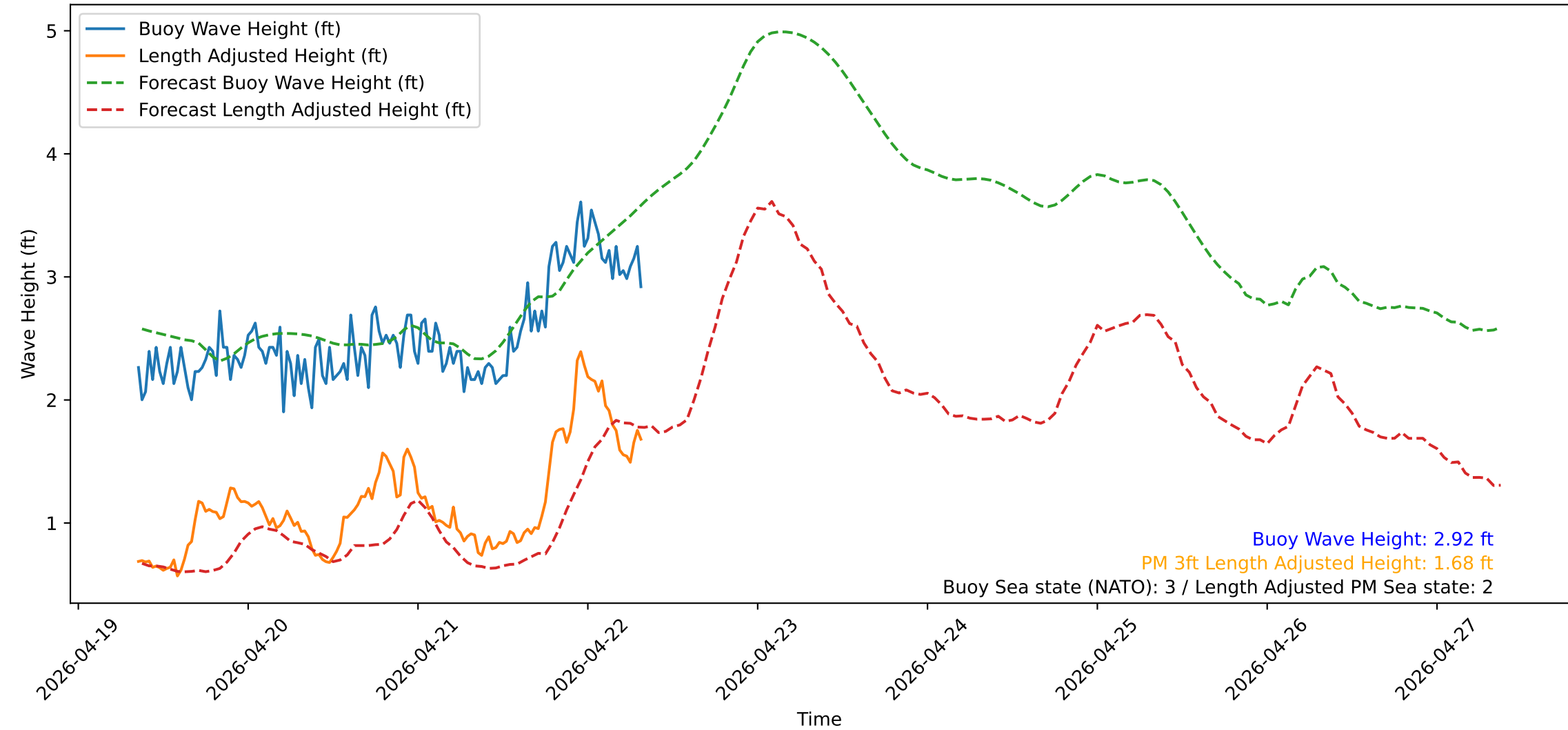
Wave Heights over Time for Oceanside Harbor at 2026-04-22 08:30:31
