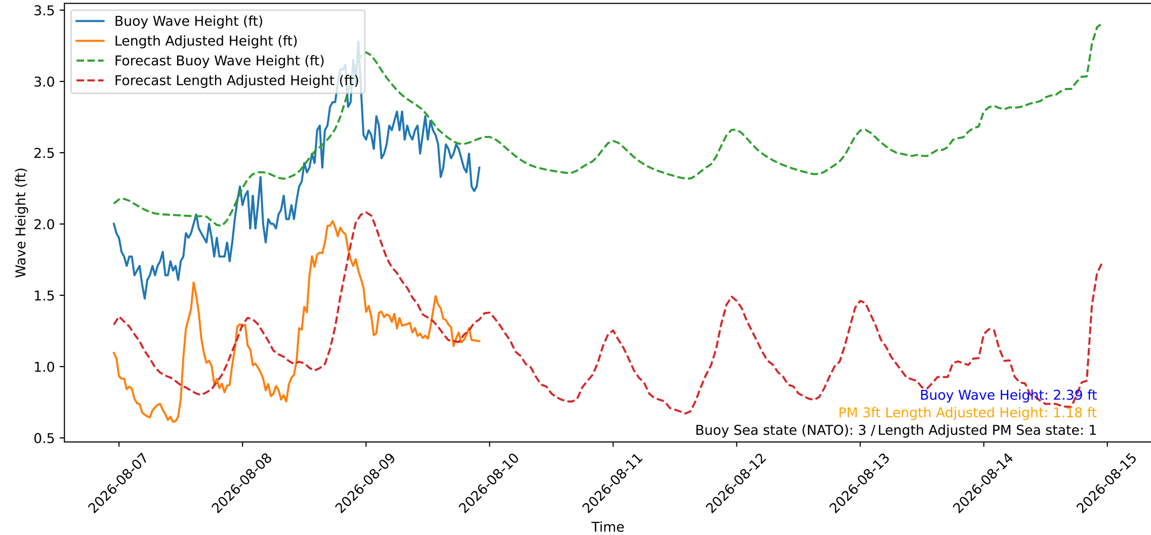
Wave Heights over Time for Red Beach at 2026-08-09 22:50:48
