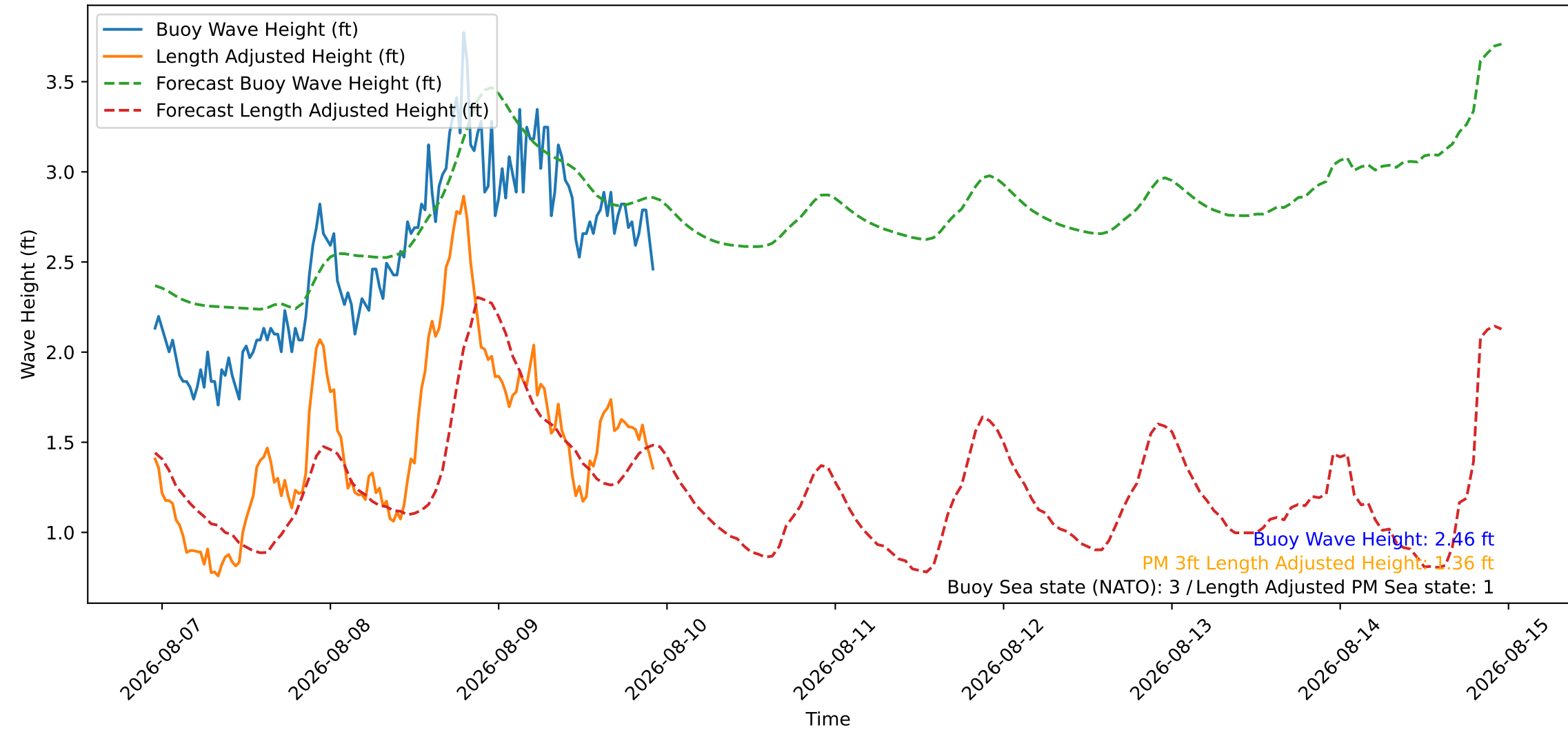
Wave Heights over Time for Green Beach at 2026-08-09 22:51:10
