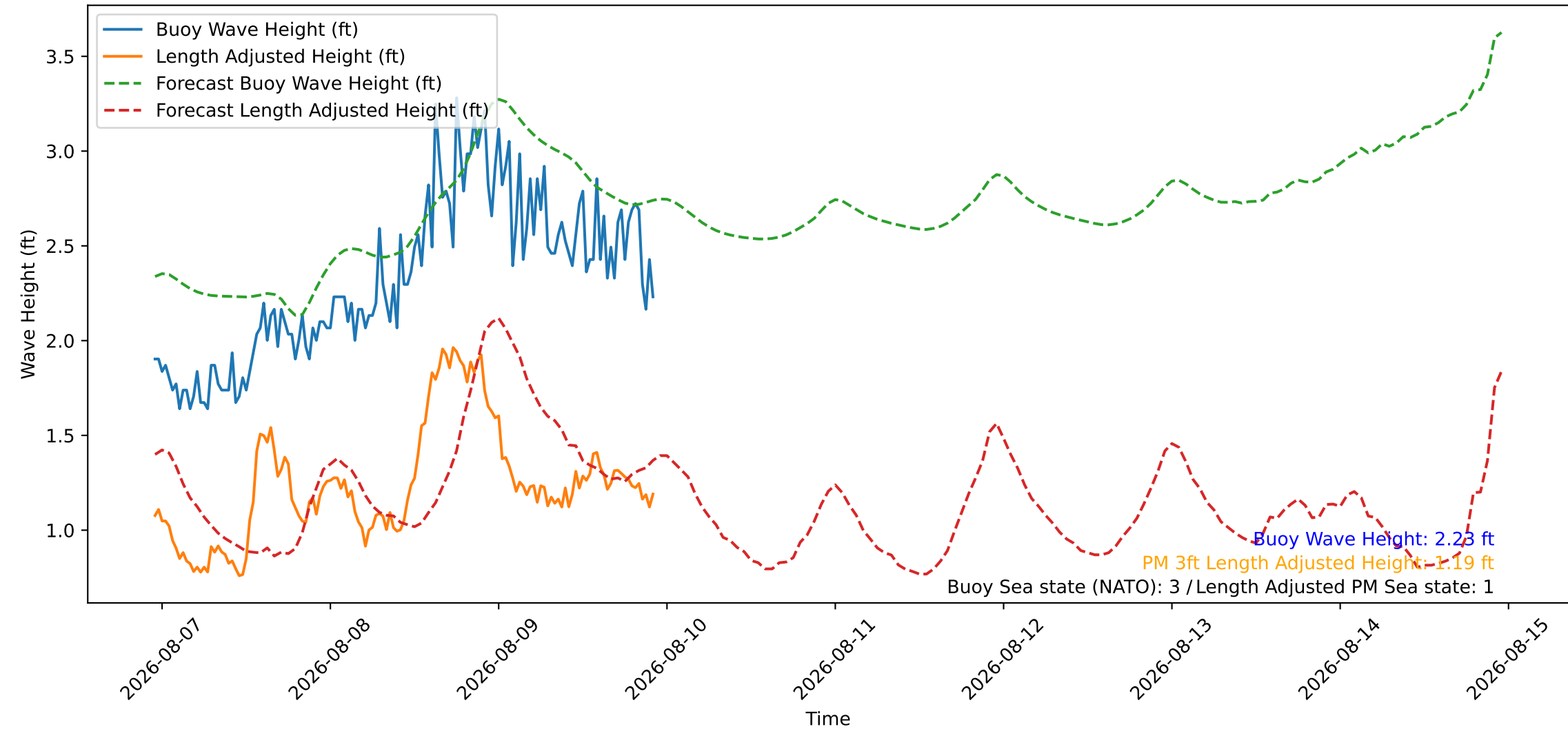
Wave Heights over Time for Oceanside Harbor at 2026-08-09 22:50:27
