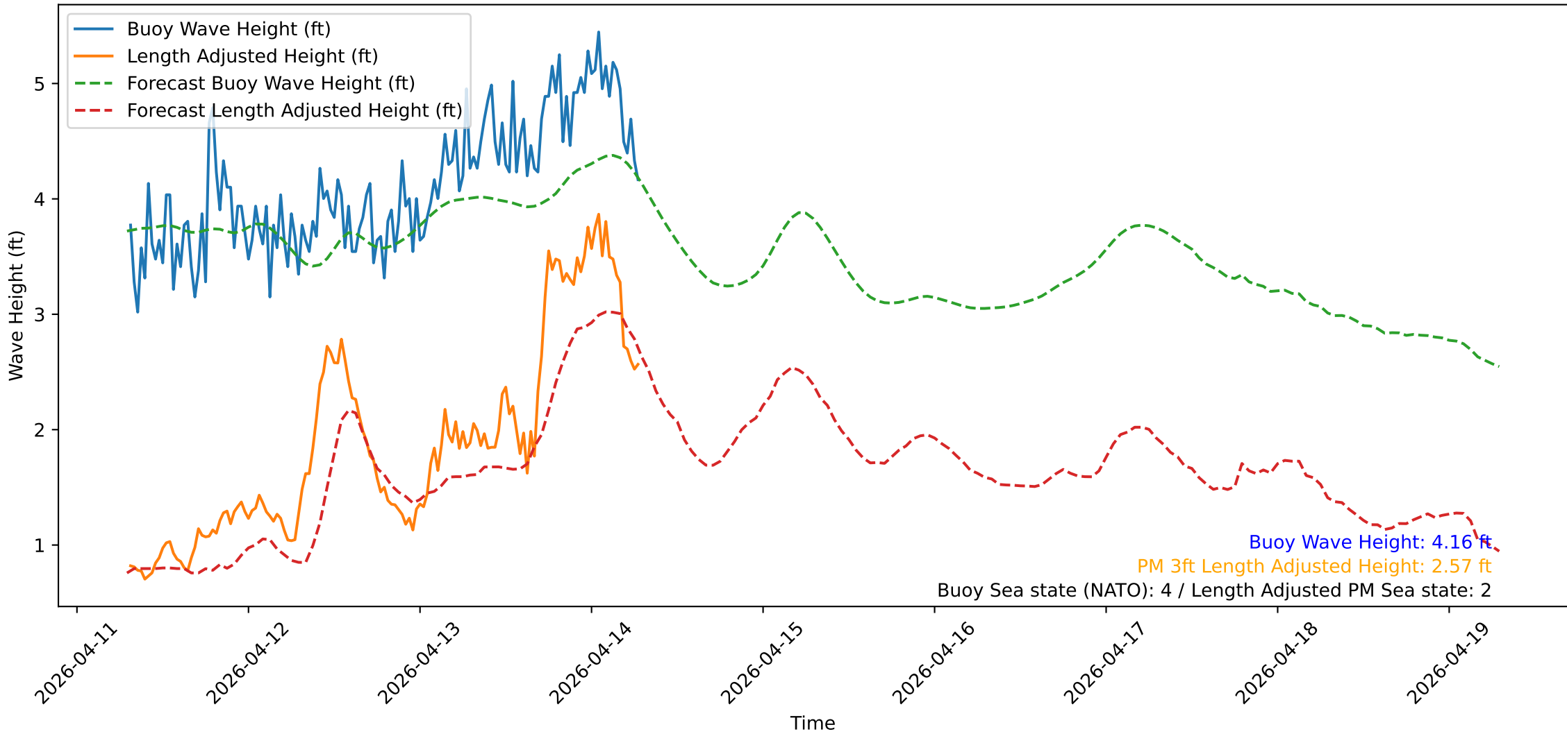
Wave Heights over Time for Oceanside Harbor at 2026-04-14 07:20:31
