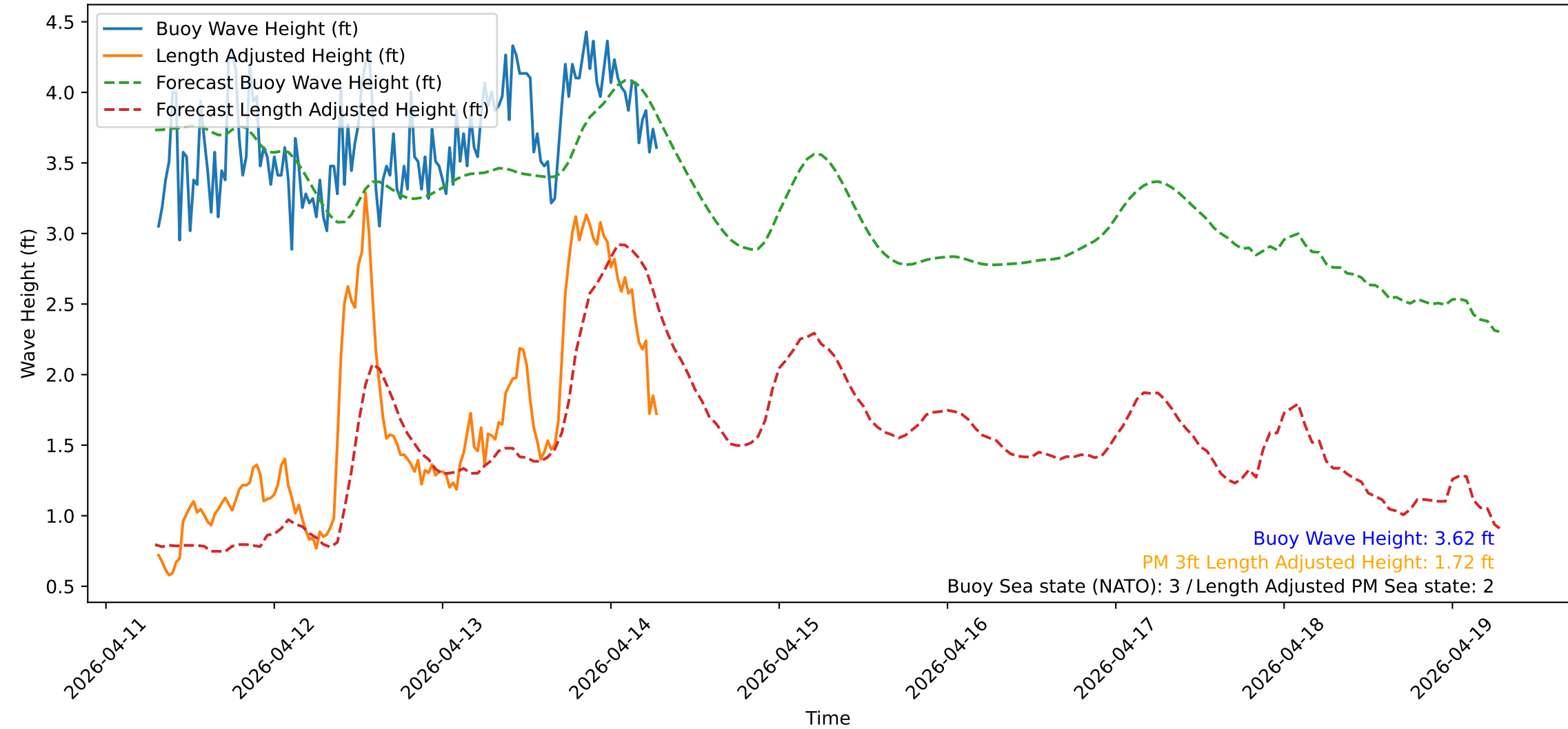
Wave Heights over Time for Red Beach at 2026-04-14 07:20:51
