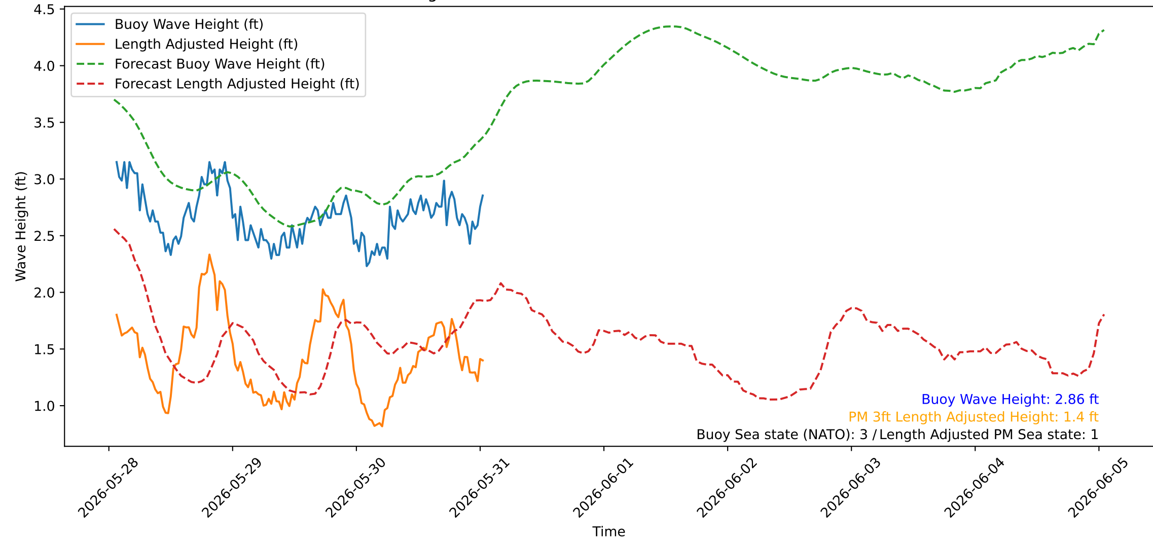
Wave Heights over Time for Red Beach at 2026-05-31 01:10:44
