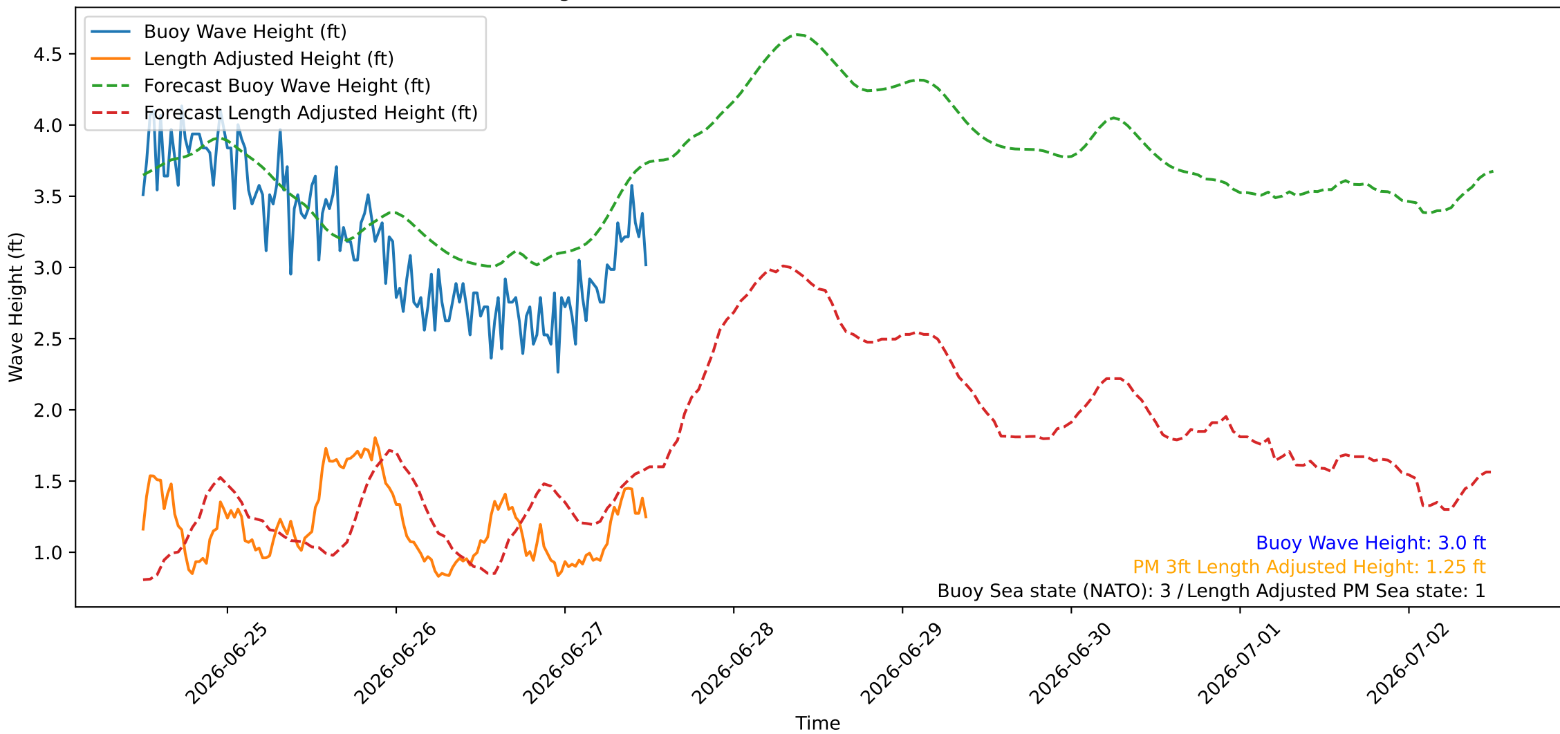
Wave Heights over Time for Green Beach at 2026-06-27 12:11:07
