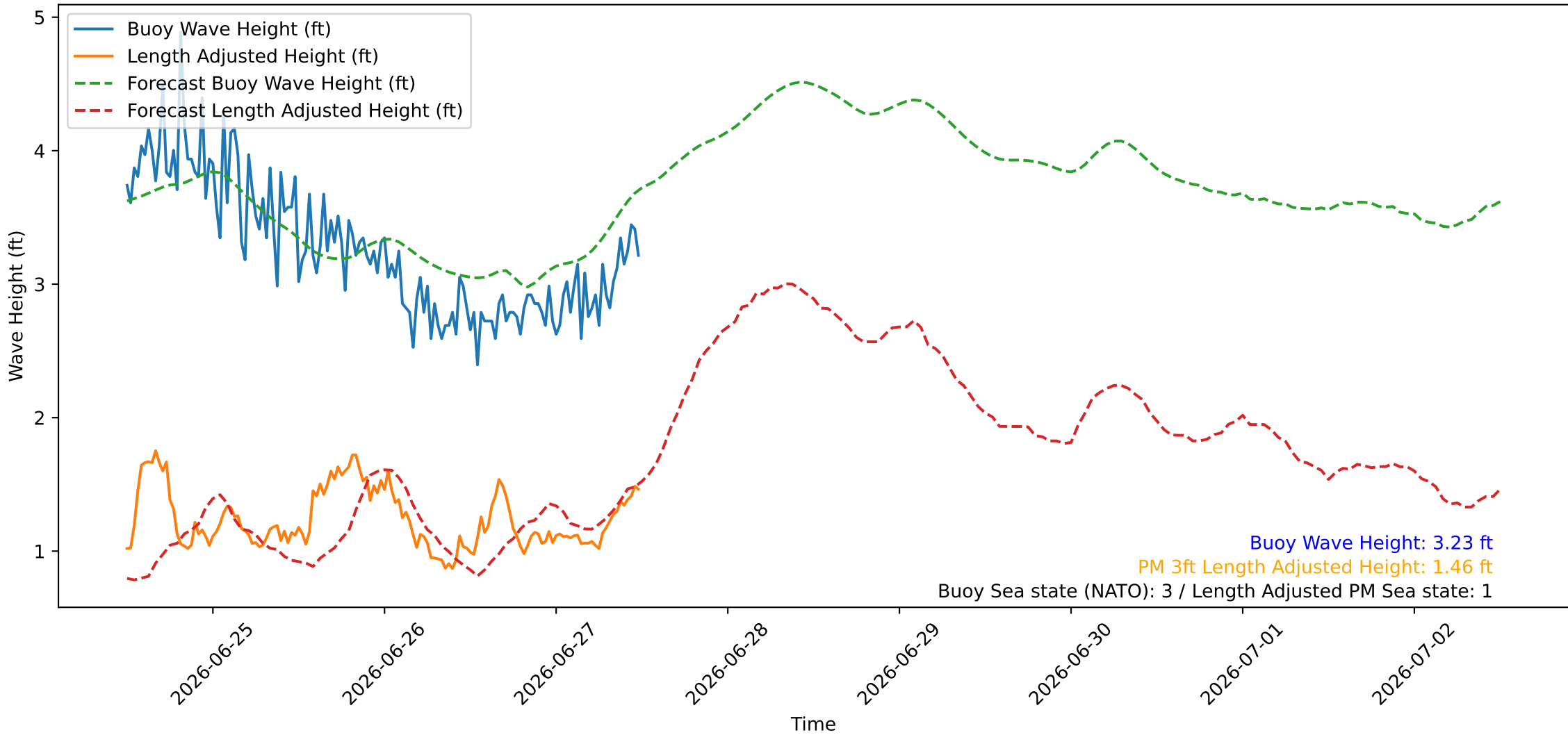
Wave Heights over Time for Oceanside Harbor at 2026-06-27 12:10:26
