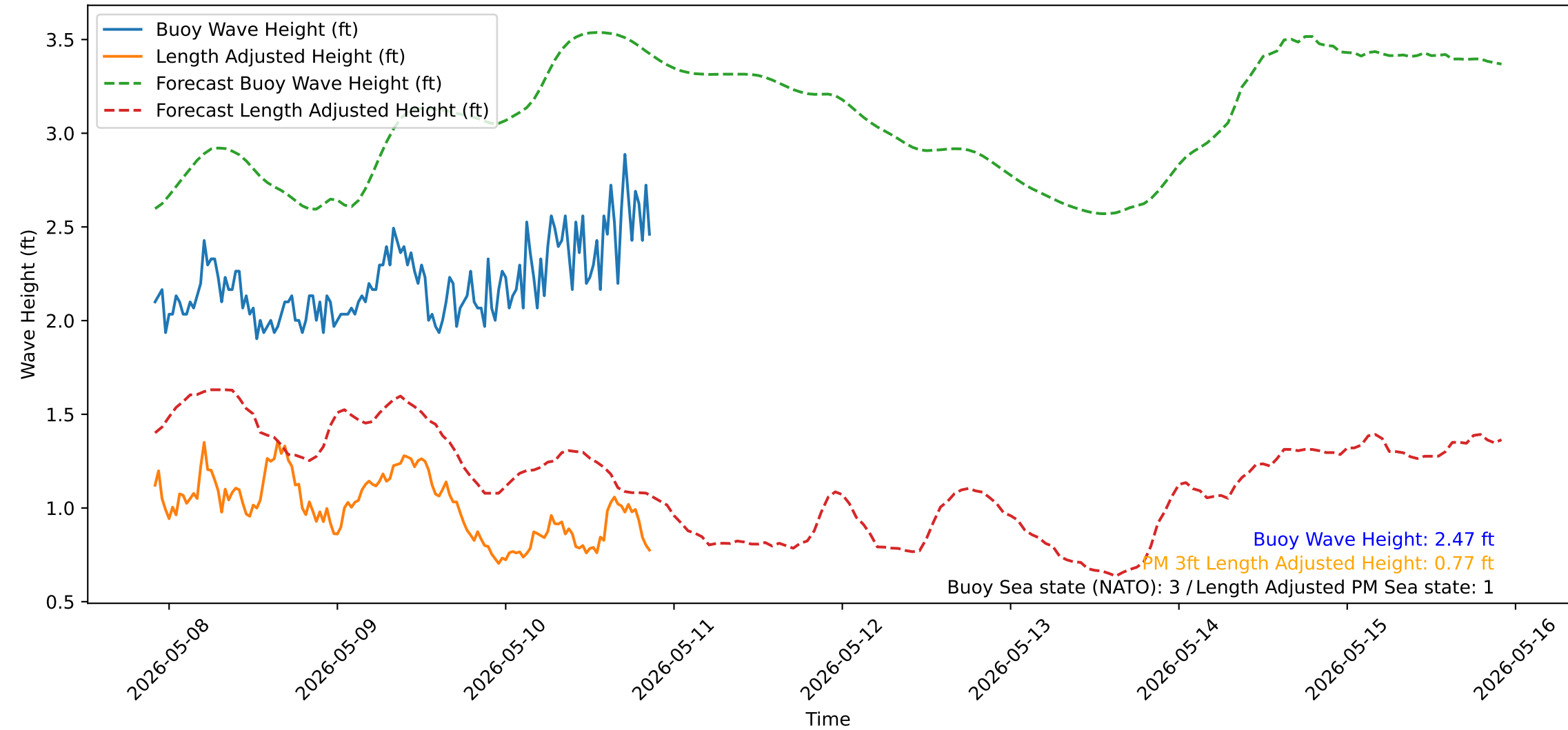
Wave Heights over Time for Red Beach at 2026-05-10 21:40:50
