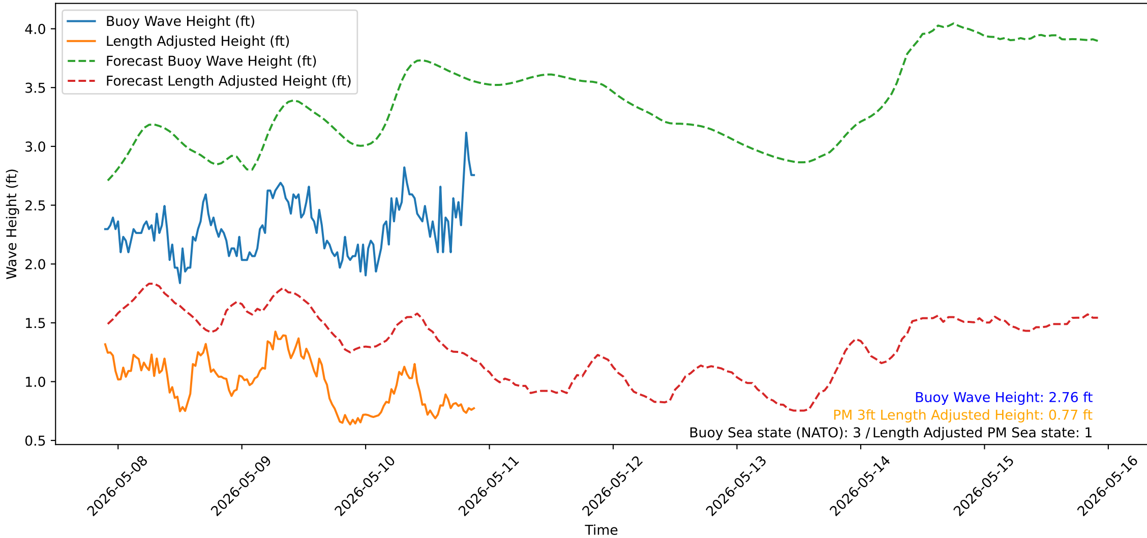
Wave Heights over Time for Green Beach at 2026-05-10 21:41:13
