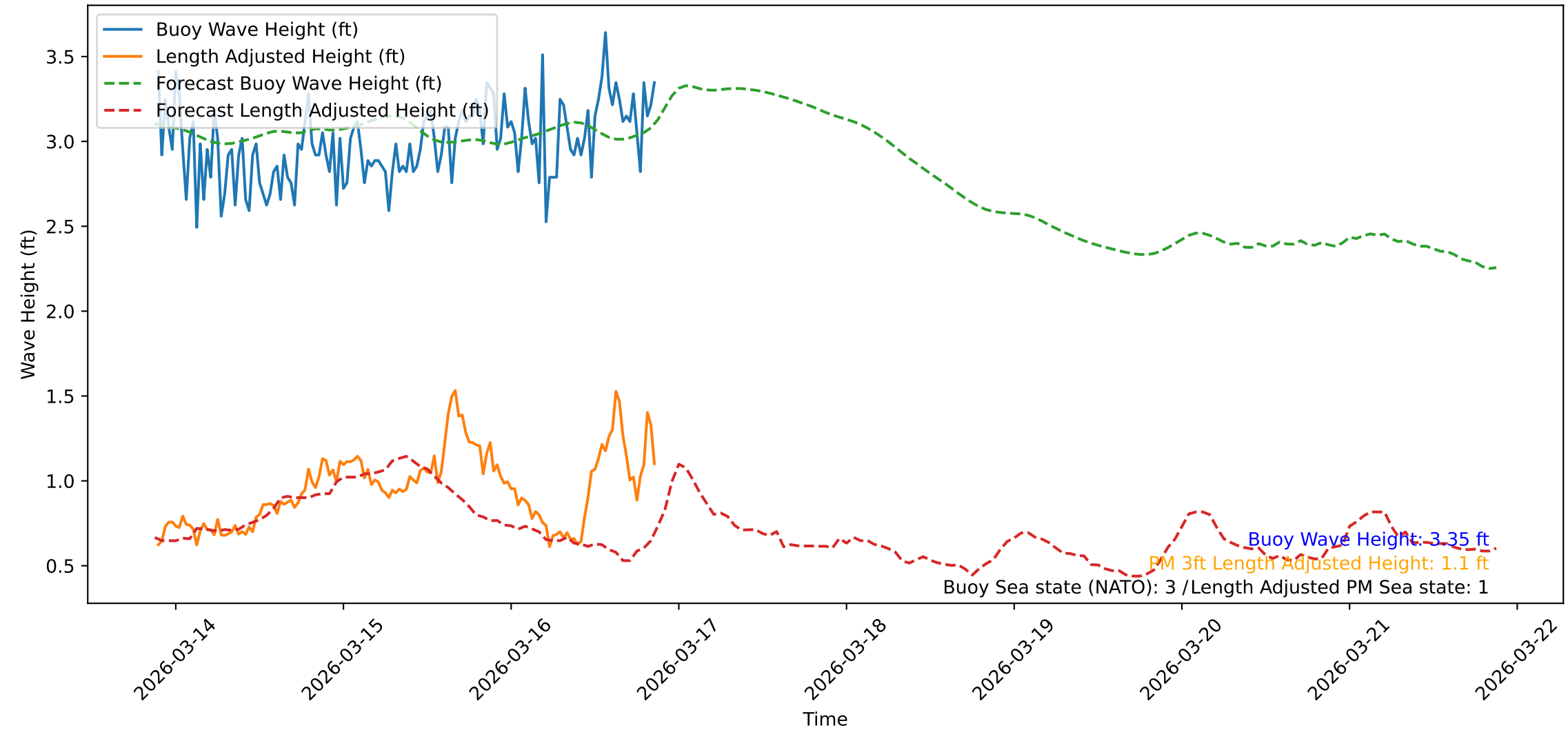
Wave Heights over Time for Red Beach at 2026-03-16 21:11:05
