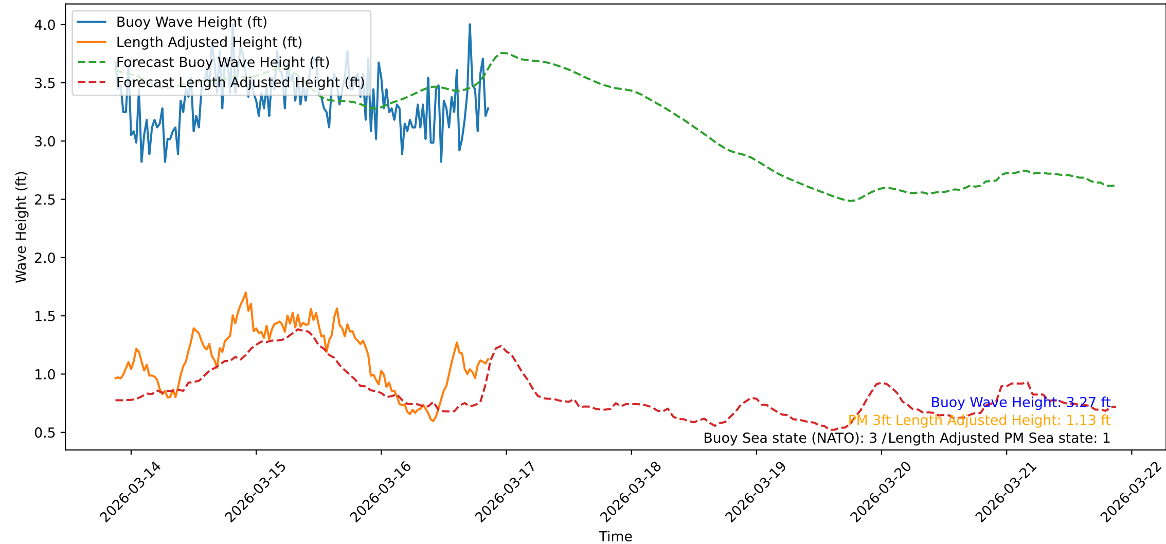
Wave Heights over Time for Green Beach at 2026-03-16 21:11:38
