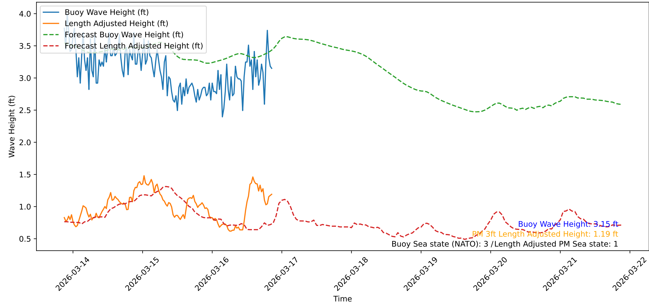
Wave Heights over Time for Oceanside Harbor at 2026-03-16 21:10:43
