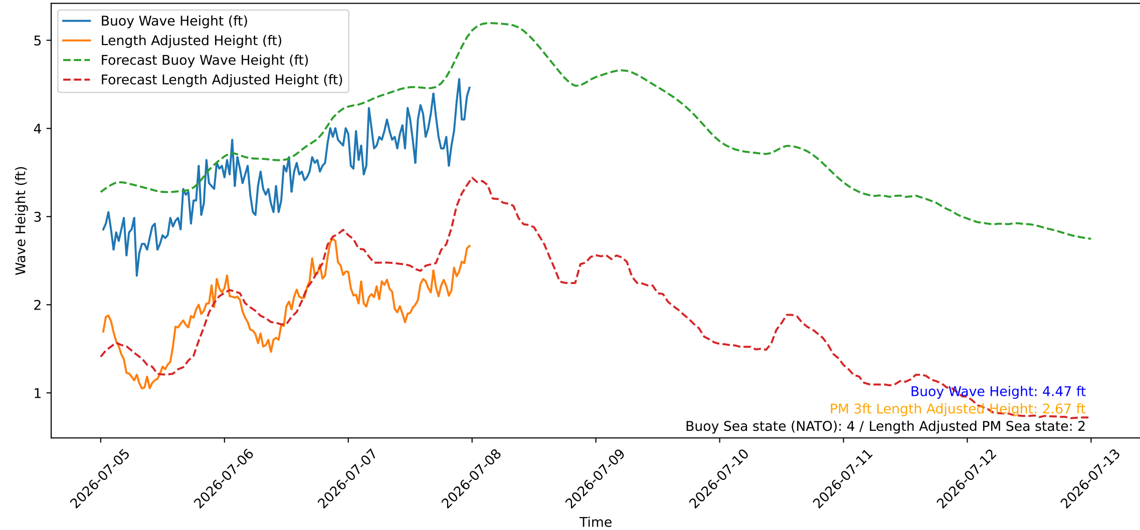
Wave Heights over Time for Oceanside Harbor at 2026-07-08 00:20:26
