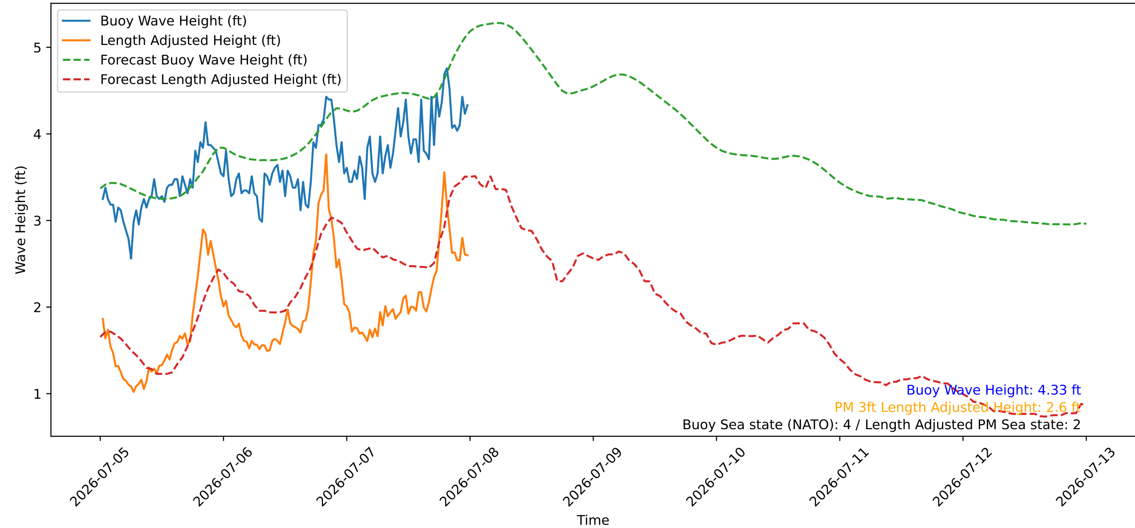
Wave Heights over Time for Green Beach at 2026-07-08 00:21:09
