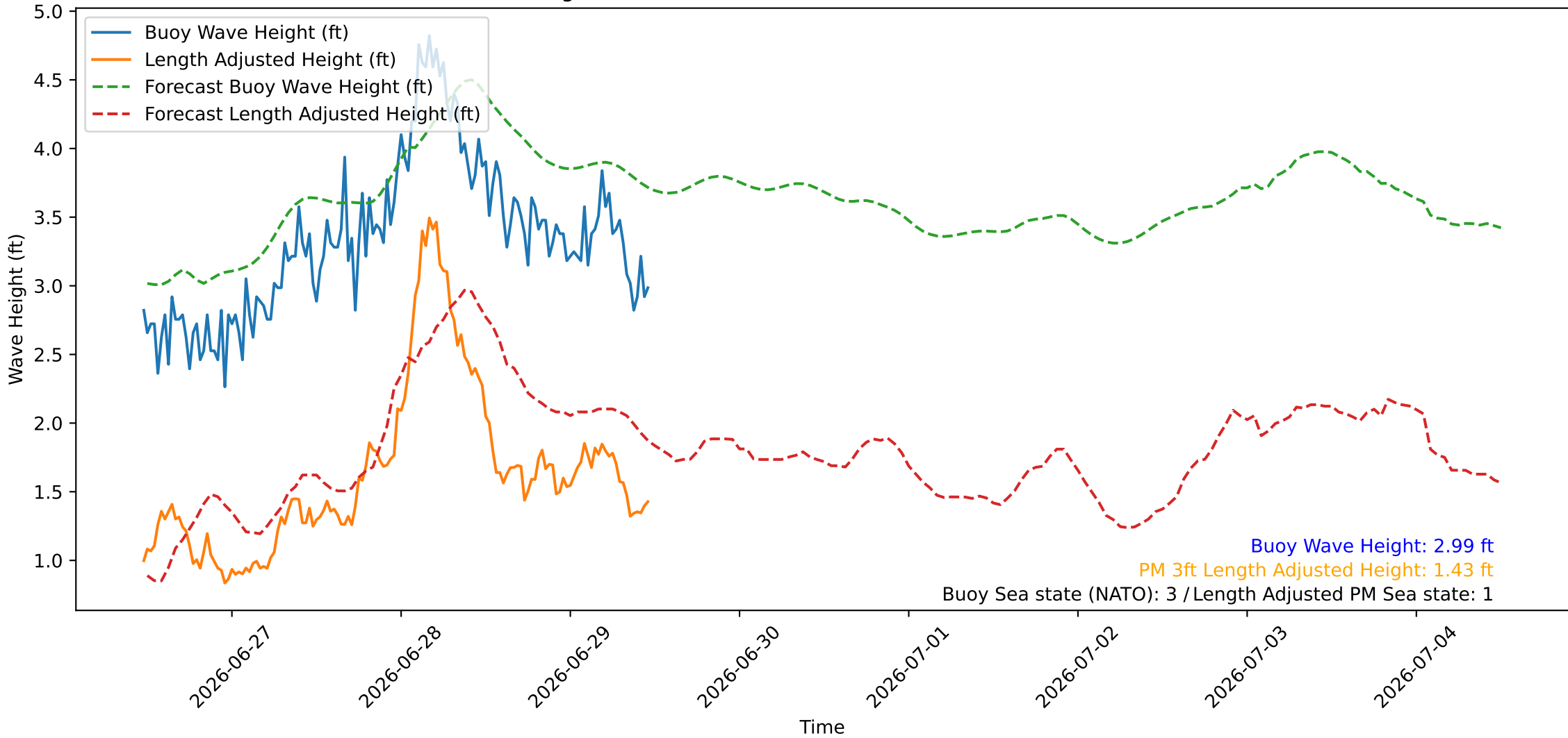
Wave Heights over Time for Green Beach at 2026-06-29 11:41:08
