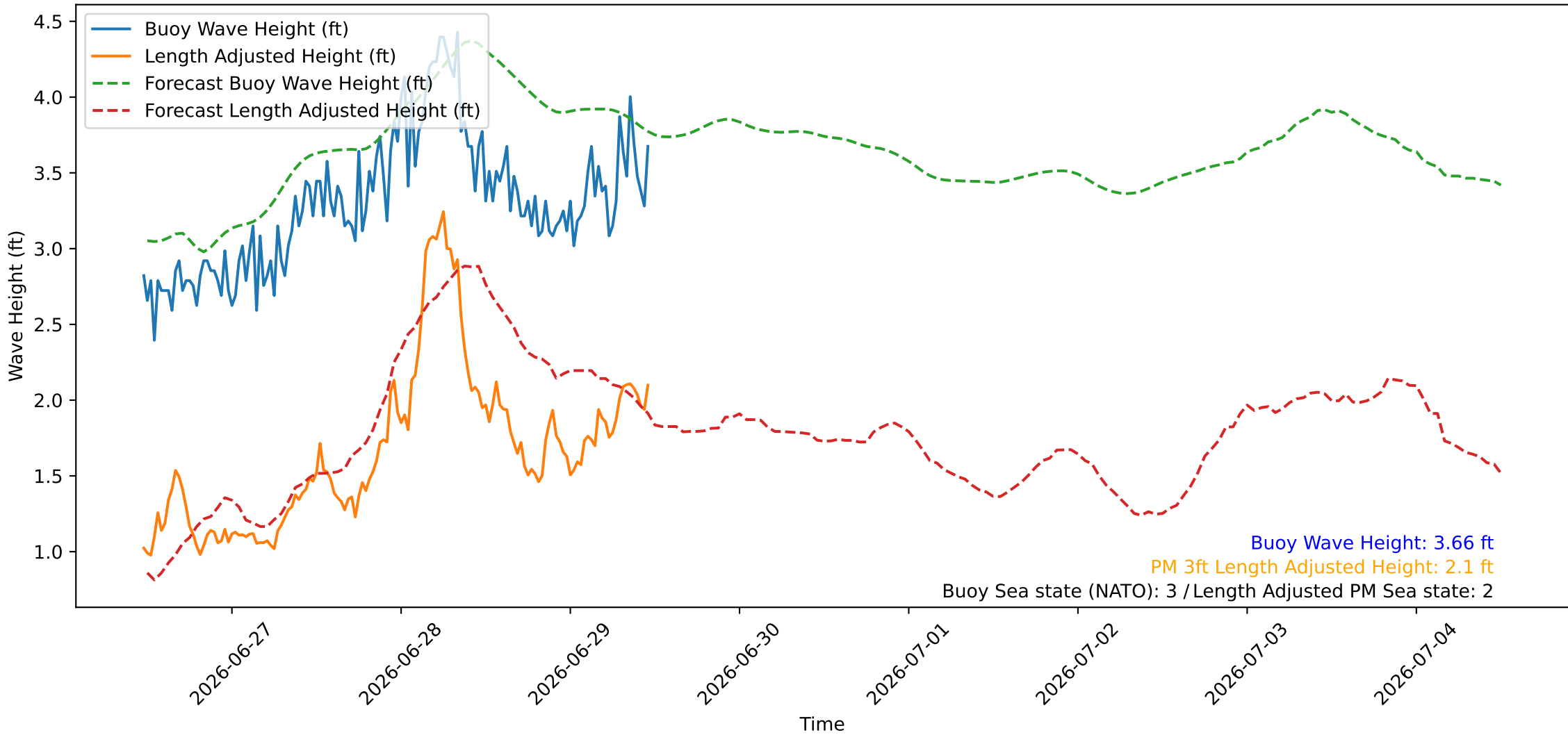
Wave Heights over Time for Oceanside Harbor at 2026-06-29 11:40:26
