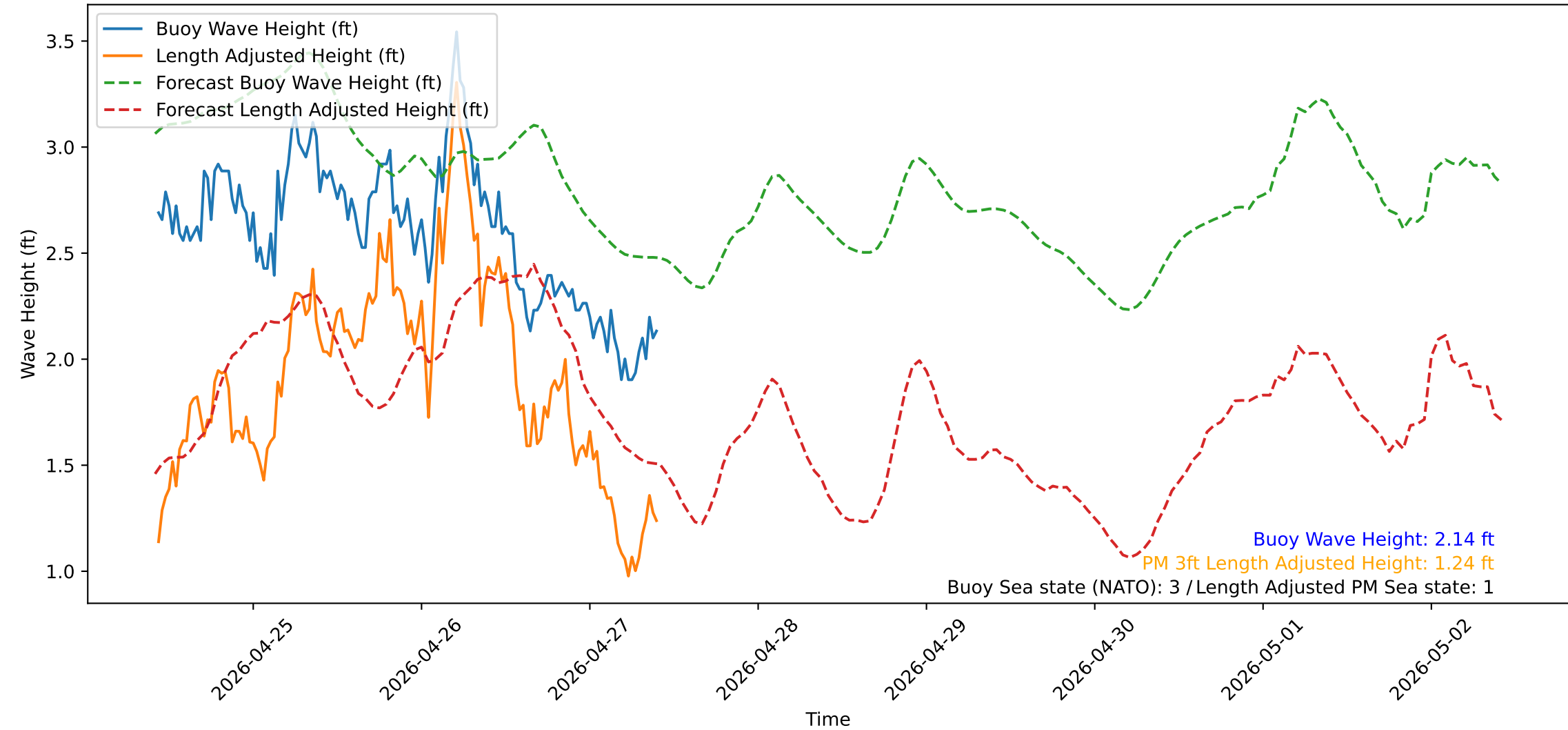
Wave Heights over Time for Red Beach at 2026-04-27 10:10:50
