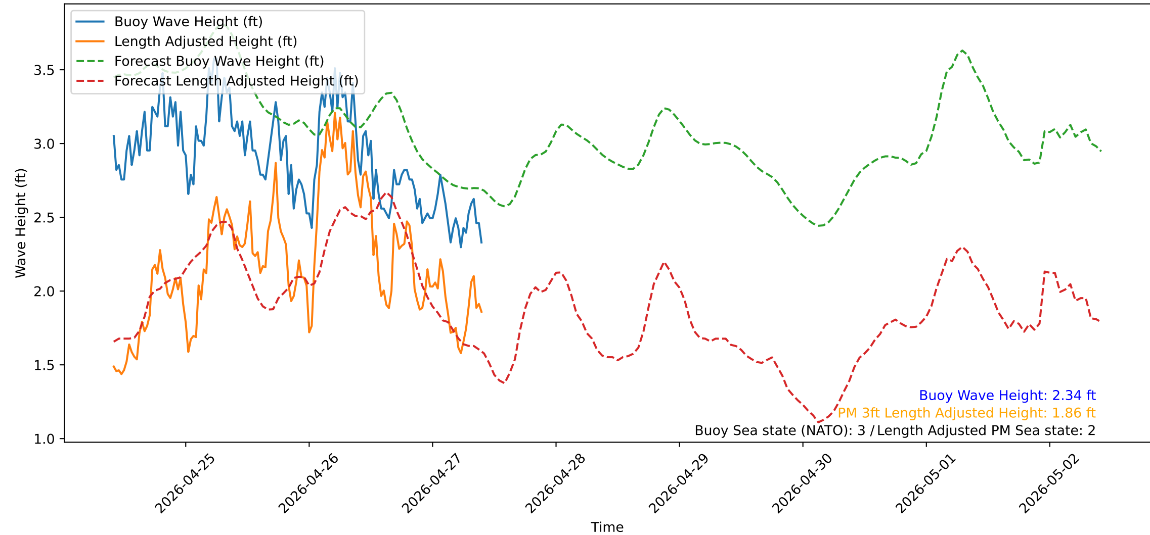
Wave Heights over Time for Green Beach at 2026-04-27 10:11:13
