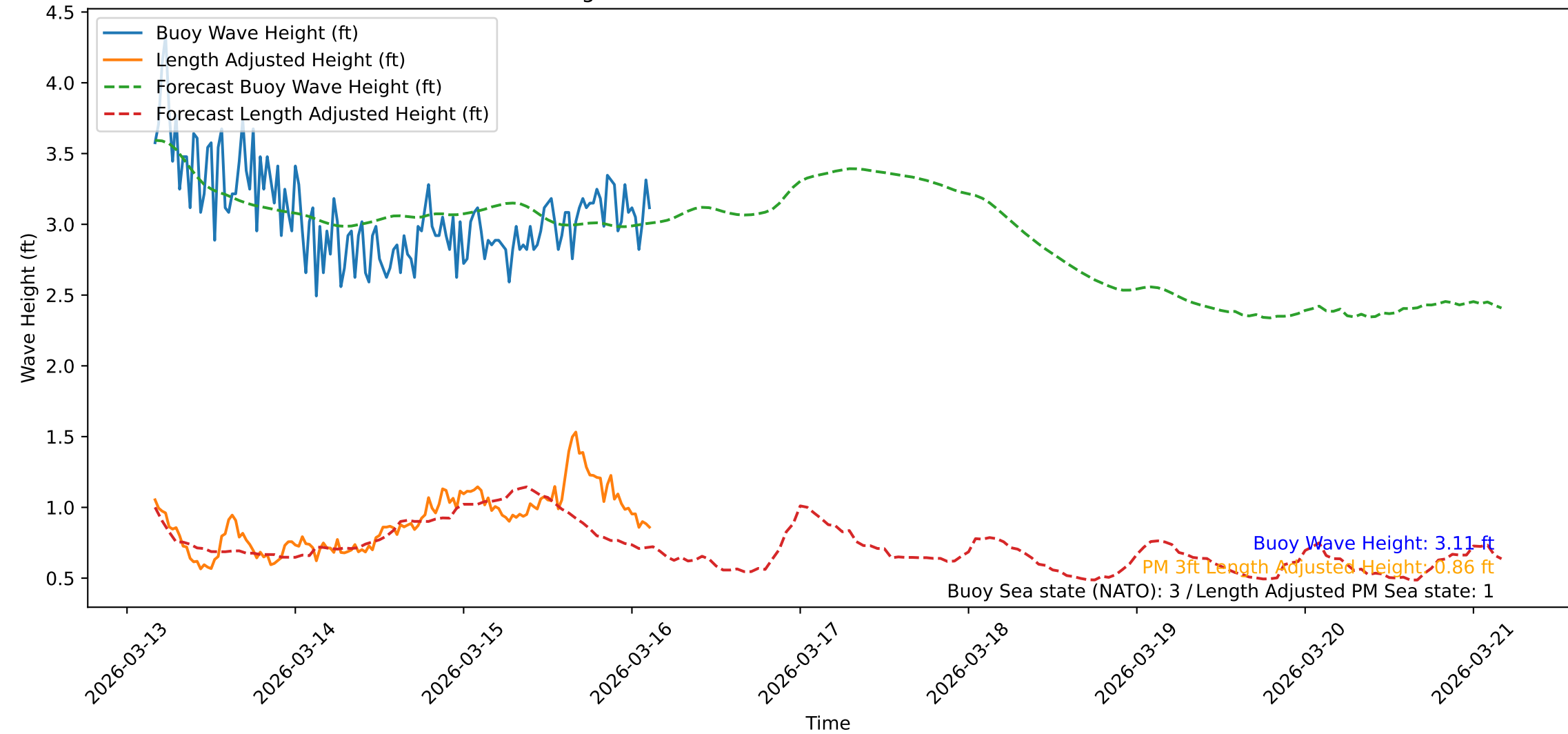
Wave Heights over Time for Red Beach at 2026-03-16 03:31:08
