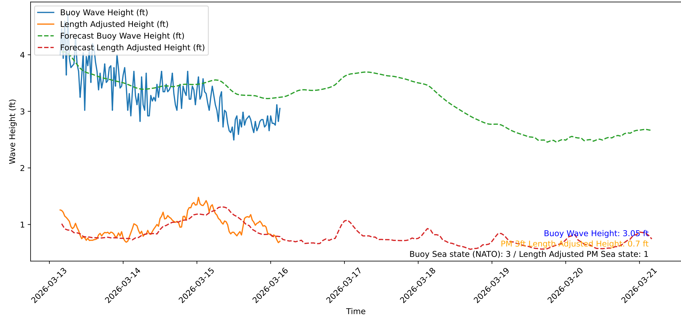
Wave Heights over Time for Oceanside Harbor at 2026-03-16 03:30:46
