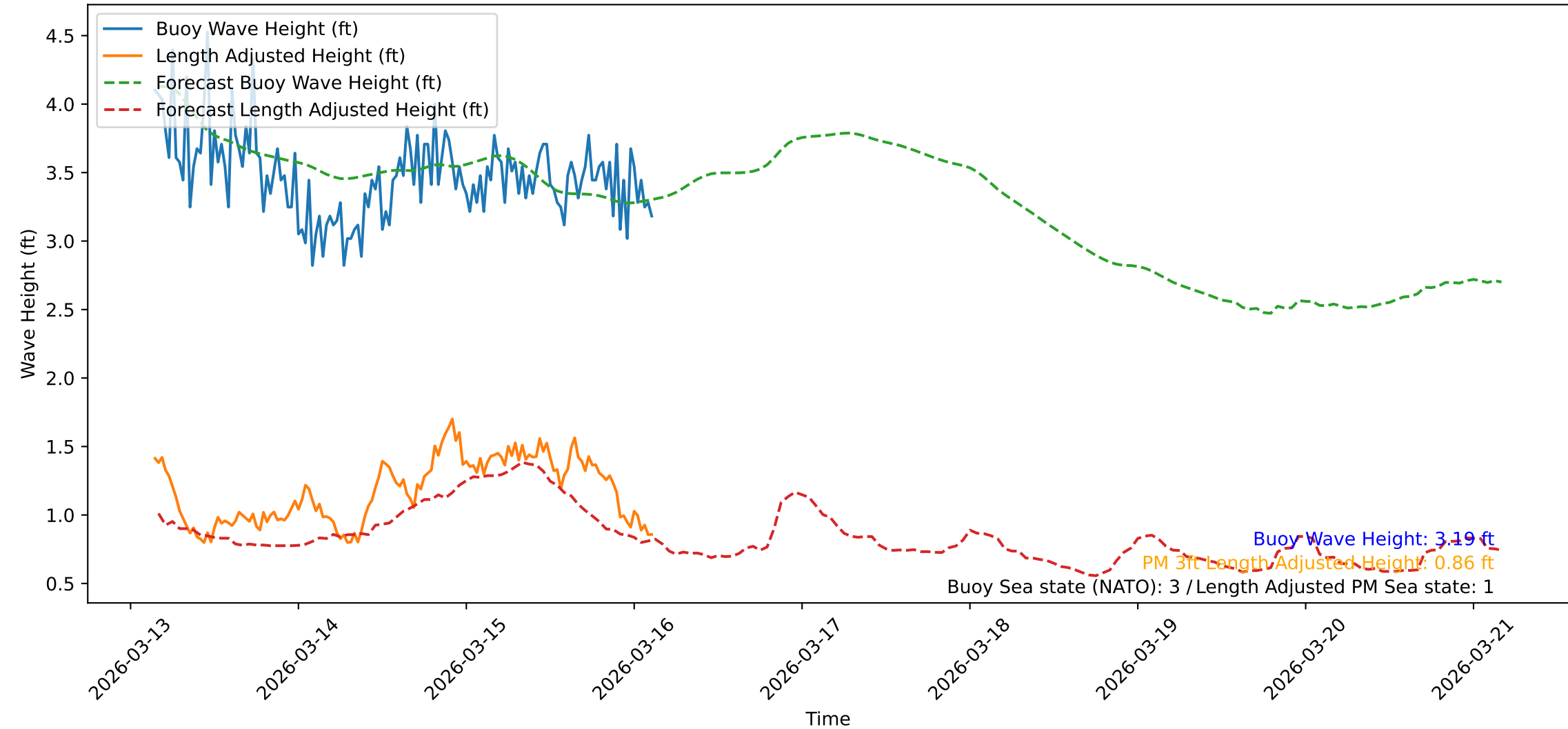
Wave Heights over Time for Green Beach at 2026-03-16 03:31:41
