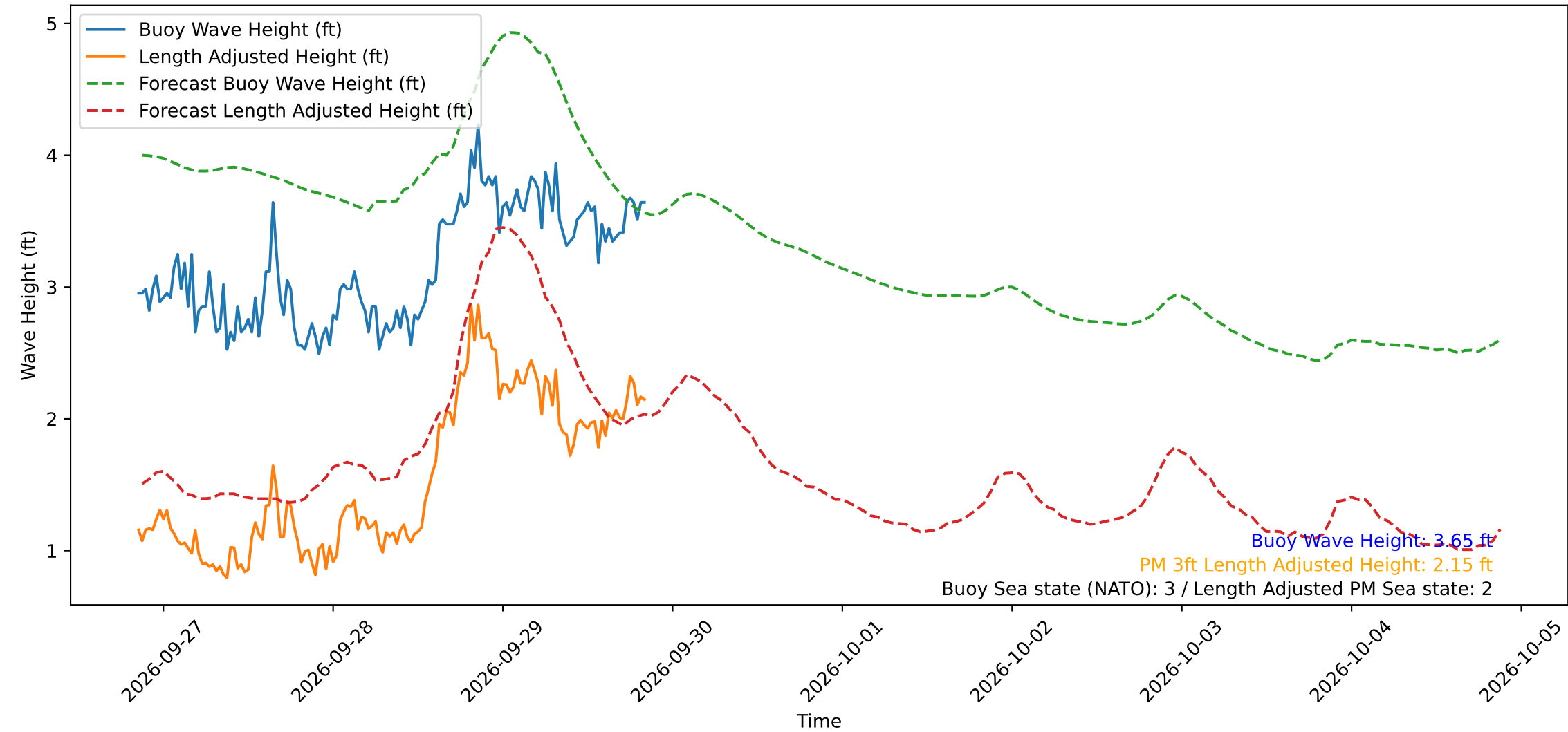
Wave Heights over Time for Oceanside Harbor at 2026-09-29 20:40:29
