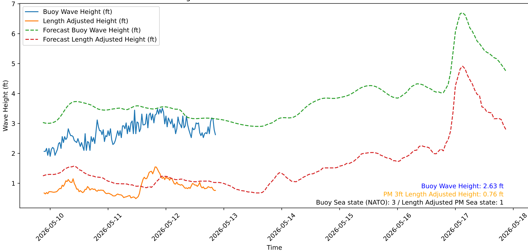
Wave Heights over Time for Green Beach at 2026-05-12 21:21:15
