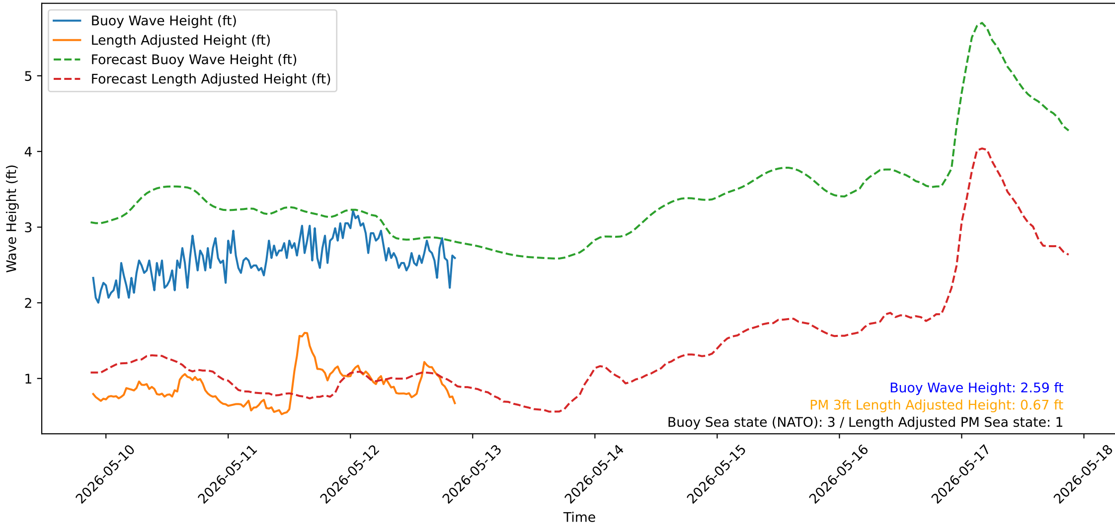
Wave Heights over Time for Red Beach at 2026-05-12 21:20:52
