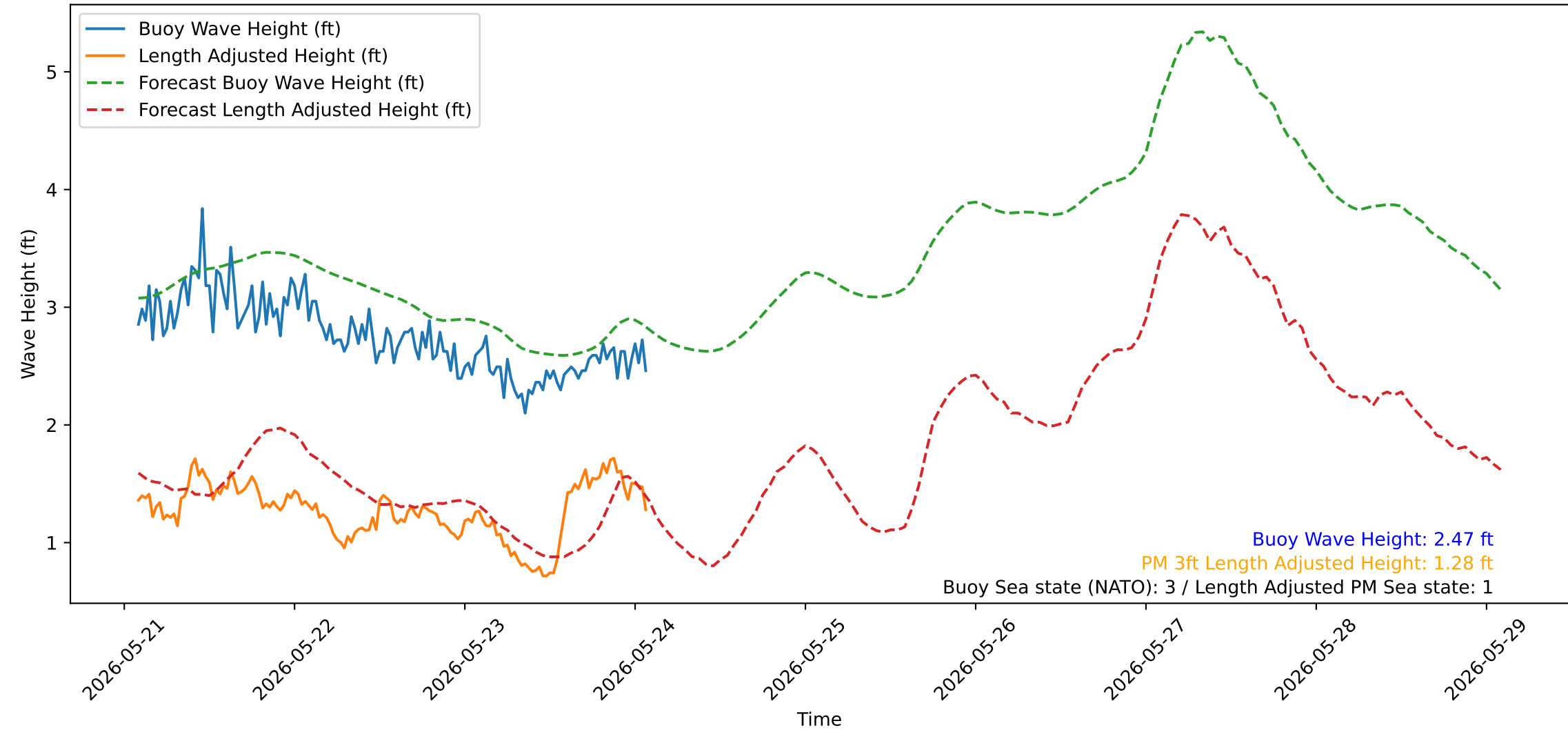
Wave Heights over Time for Oceanside Harbor at 2026-05-24 02:10:31
