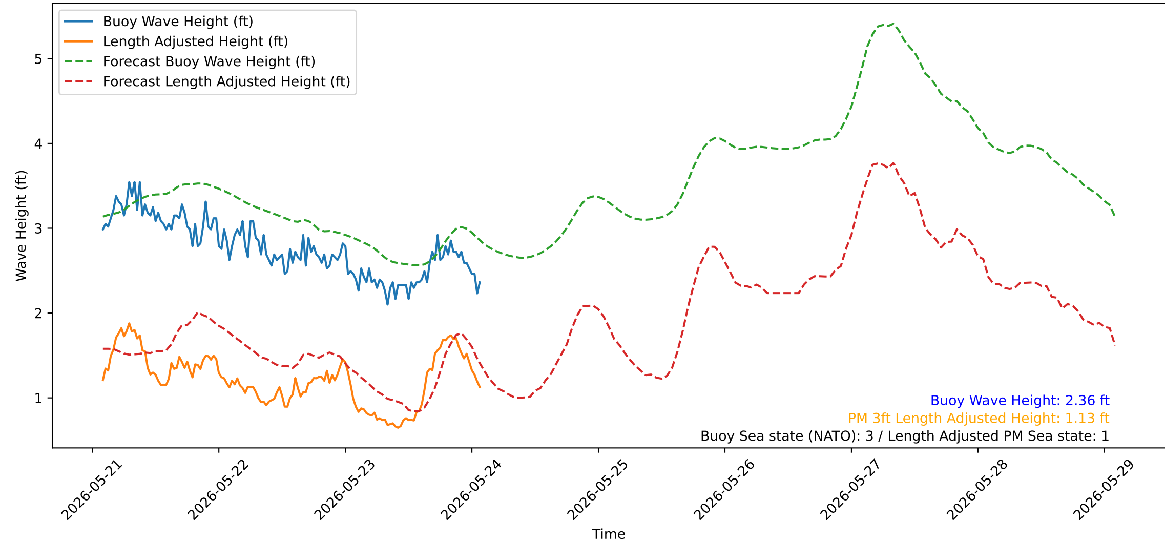
Wave Heights over Time for Green Beach at 2026-05-24 02:11:13
