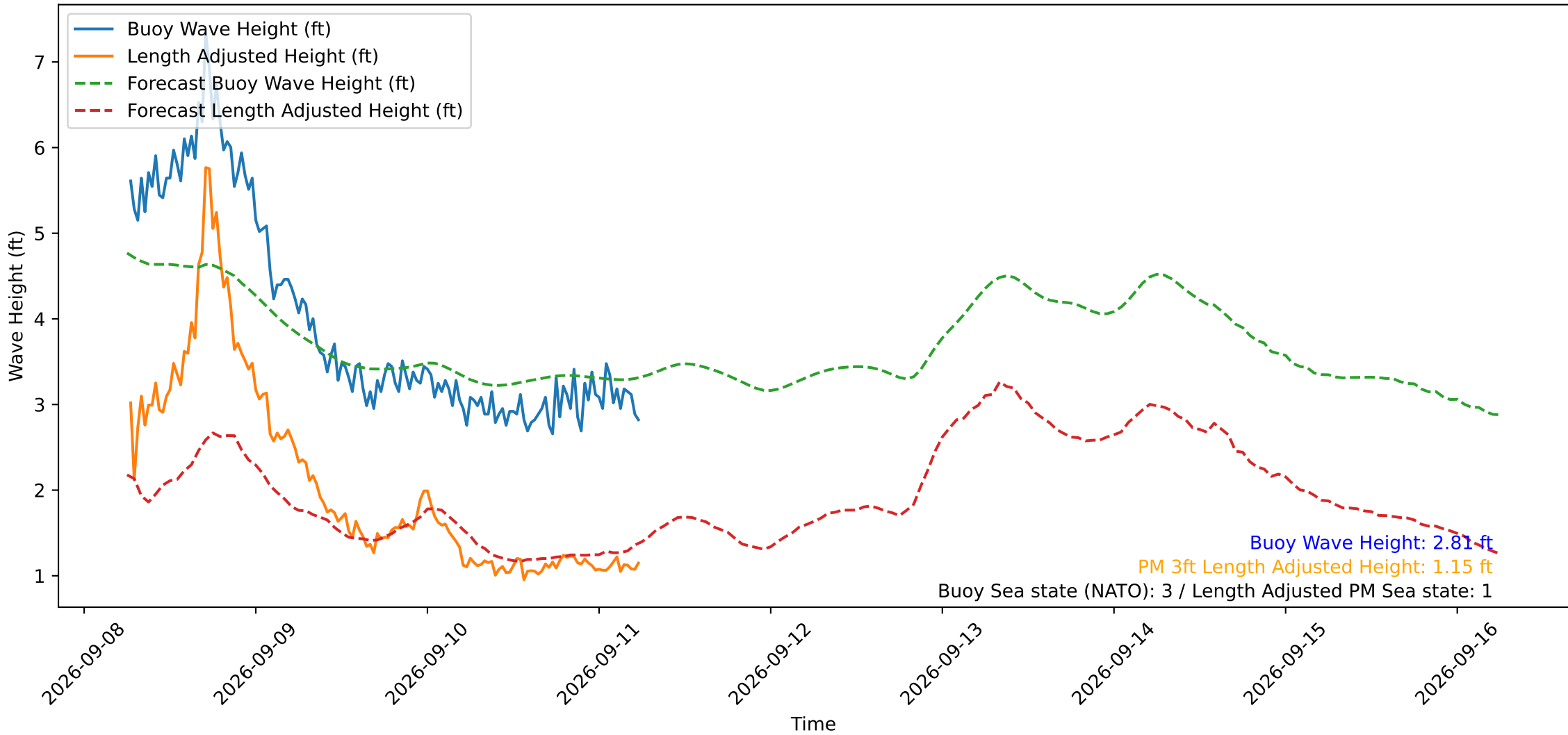
Wave Heights over Time for Oceanside Harbor at 2026-09-11 06:20:30
