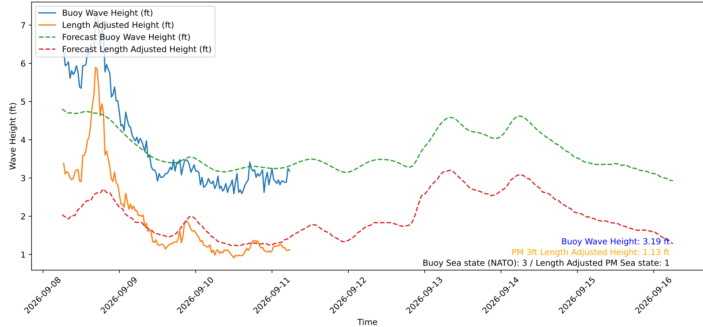
Wave Heights over Time for Green Beach at 2026-09-11 06:21:15
