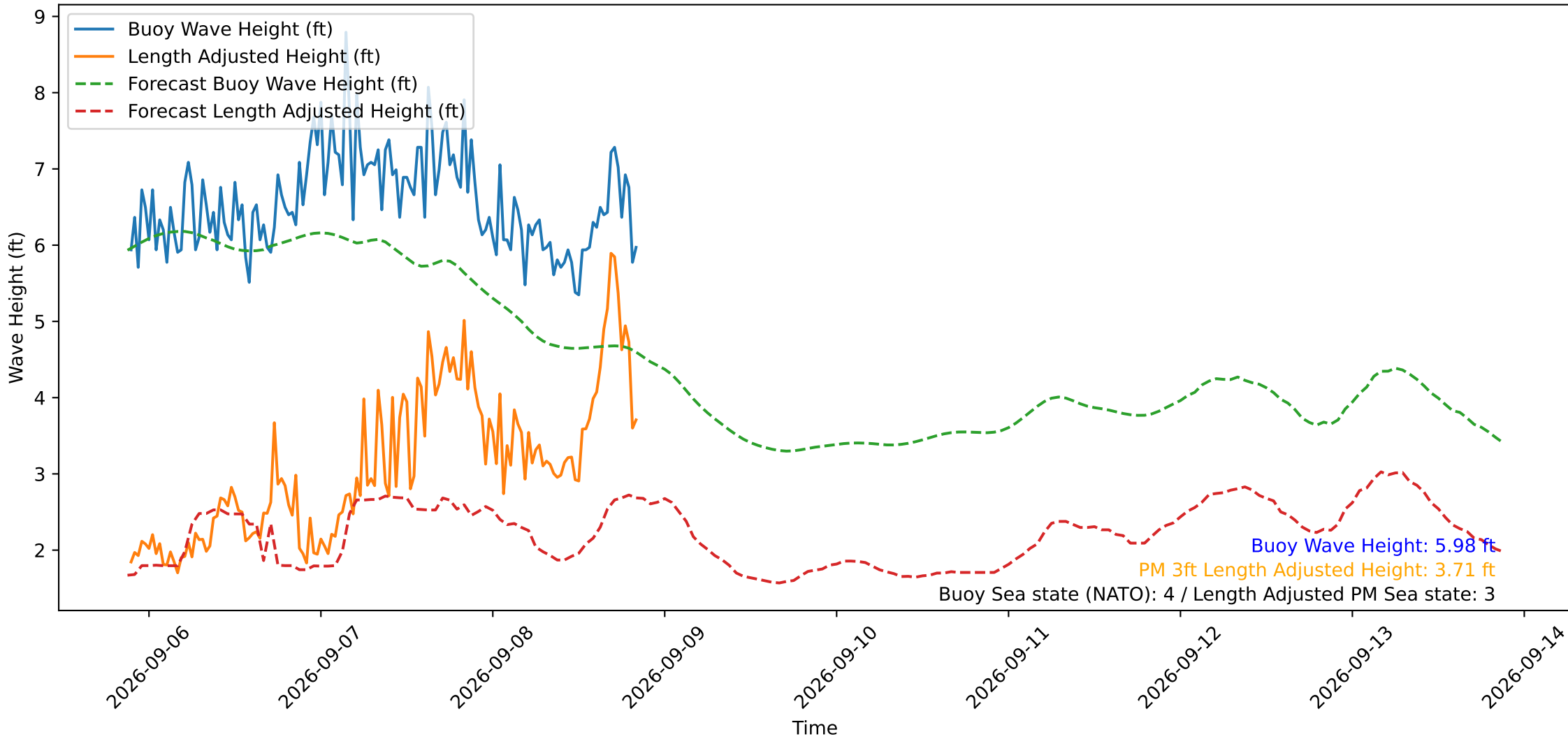
Wave Heights over Time for Green Beach at 2026-09-08 21:01:11
