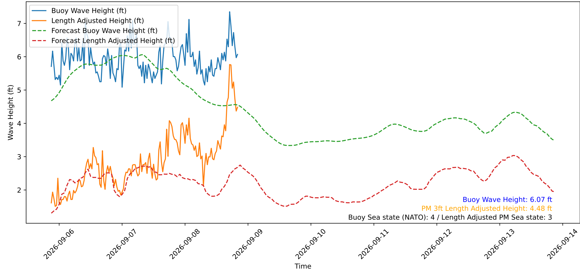
Wave Heights over Time for Oceanside Harbor at 2026-09-08 21:00:30
