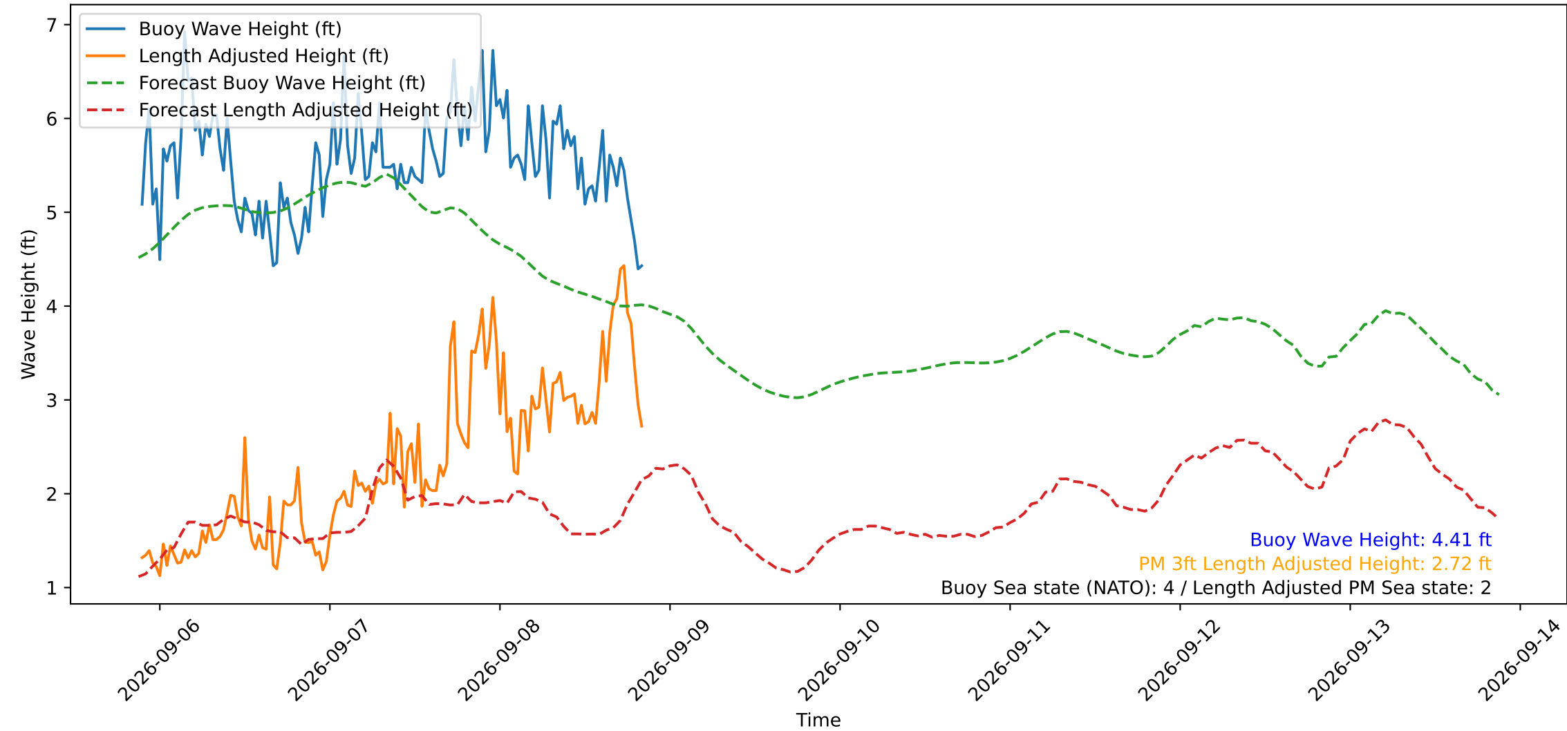
Wave Heights over Time for Red Beach at 2026-09-08 21:00:49
