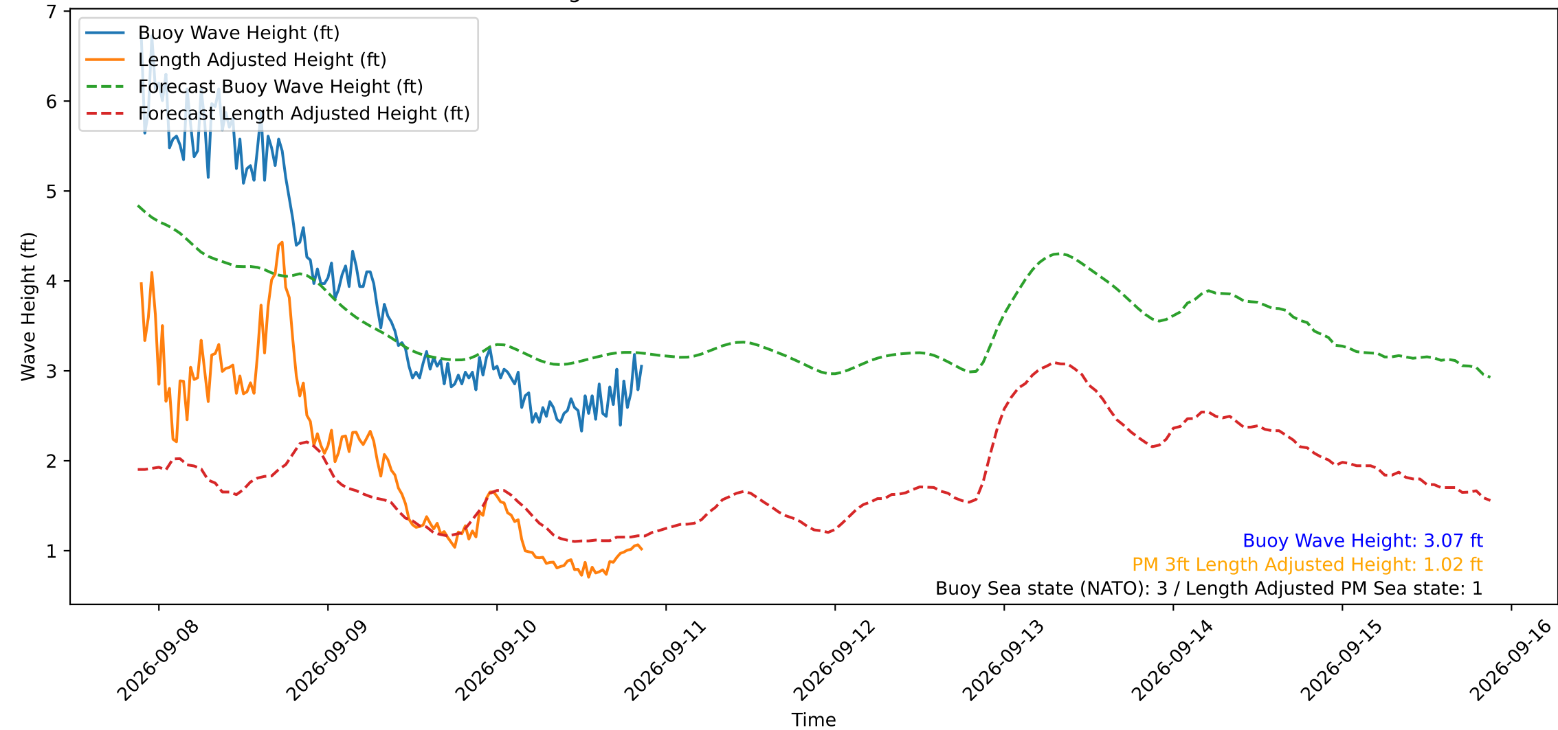
Wave Heights over Time for Red Beach at 2026-09-10 21:20:50
