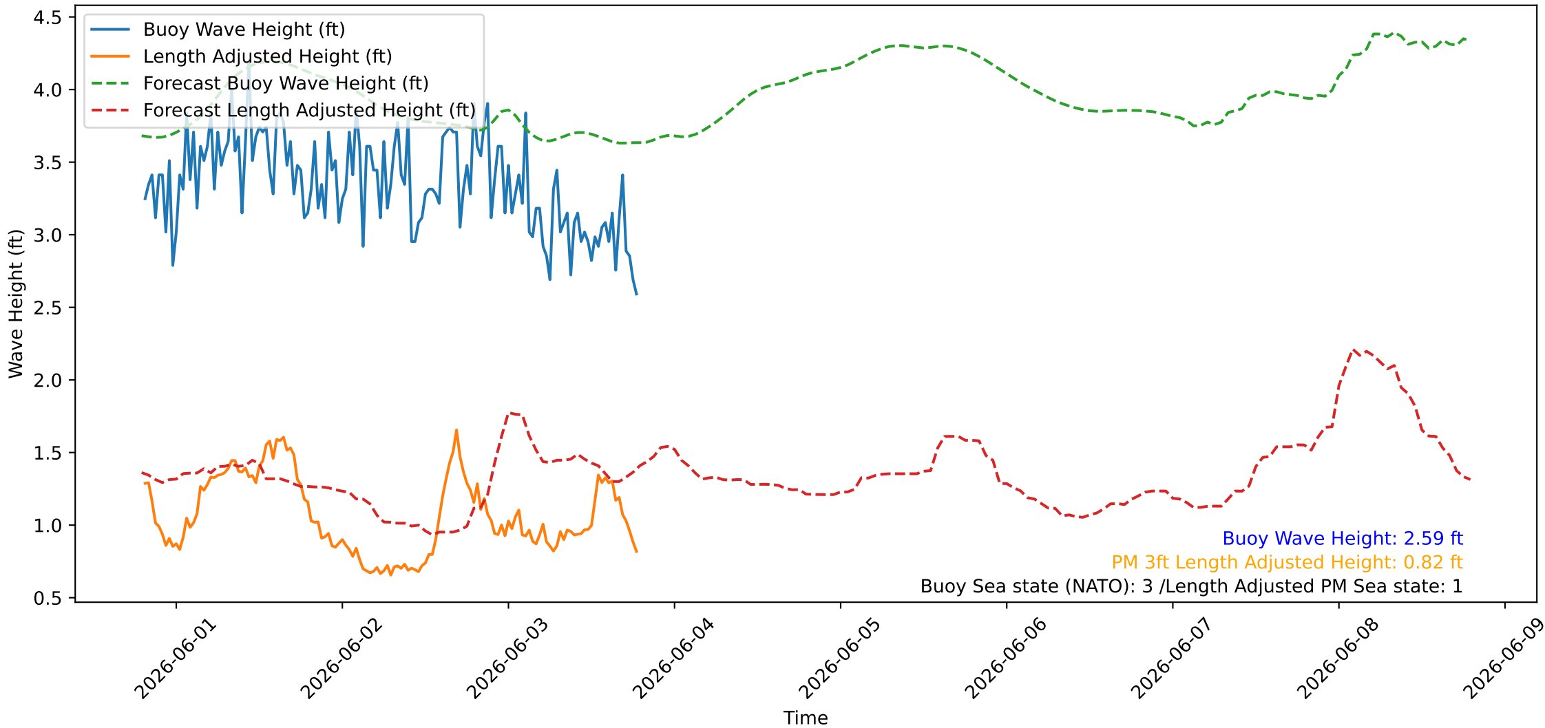
Wave Heights over Time for Red Beach at 2026-06-03 19:20:46
