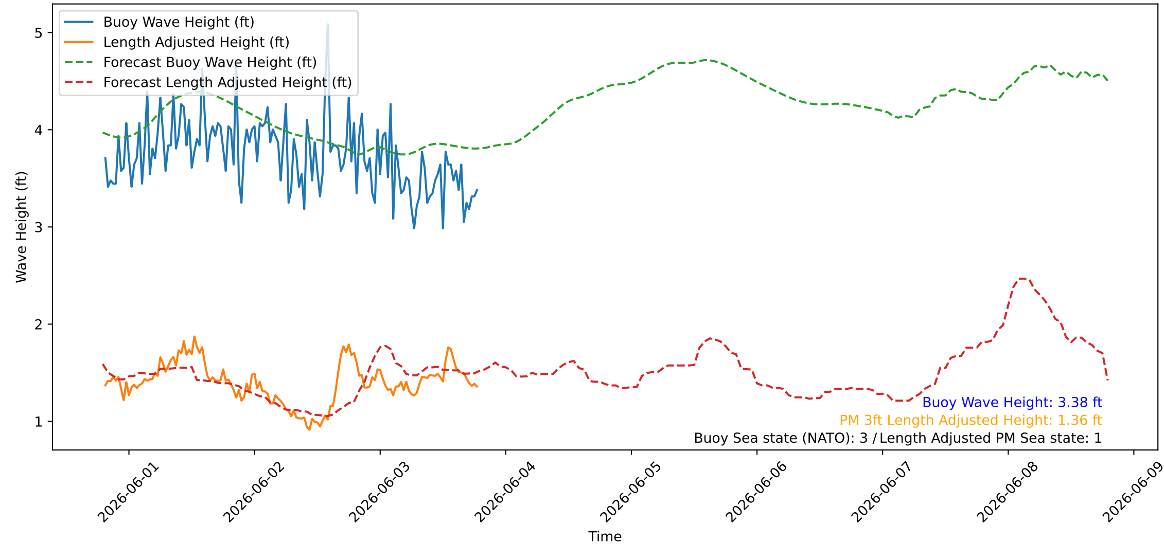
Wave Heights over Time for Oceanside Harbor at 2026-06-03 19:20:26
