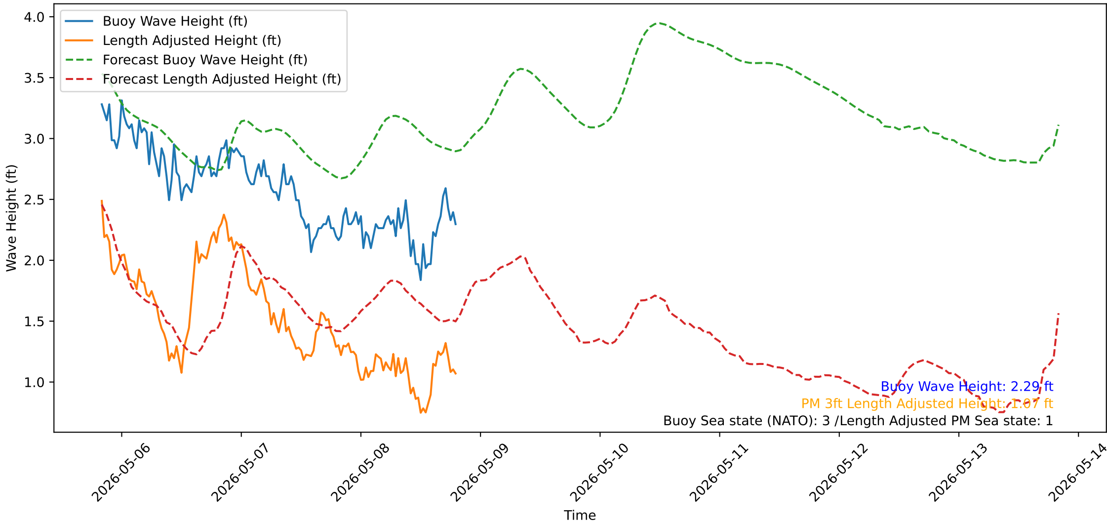
Wave Heights over Time for Green Beach at 2026-05-08 20:01:13
