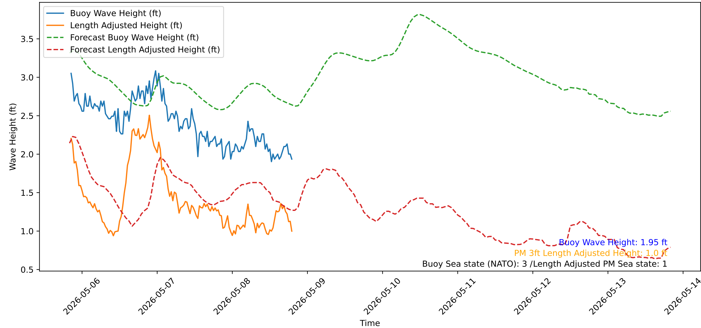
Wave Heights over Time for Red Beach at 2026-05-08 20:00:50
