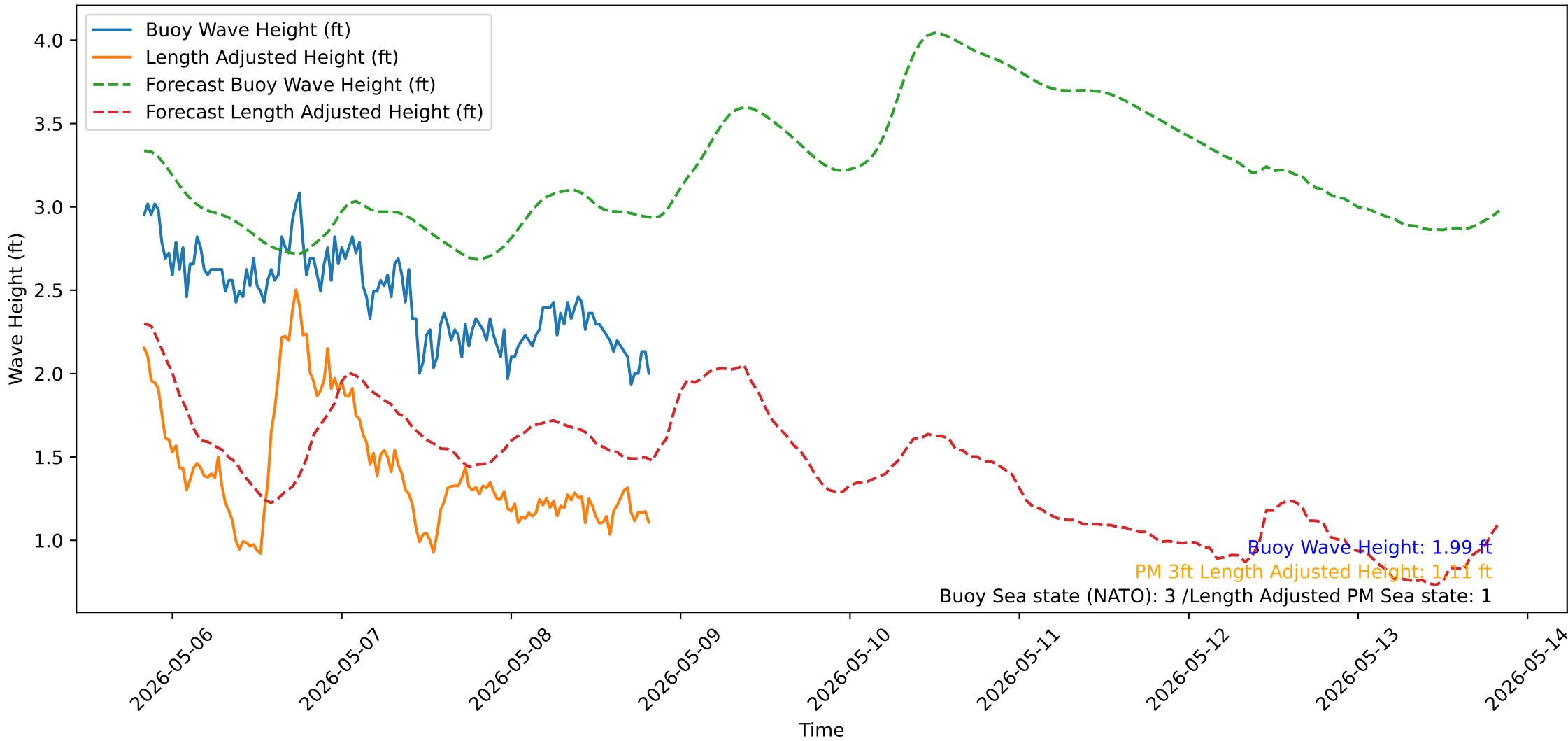
Wave Heights over Time for Oceanside Harbor at 2026-05-08 20:00:31
