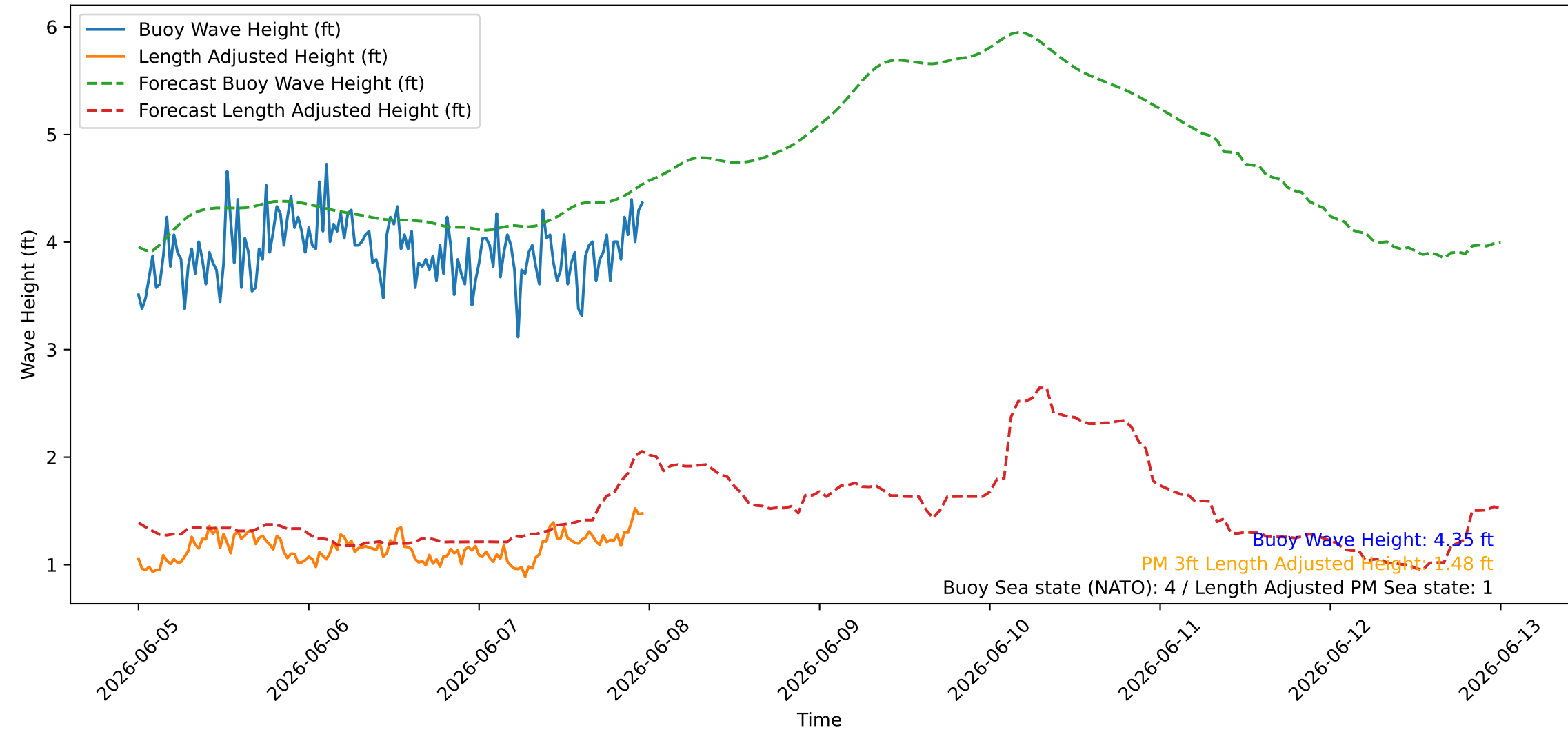
Wave Heights over Time for Green Beach at 2026-06-08 00:01:08
