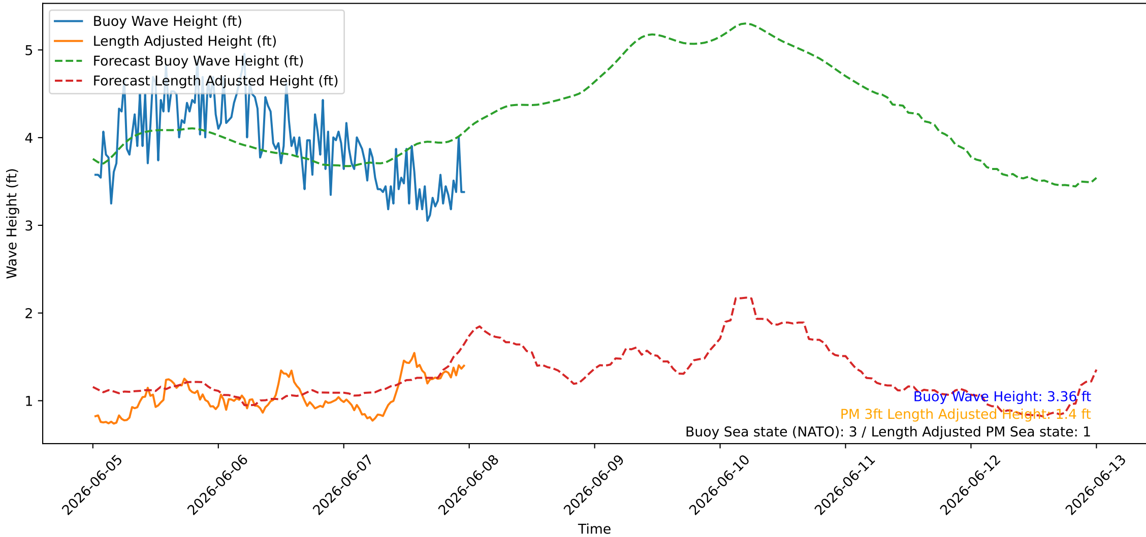
Wave Heights over Time for Red Beach at 2026-06-08 00:00:45
