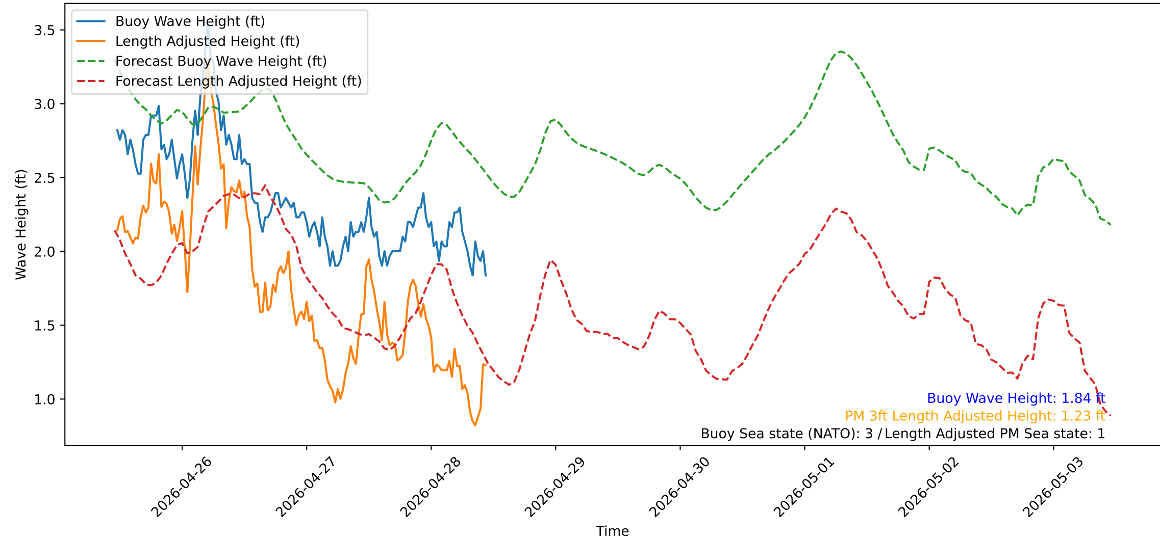
Wave Heights over Time for Red Beach at 2026-04-28 11:10:50
