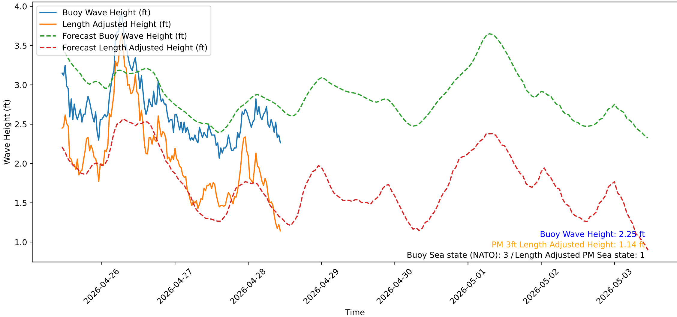
Wave Heights over Time for Oceanside Harbor at 2026-04-28 11:10:31
