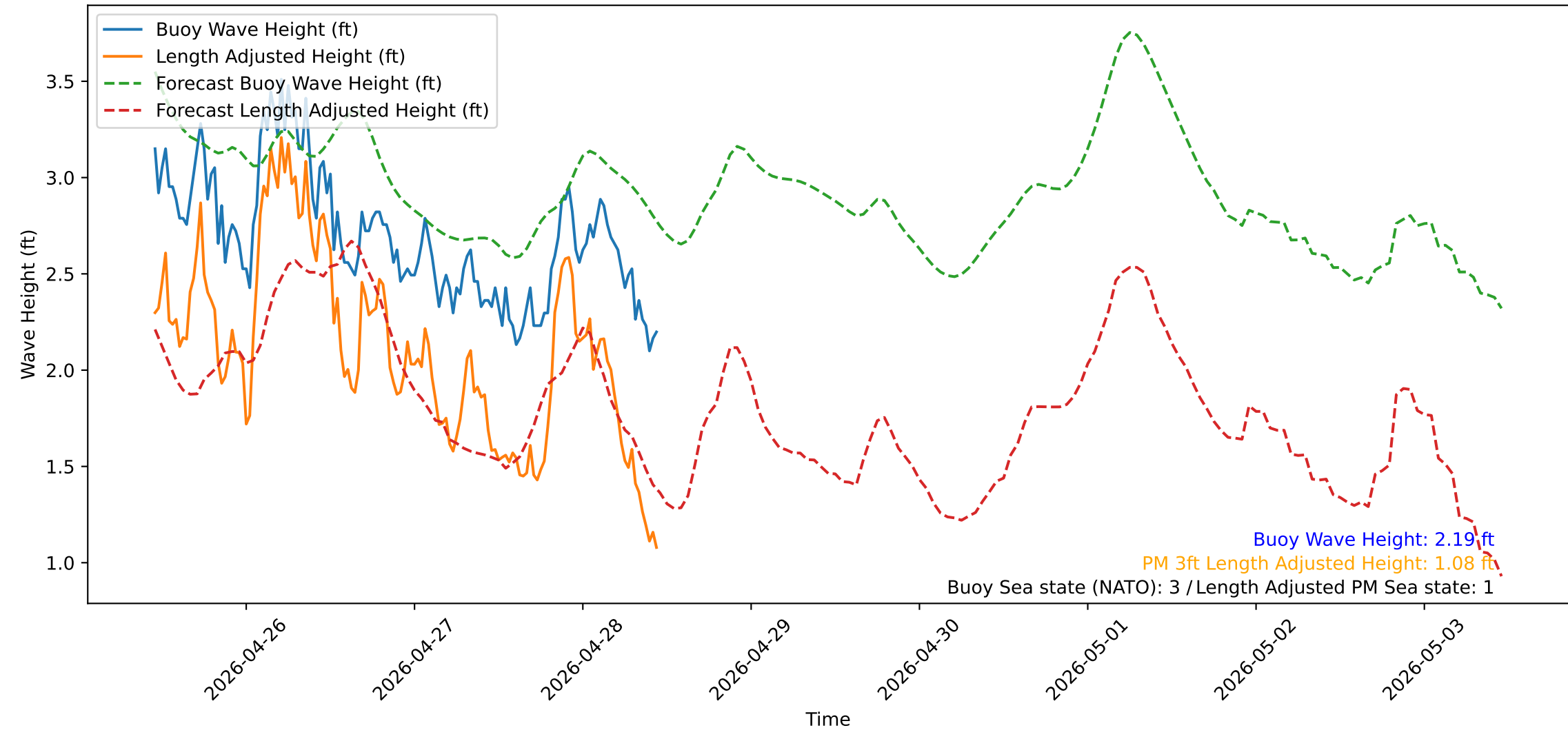
Wave Heights over Time for Green Beach at 2026-04-28 11:11:12
