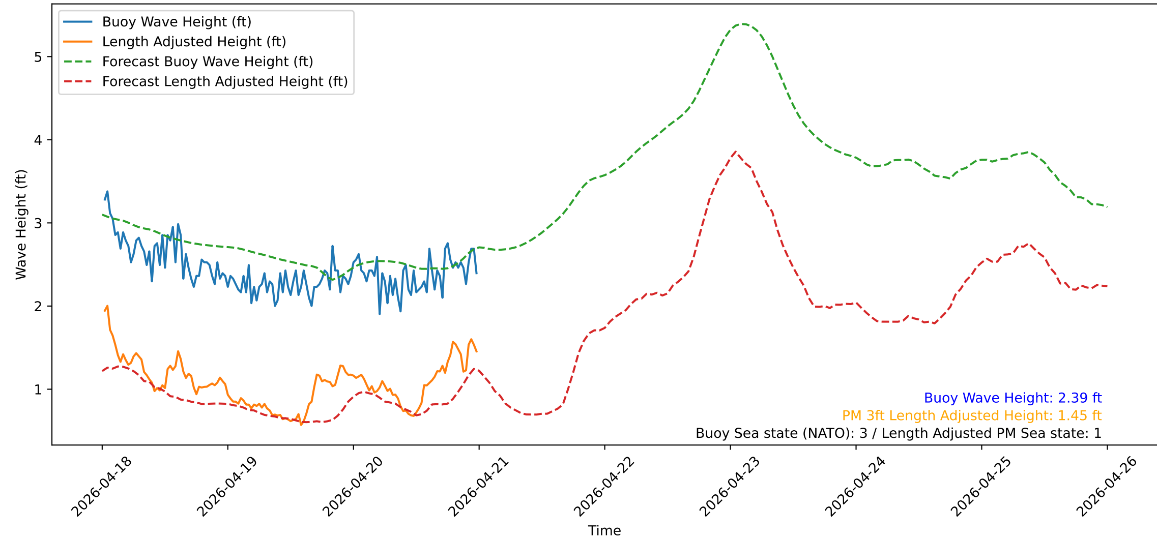
Wave Heights over Time for Oceanside Harbor at 2026-04-21 00:20:31
