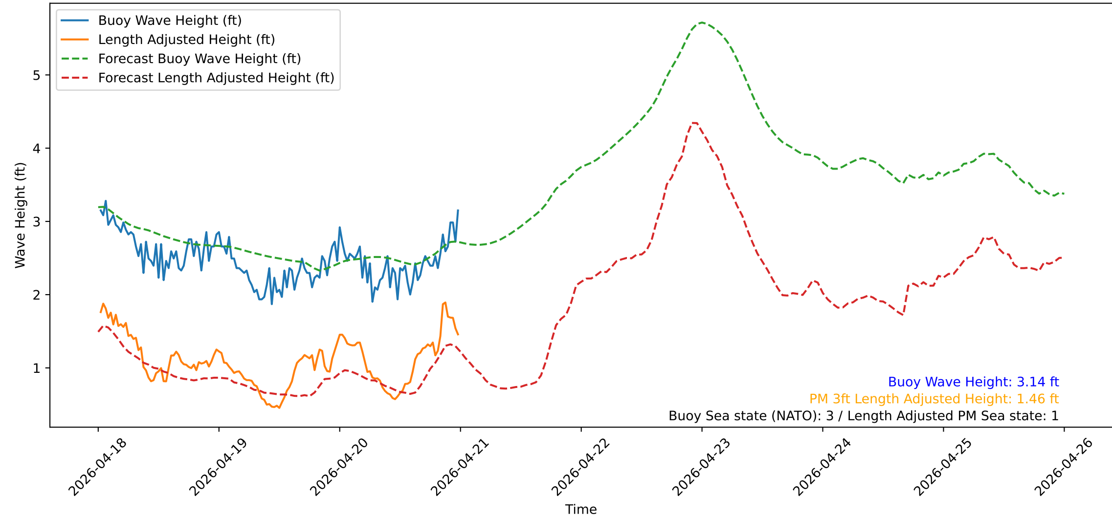
Wave Heights over Time for Green Beach at 2026-04-21 00:21:14
