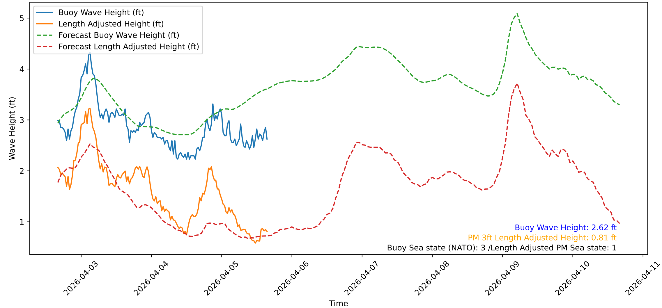
Wave Heights over Time for Green Beach at 2026-04-05 16:11:15
