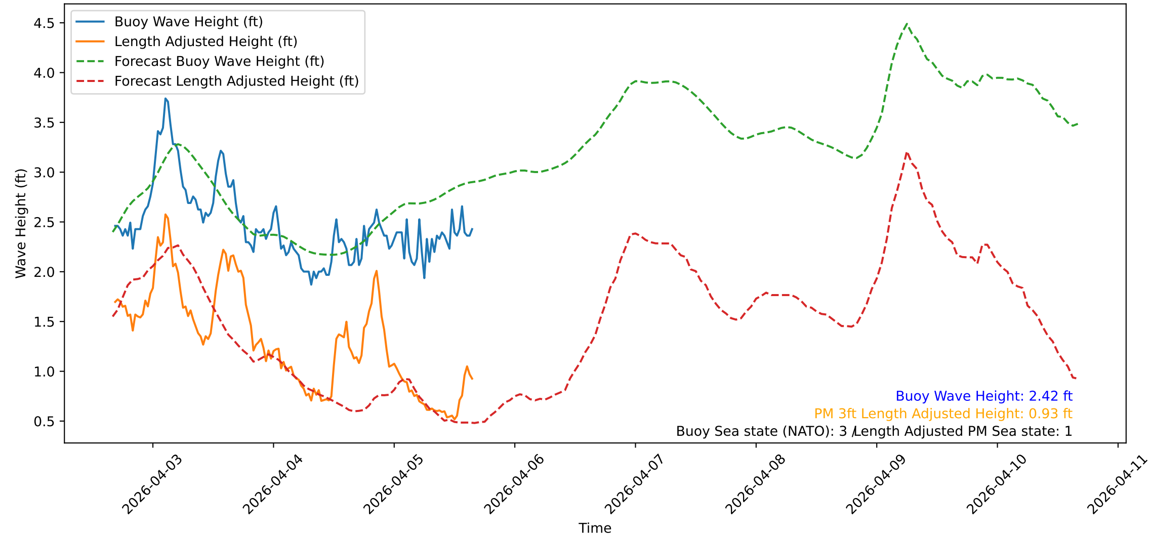
Wave Heights over Time for Red Beach at 2026-04-05 16:10:50
