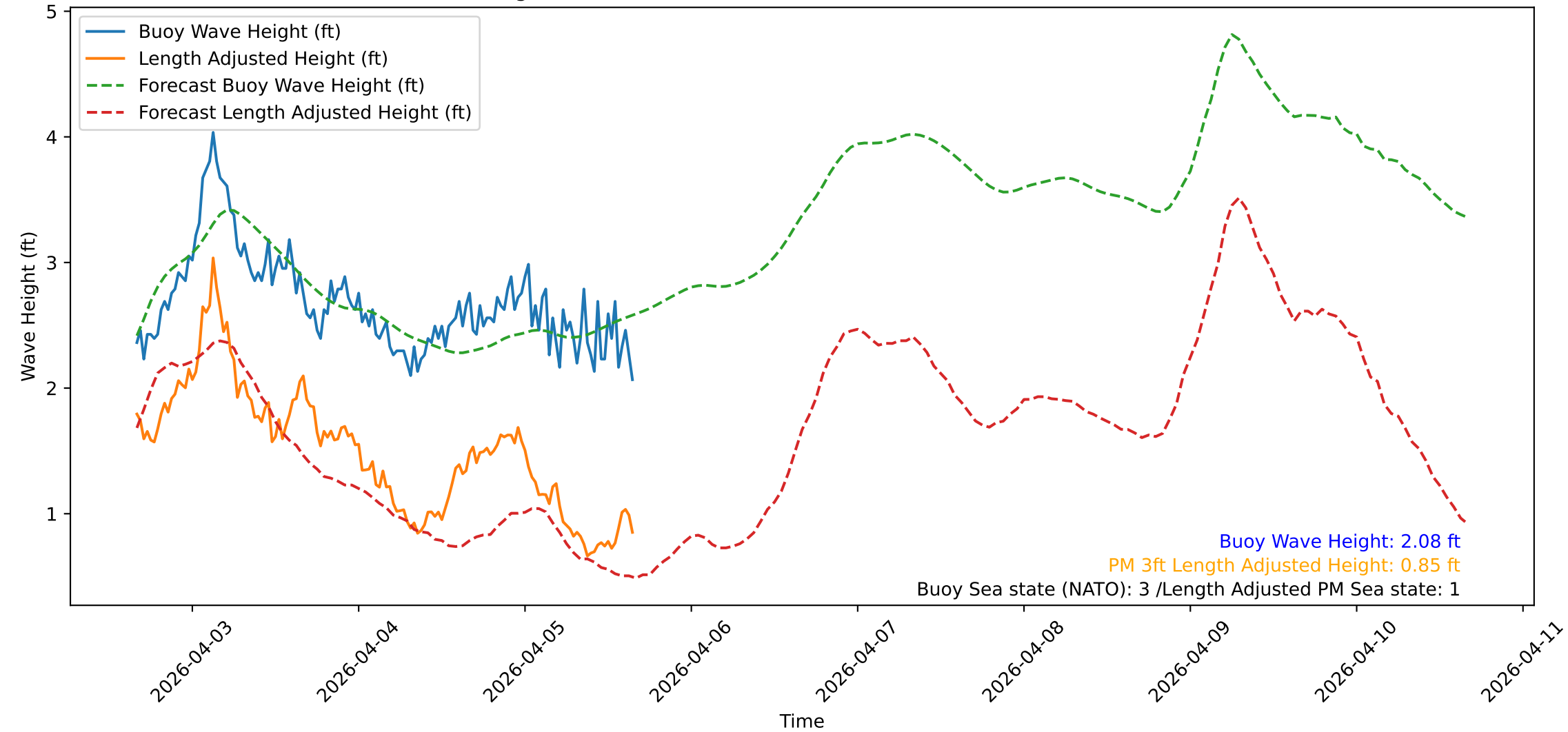
Wave Heights over Time for Oceanside Harbor at 2026-04-05 16:10:33
