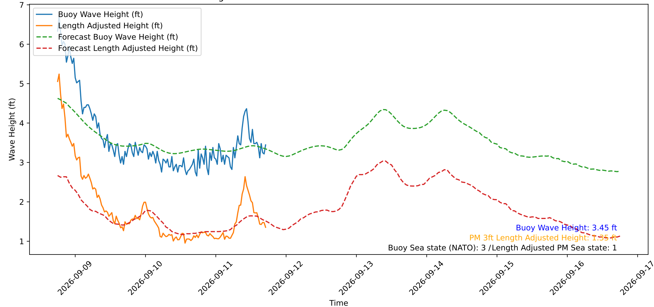
Wave Heights over Time for Oceanside Harbor at 2026-09-11 17:50:30
