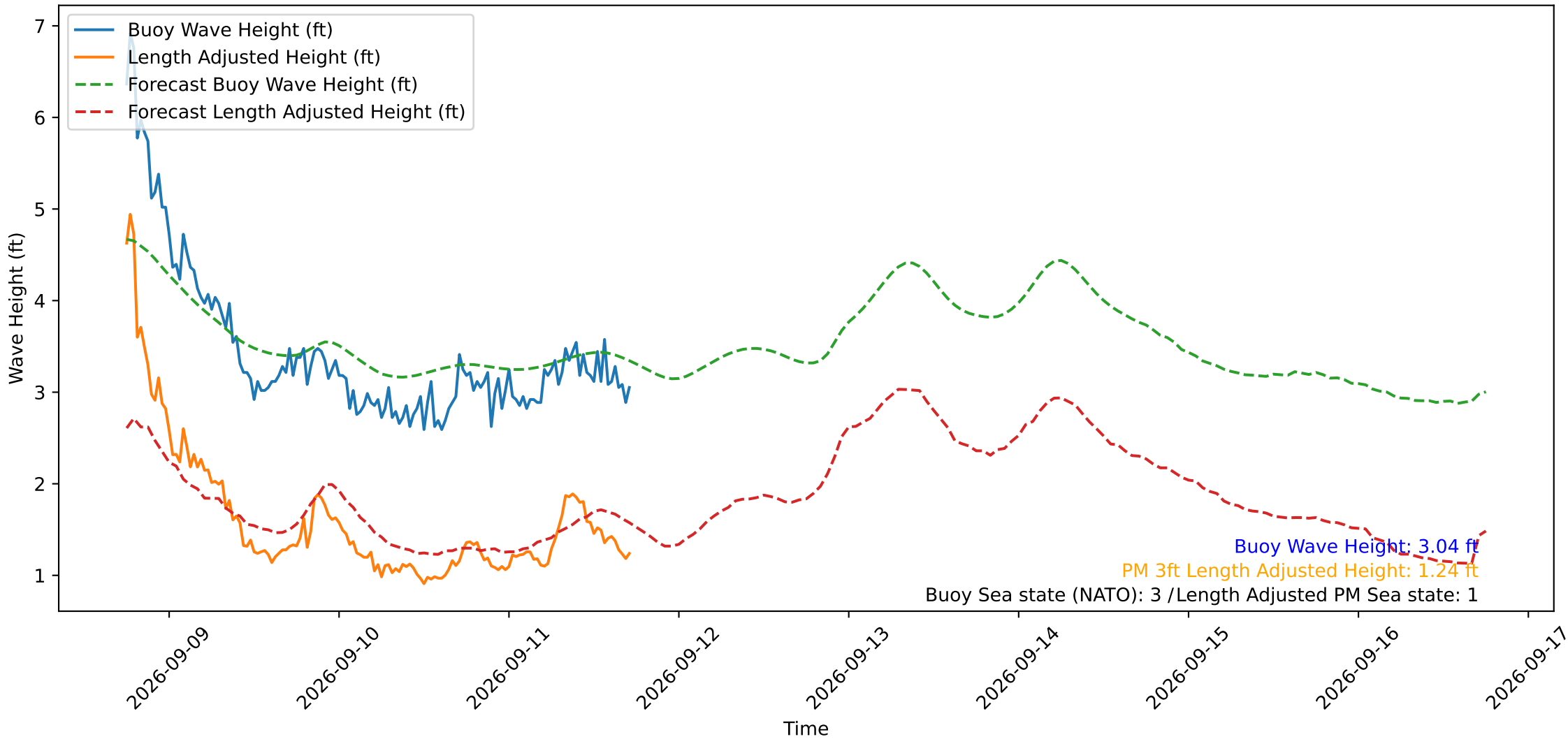
Wave Heights over Time for Green Beach at 2026-09-11 17:51:15
