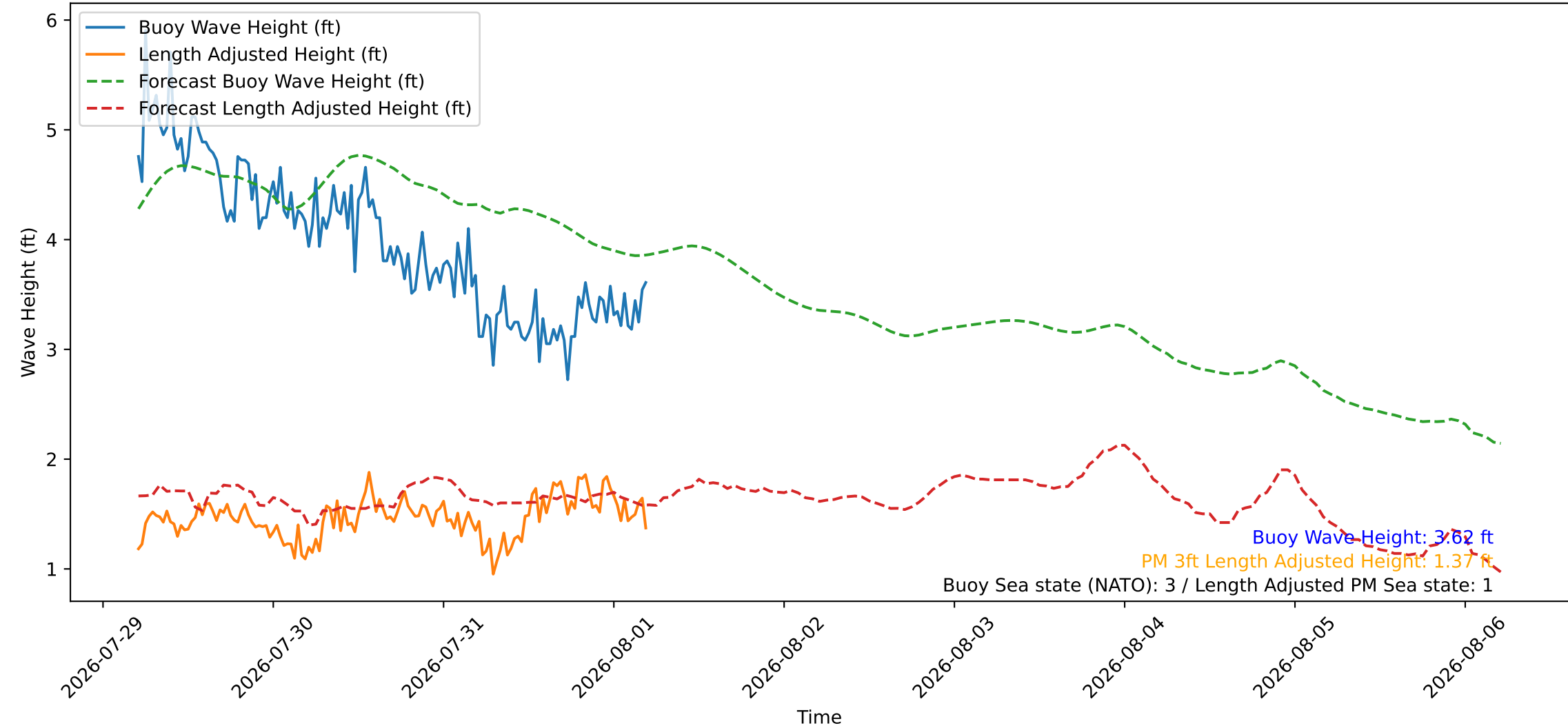
Wave Heights over Time for Oceanside Harbor at 2026-08-01 05:00:26
