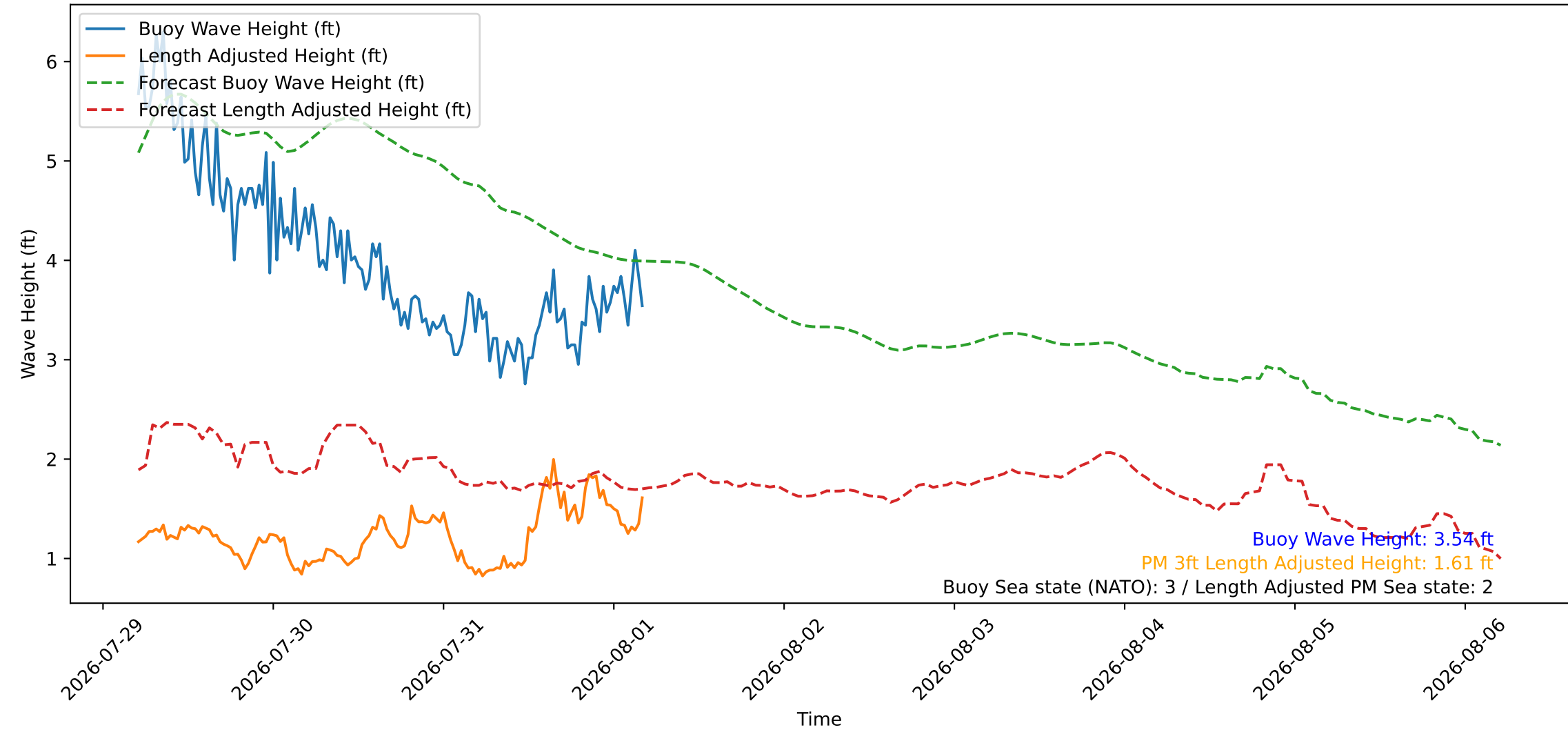
Wave Heights over Time for Green Beach at 2026-08-01 05:01:08
