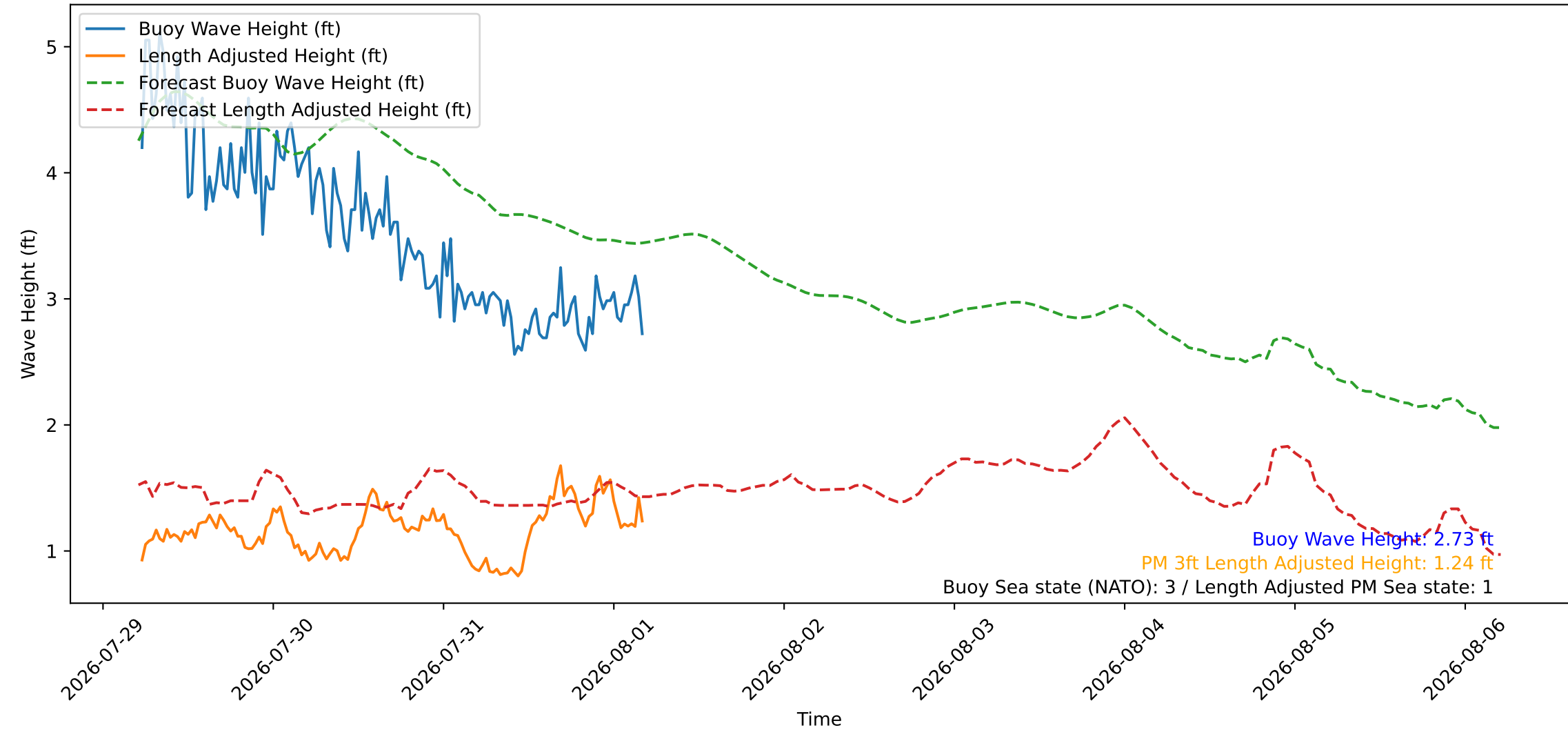
Wave Heights over Time for Red Beach at 2026-08-01 05:00:46
