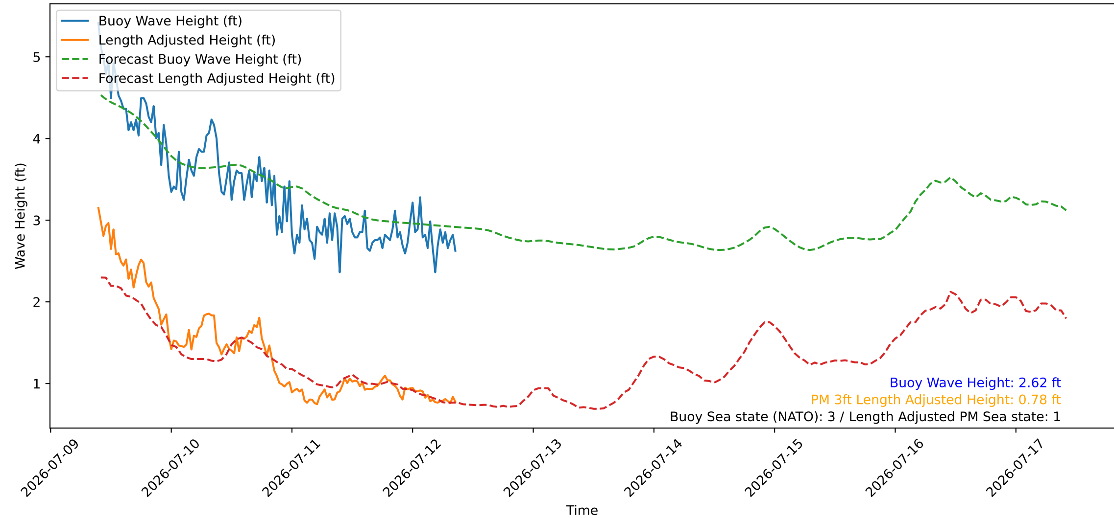
Wave Heights over Time for Oceanside Harbor at 2026-07-12 09:30:26
