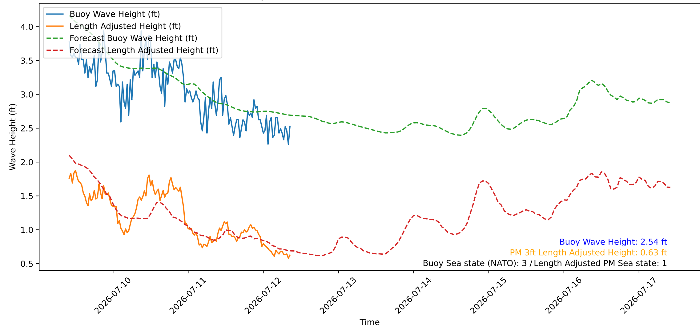
Wave Heights over Time for Red Beach at 2026-07-12 09:30:45
