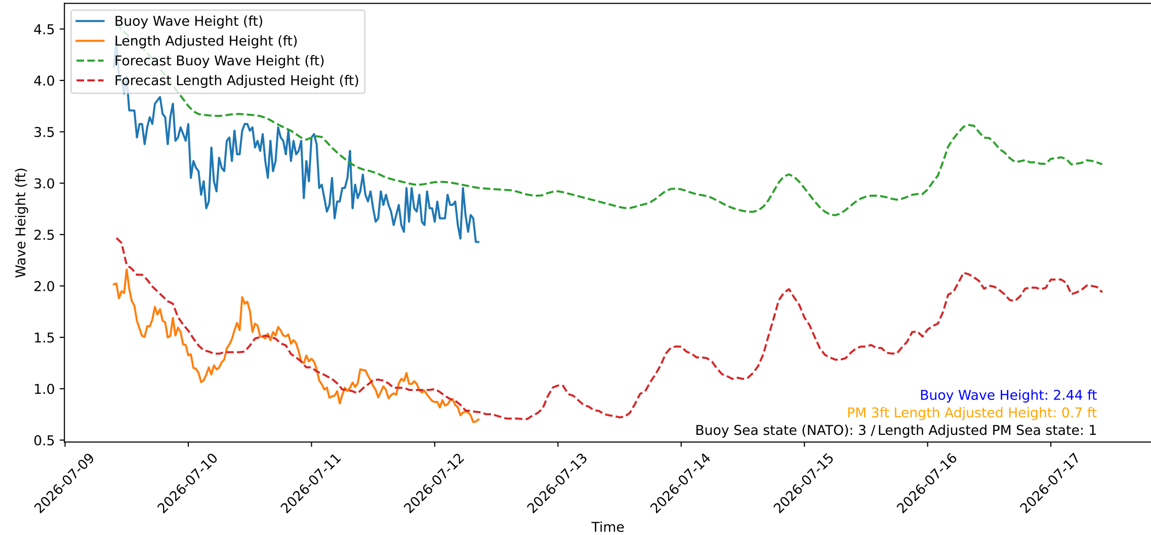
Wave Heights over Time for Green Beach at 2026-07-12 09:31:07
